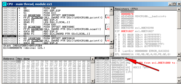
Figure 7.4: OllyDbg: preparing the value for printf()
