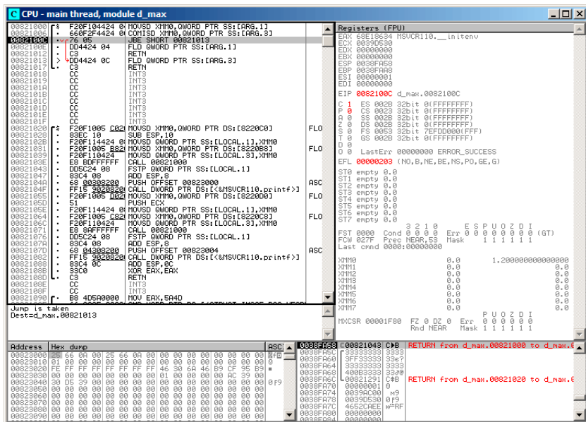
Figure 27.6: OllyDbg: COMISD changed CF and PF flags
