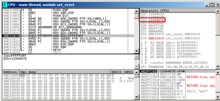
Figure 19.3: OllyDbg: value was reloaded into EDX
