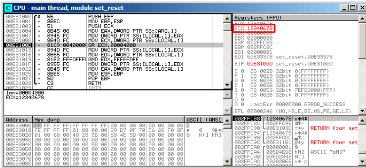
Figure 19.1: OllyDbg: value is loaded into ECX
