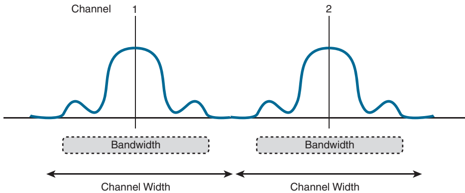
Figure 17-9 Non-overlapping Channel Spacing
