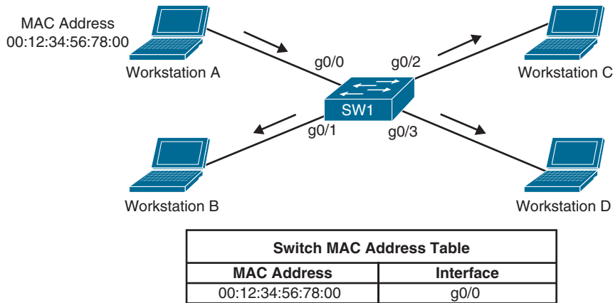
Figure 13-8 Unknown Frame Flooding
