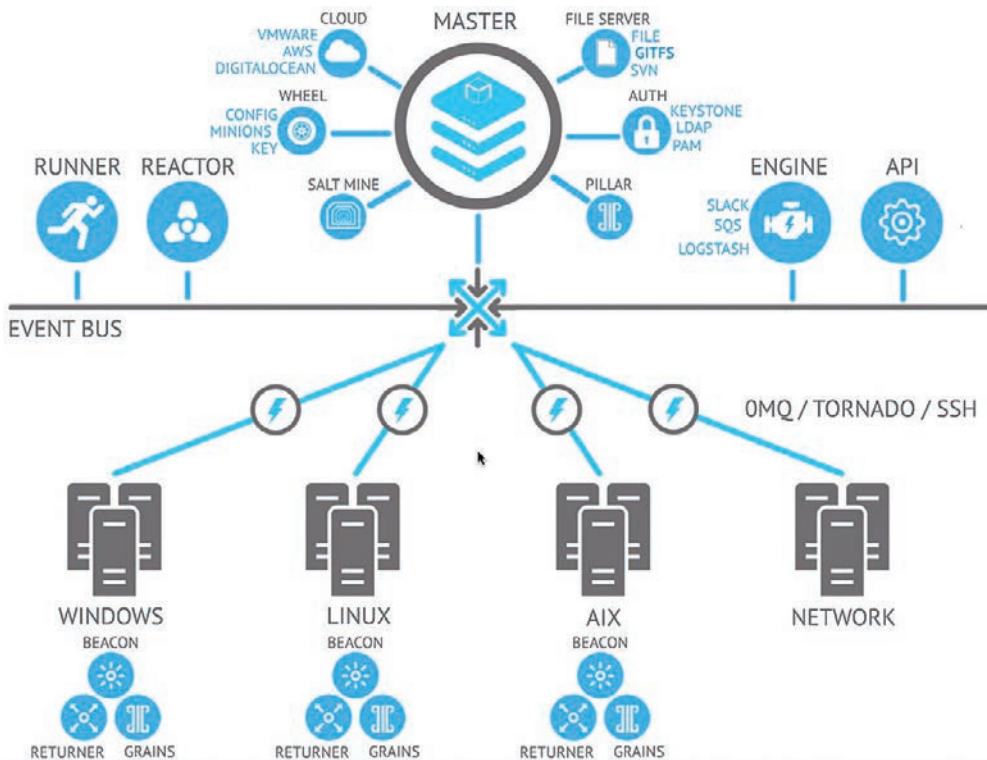
Figure 29-5 High-Level SaltStack Architecture
