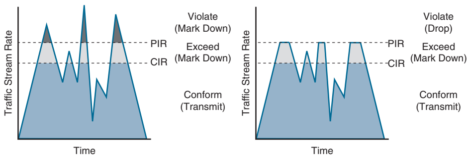
Figure 14-17 Two-Rate Three-Color Marker/Policer Token Bucket Algorithm
