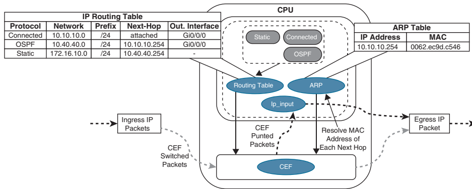
Figure 1-6 Process Switching
