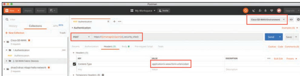
Figure 28-11 Cisco vManage Authentication API Setup for Postman
