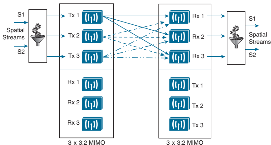
Figure 17-29 Spatial Multiplexing Between Two 3x3:2 MIMO Devices
