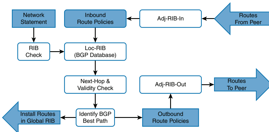
Figure 11-9 BGP Decision Process
