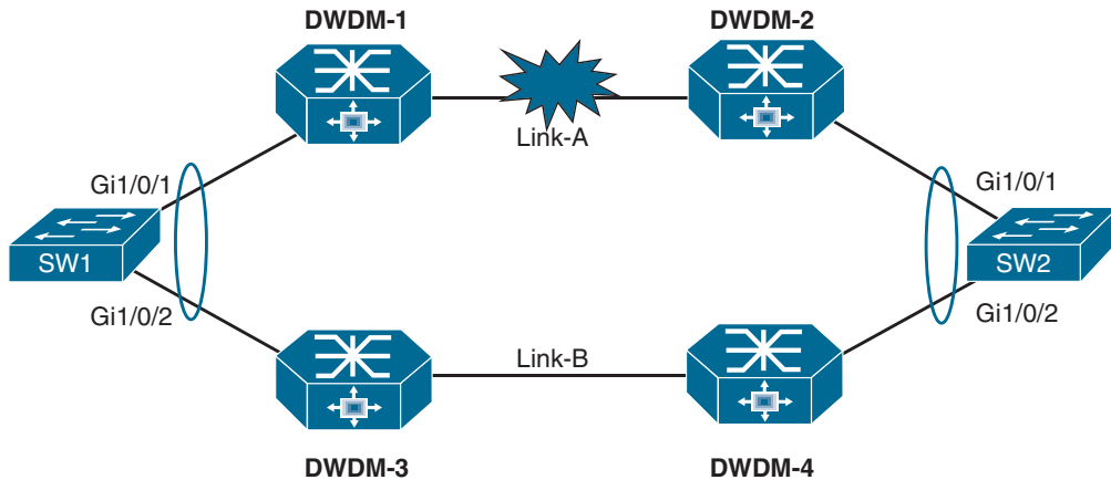
Figure 5-4 EtherChannel Link-State Propagation and Detection
