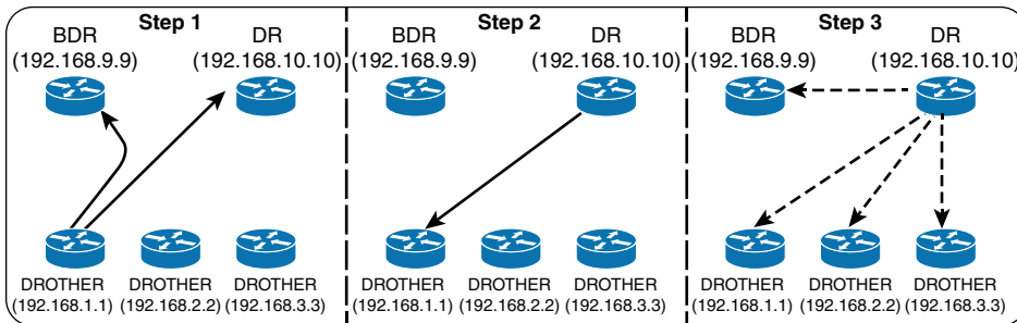
Figure 8-6 LSA Flooding with DR Segments
