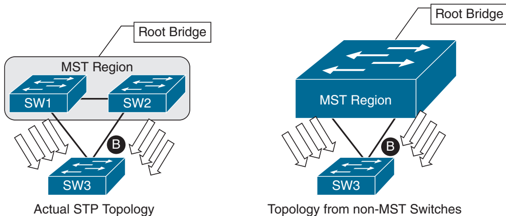
Figure 4-7 MST Region as the Root
