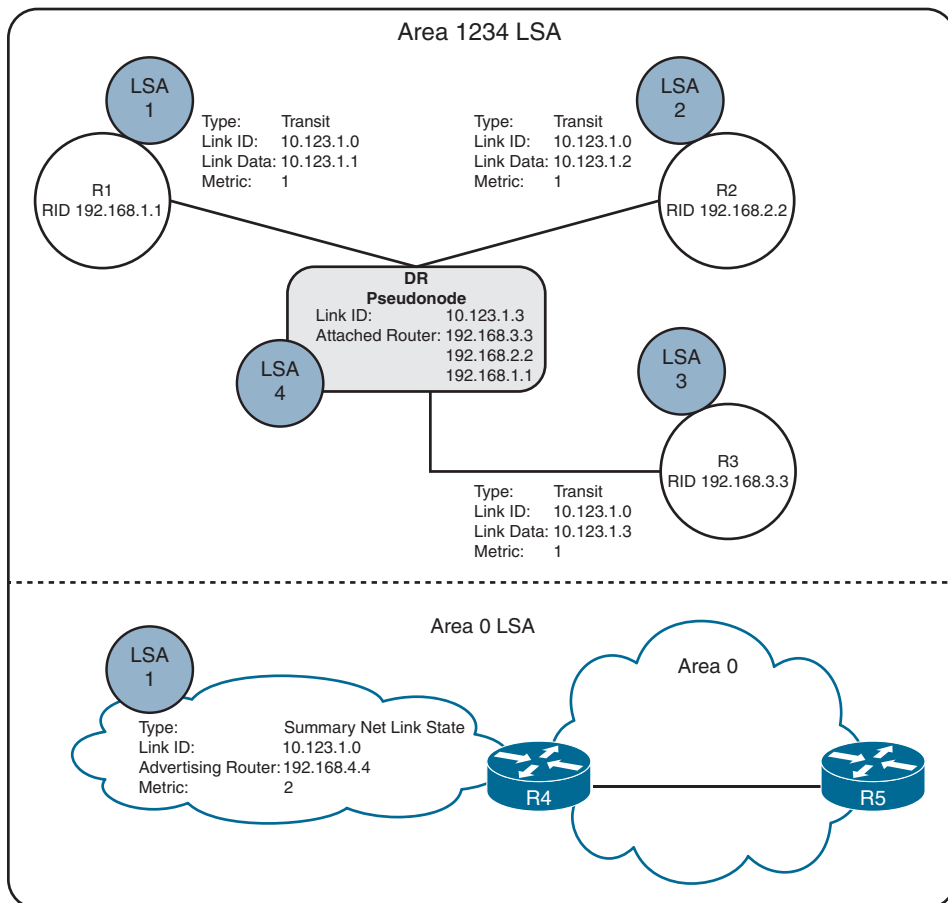
Figure 9-16 LSA Reduction Through Area Segmentation
