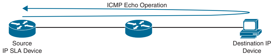
Figure 24-6 IP SLA Echo Operation
