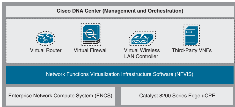
Figure 27-14 Enterprise NFV Solution Main Components
