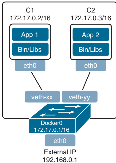
Figure 27-6 Container Bridging
