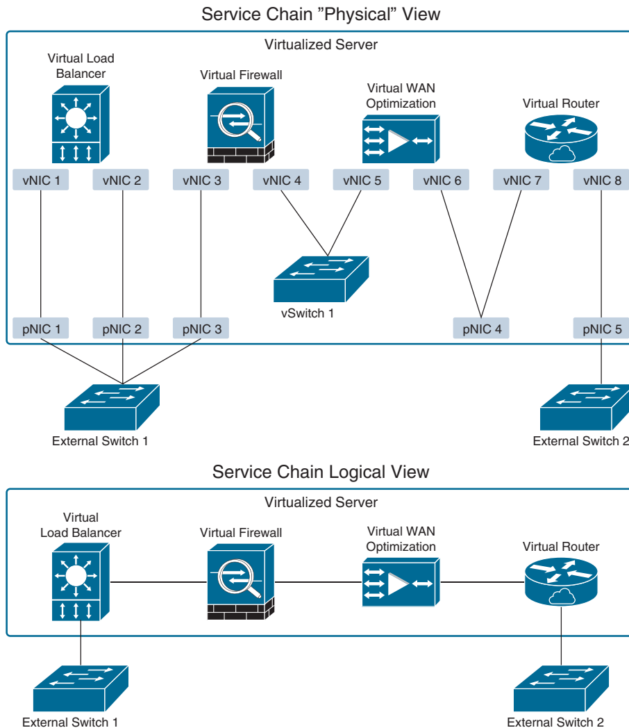
Figure 27-8 Service Chaining
