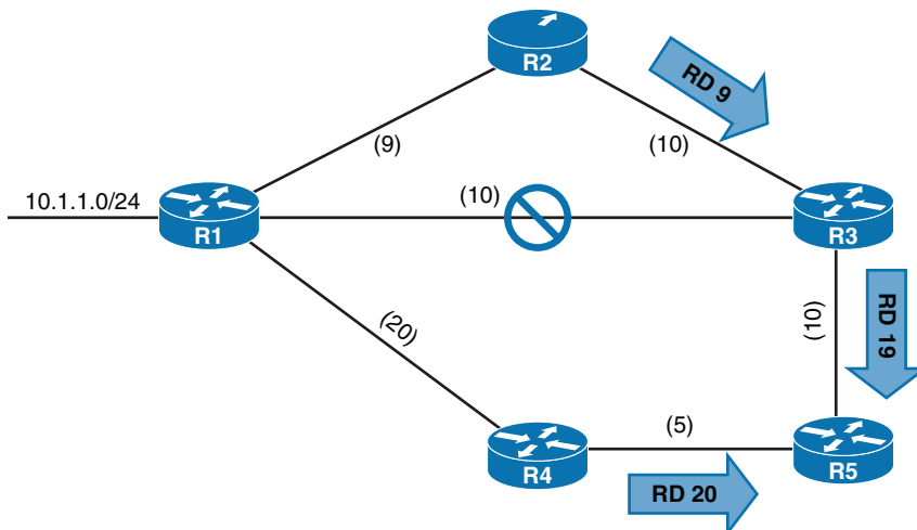
Figure 7-11 EIGRP Topology with Link Failure
