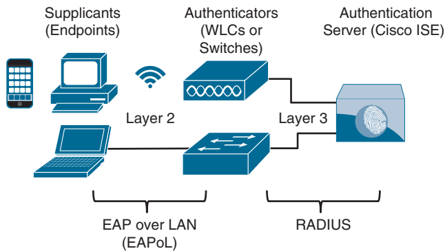
Figure 25-5 802.1x Roles and Components
