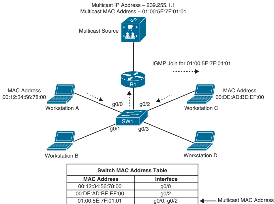
Figure 13-10 IGMP Snooping Example
