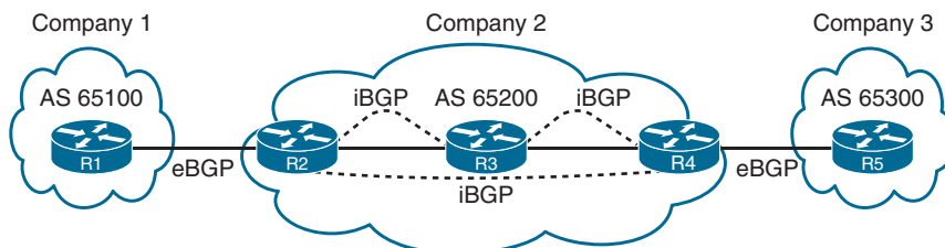
Figure 11-5 eBGP and iBGP Sessions
