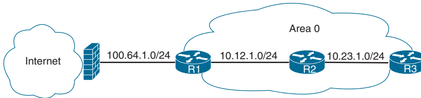
Figure 8-8 Default Route Topology
