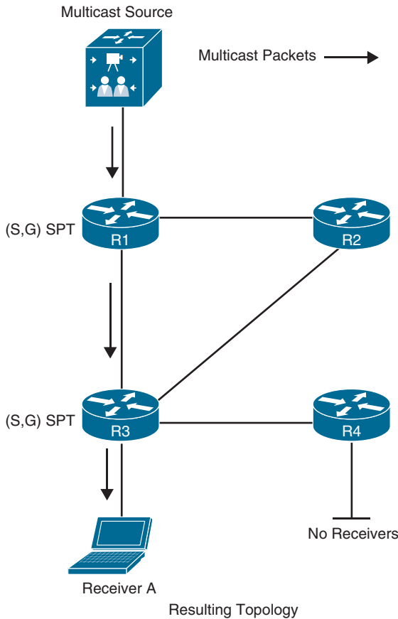
Figure 13-16 PIM-DM Resulting Topology After Pruning
