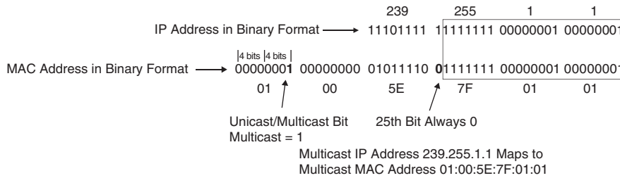
Figure 13-5 Multicast IP Address to Multicast MAC Address Mapping
