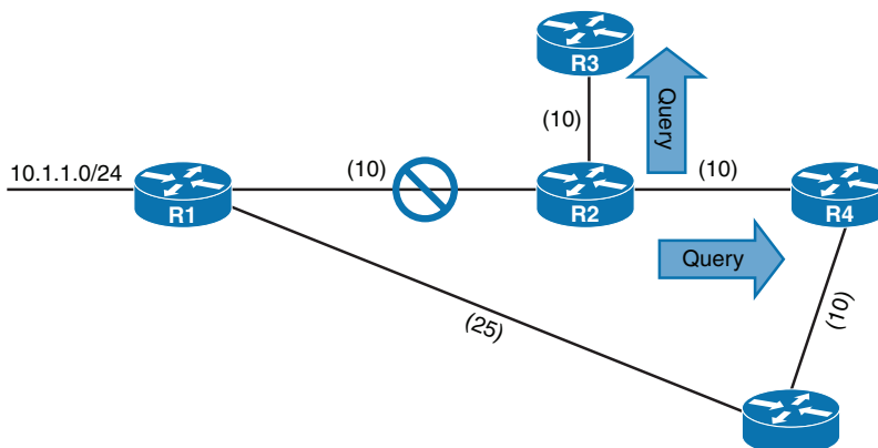
Figure 7-12 Generation of Query Packets on R2
