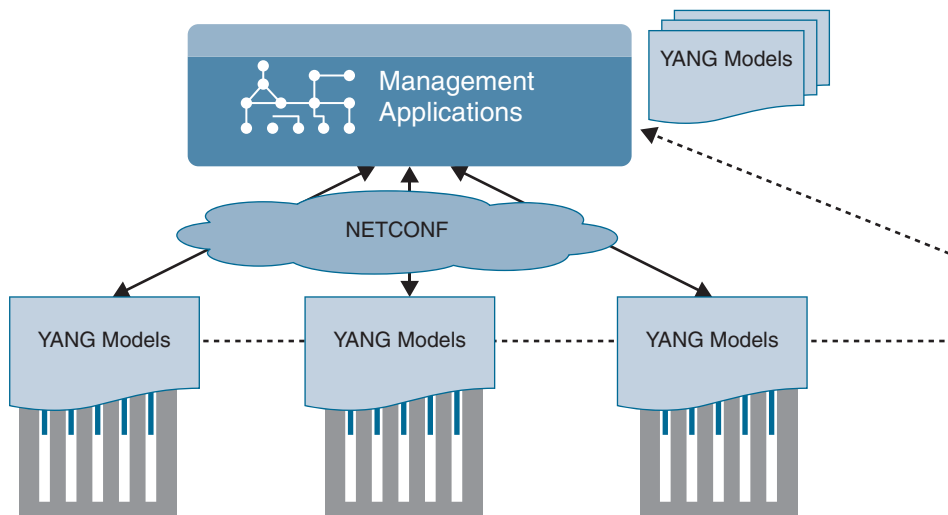
Figure 28-15 NETCONF/YANG Interfacing with Management Applications
