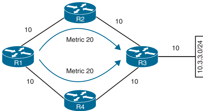
Figure 6-6 OSPF ECMP Technology
