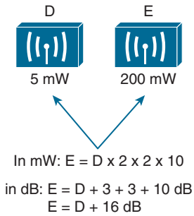
Figure 17-17 Example of Computing dB with Simple Rules
