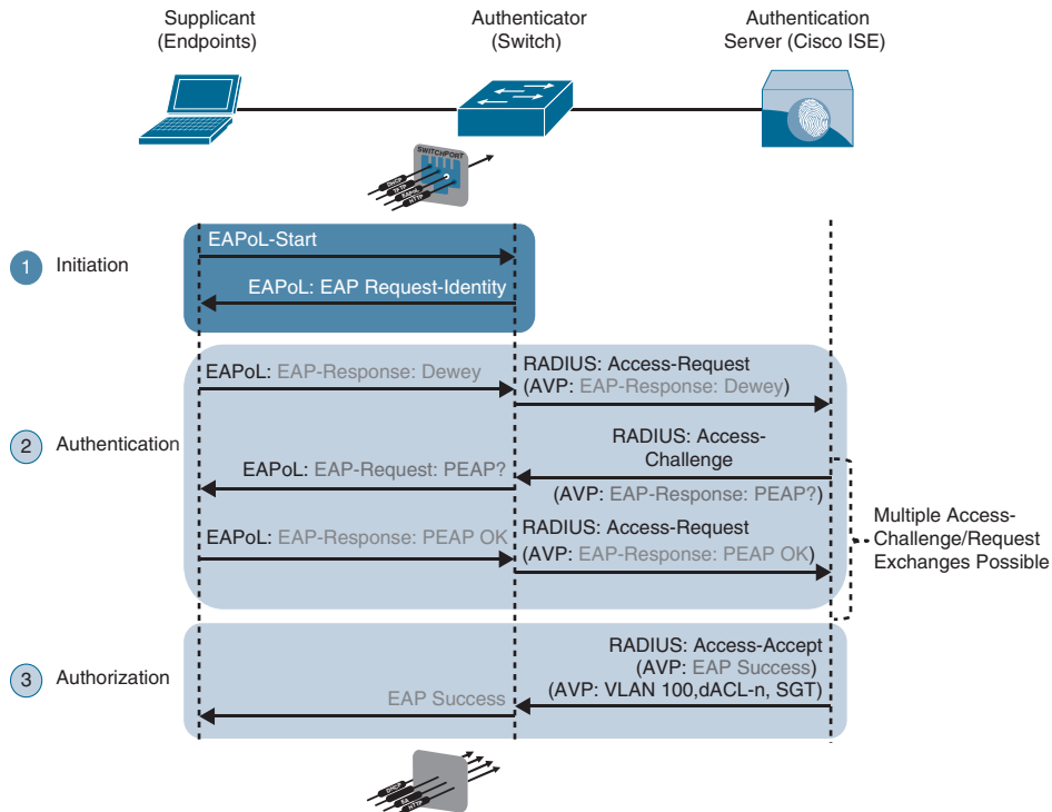
Figure 25-6 Successful 802.1x Authentication Process Flow
