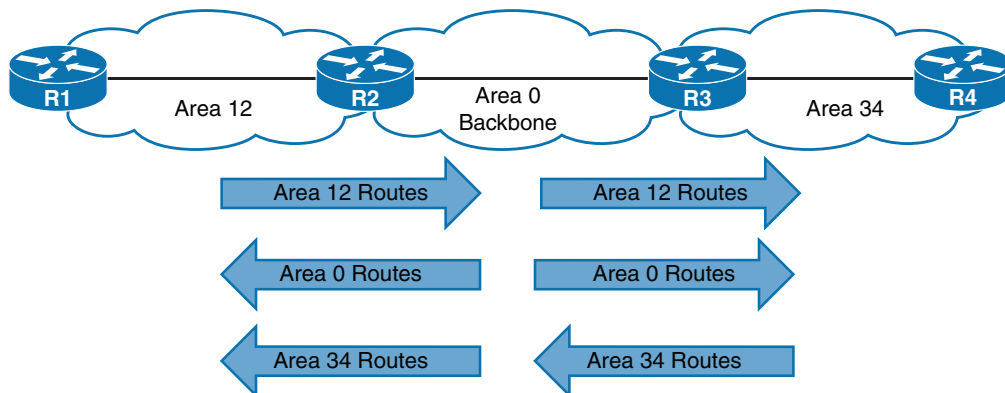
Figure 8-2 Two-Tier Hierarchical Area Structure
