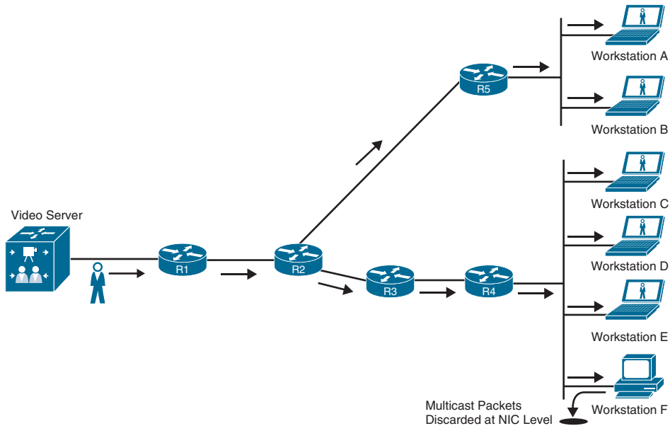
Figure 13-4 Multicast Video Feed
