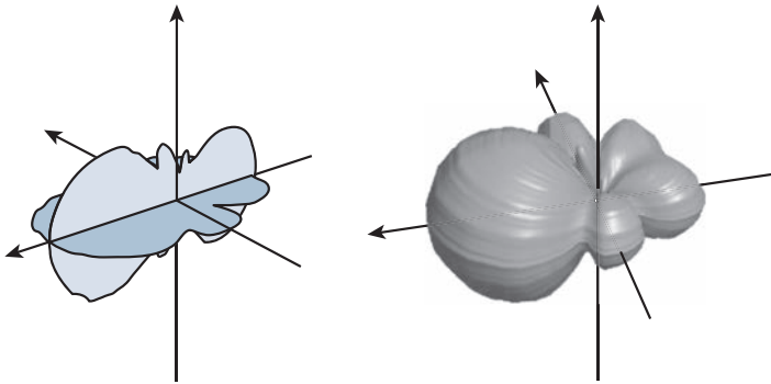
Figure 18-26 Yagi Antenna Radiation Pattern in Three Dimensions
