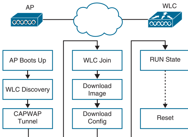
Figure 18-8 State Machine of a Lightweight AP
