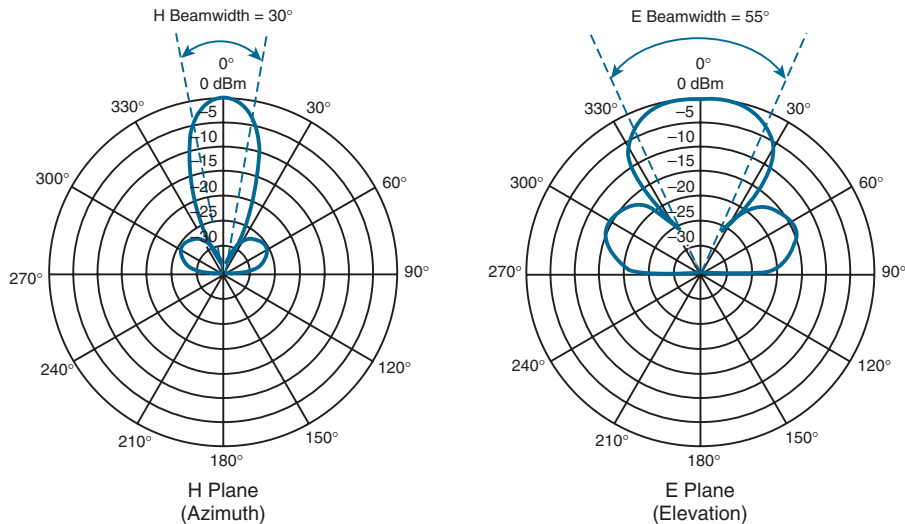
Figure 18-14 Example of Antenna Beamwidth Measurement
