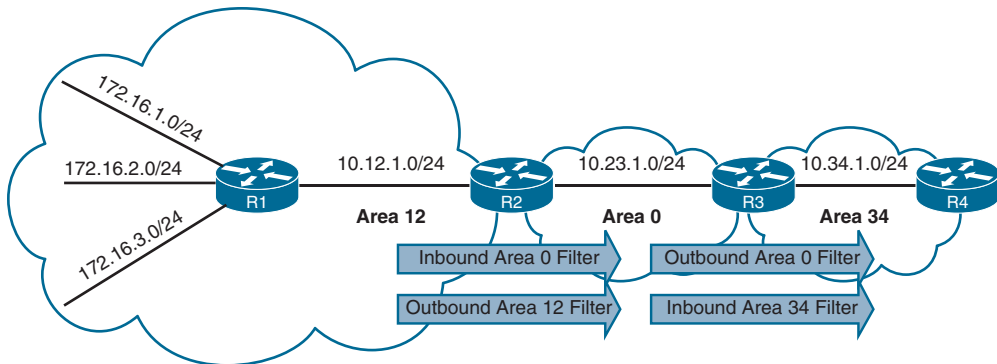
Figure 9-24 OSPF Area Filtering Topology
