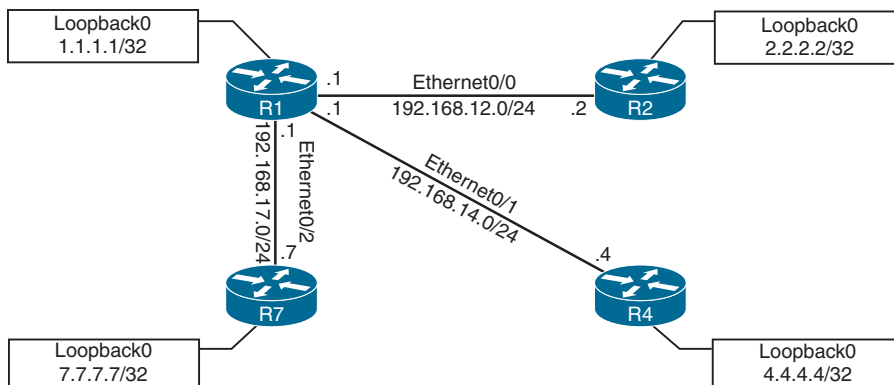
Figure 24-2 Debugging Topology
