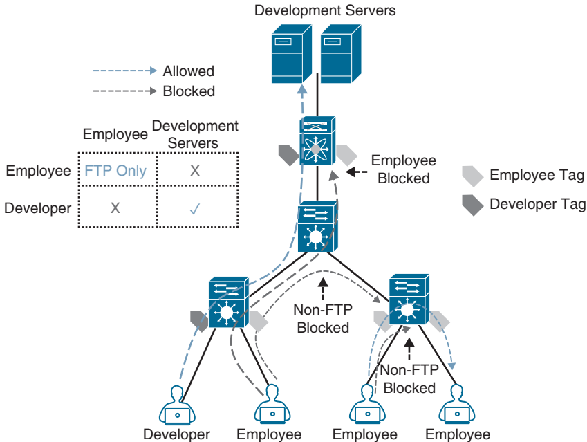
Figure 25-16 TrustSec Software-Defined Segmentation
