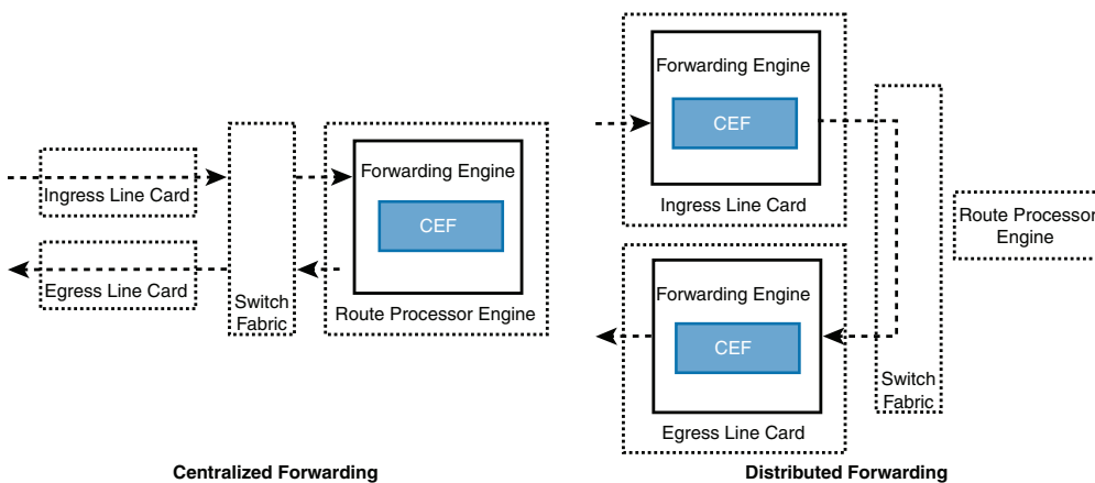
Figure 1-7 Centralized Versus Distributed Forwarding Architectures
