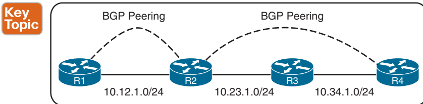
Figure 11-2 BGP Single- and Multi-Hop Sessions
