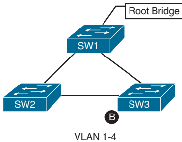
Figure 4-1 Common Spanning Tree Instance (CST) Topology
