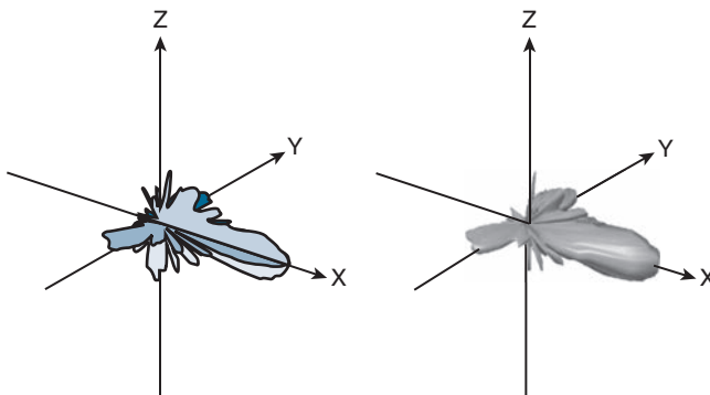
Figure 18-29 Parabolic Dish Antenna Radiation Pattern in Three Dimensions
