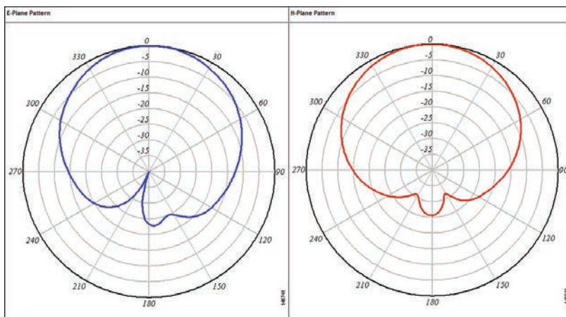
Figure 18-22 E and H Radiation Patterns for a Typical Patch Antenna
