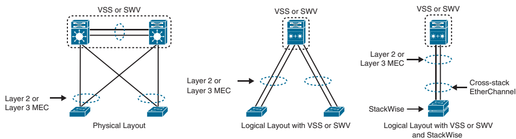
Figure 22-11 Simplified Campus Design with VSS, SWV, and StackWise
