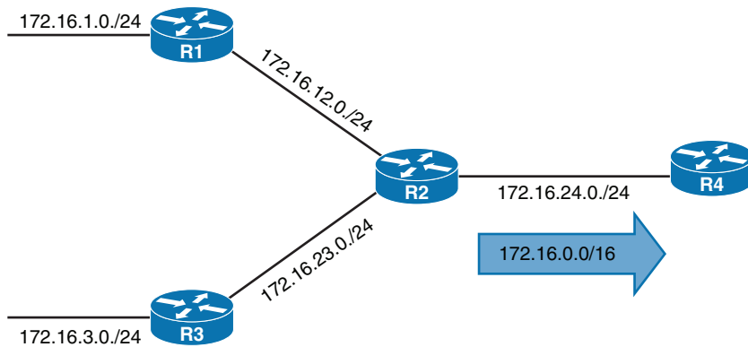
Figure 7-13 EIGRP Summarization
