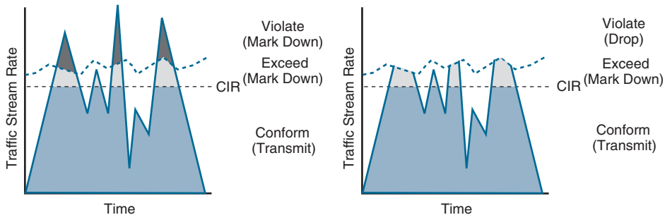
Figure 14-15 Single-Rate Three-Color Marker/Policer
