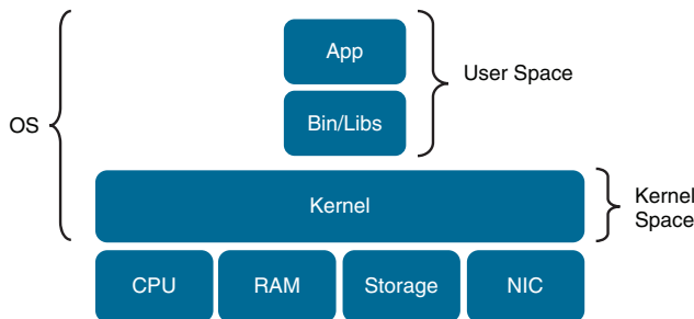
Figure 27-9 Operating System Kernel and User Space
