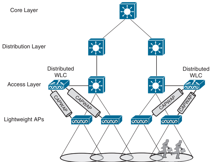
Figure 18-6 WLC Location in a Distributed Wireless Deployment
