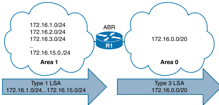
Figure 9-19 OSPF Inter-Area Summarization
