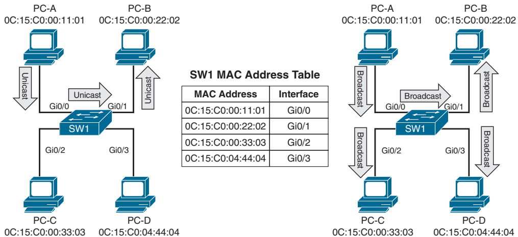
Figure 1-3 Unicast and Broadcast Traffic Patterns
