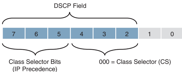
Figure 14-6 Class Selector (CS) PHB
