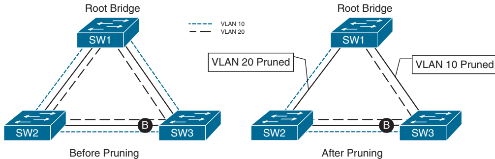
Figure 4-6 Trunk Link Pruning
