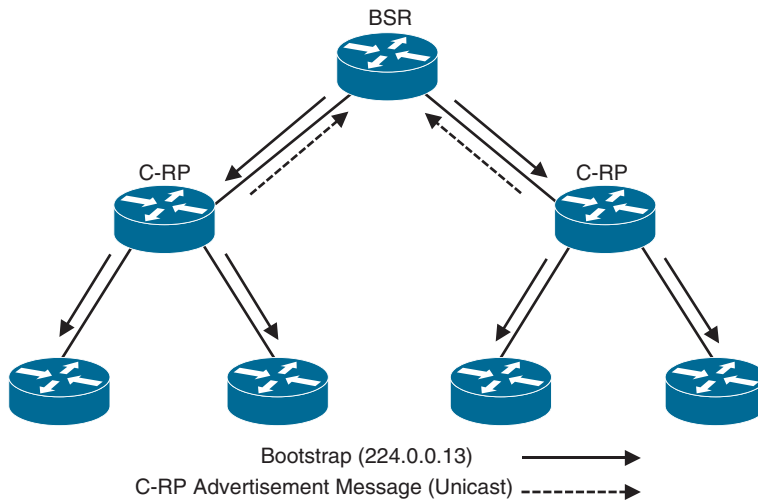
Figure 13-23 BSR Mechanism
