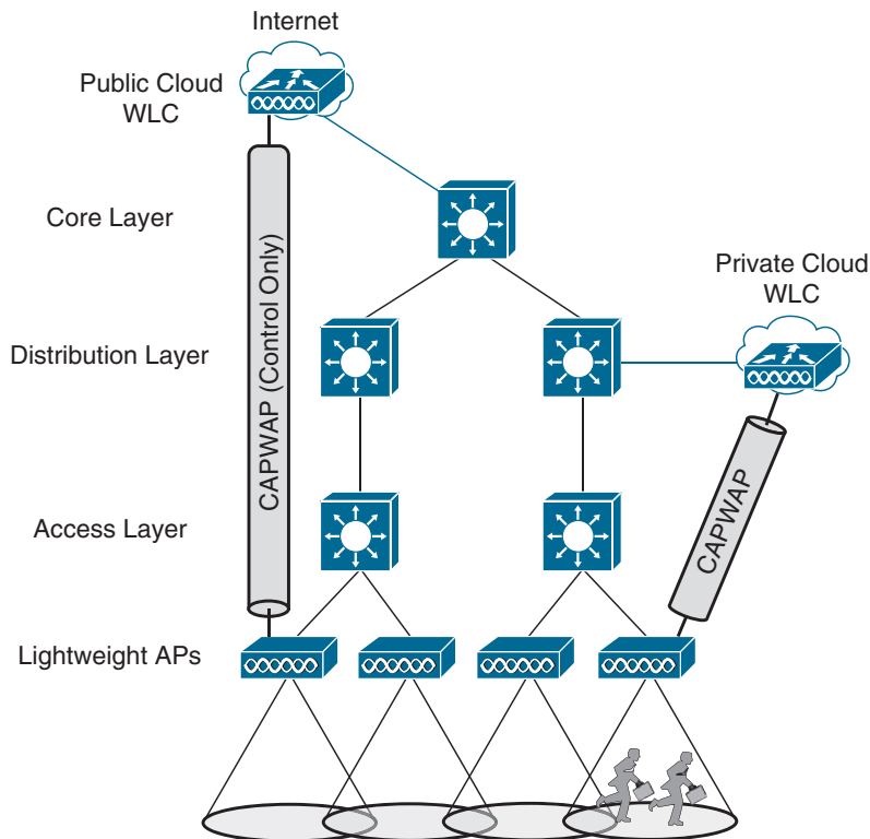
Figure 18-5 WLC Location in a Cloud-Based Wireless Deployment
