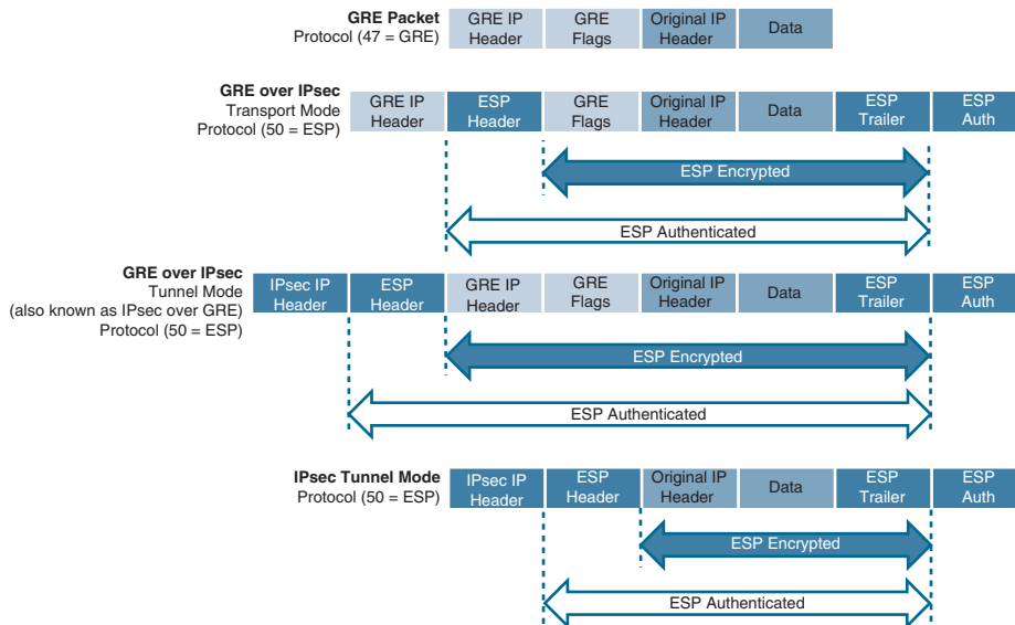
Figure 16-4 GRE over IPsec Versus IPsec Tunnel Mode
