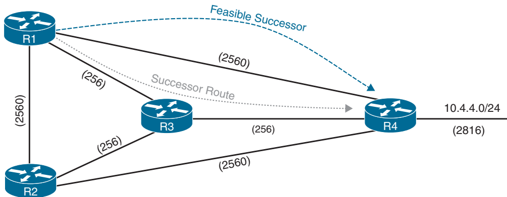
Figure 7-2 EIGRP Reference Topology
