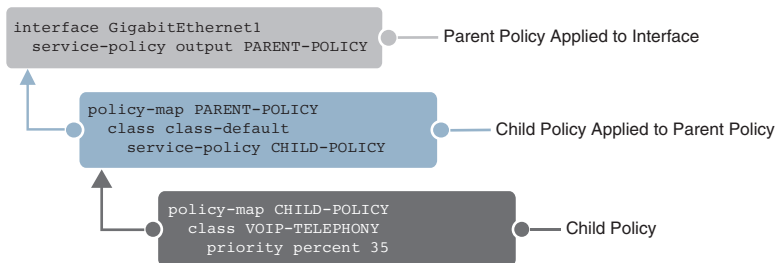
Figure 14-3 MQC Hierarchical QoS Policy Map Example
