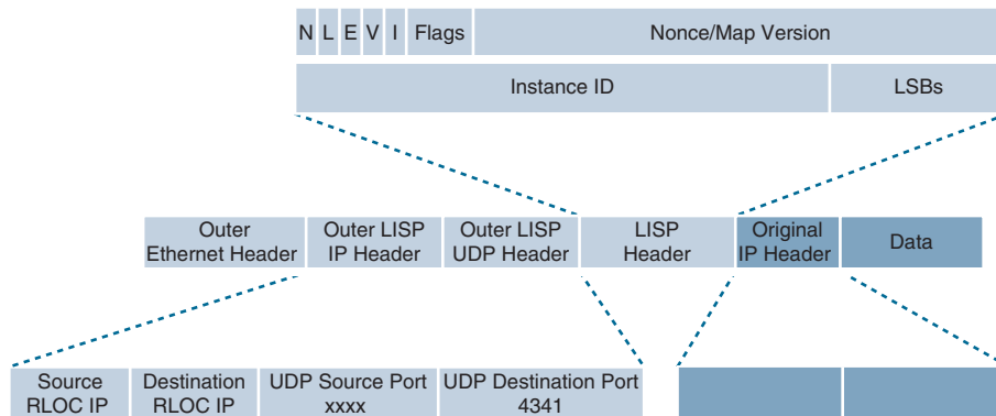
Figure 16-7 LISP Packet Format
