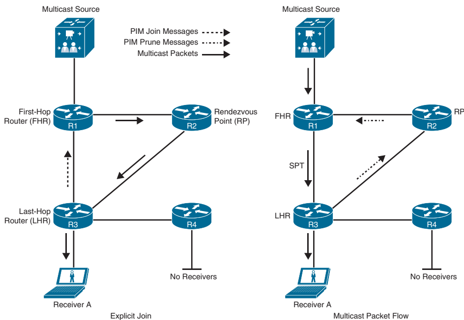
Figure 13-18 PIM-SM SPT Switchover Example
