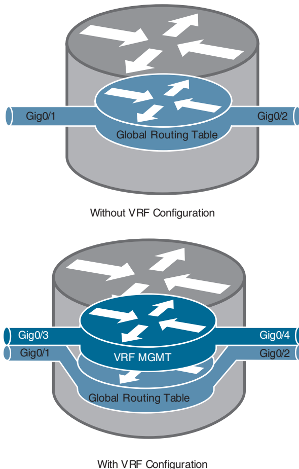
Figure 6-15 Comparison of a Router with No VRF Instances and a Router with a VRF Instance
