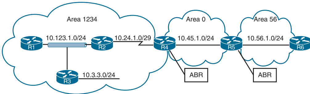
Figure 9-3 OSPF Multi-Area Topology
