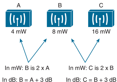
Figure 17-16 Comparing Power Levels Using dB
