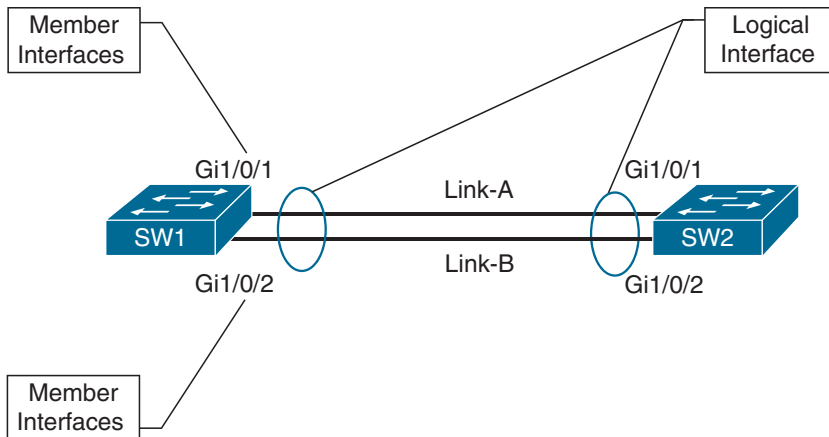
Figure 5-3 EtherChannel Components
