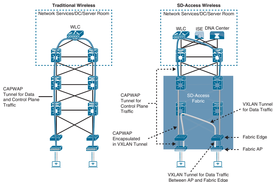
Figure 23-7 Traditional Wireless and SD-Access Wireless Deployments
