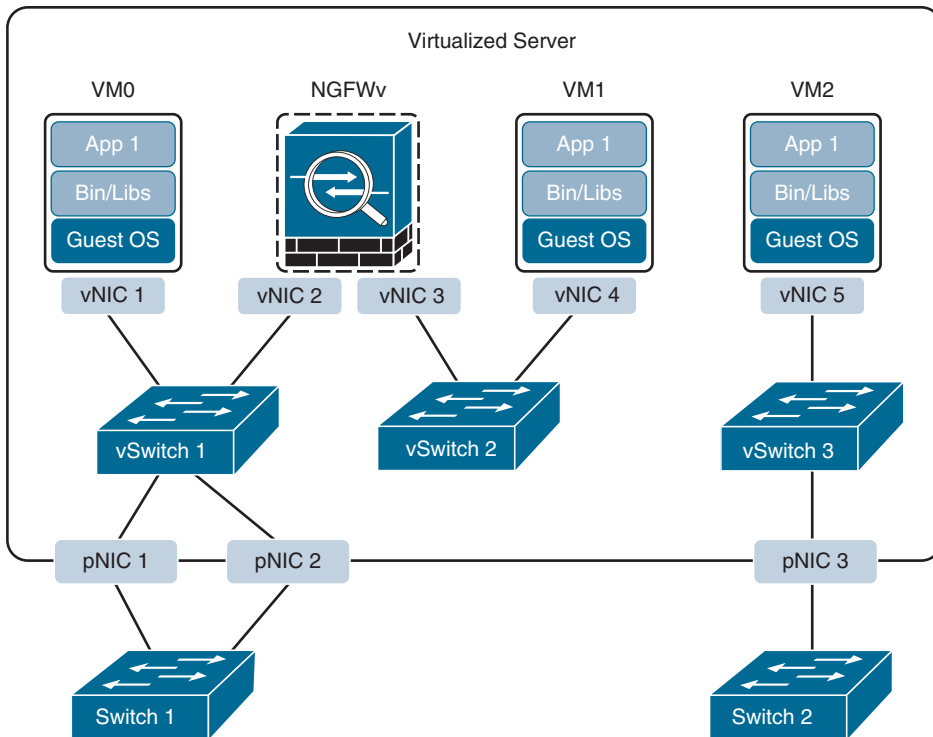
Figure 27-5 Virtualized Server with vSwitches
