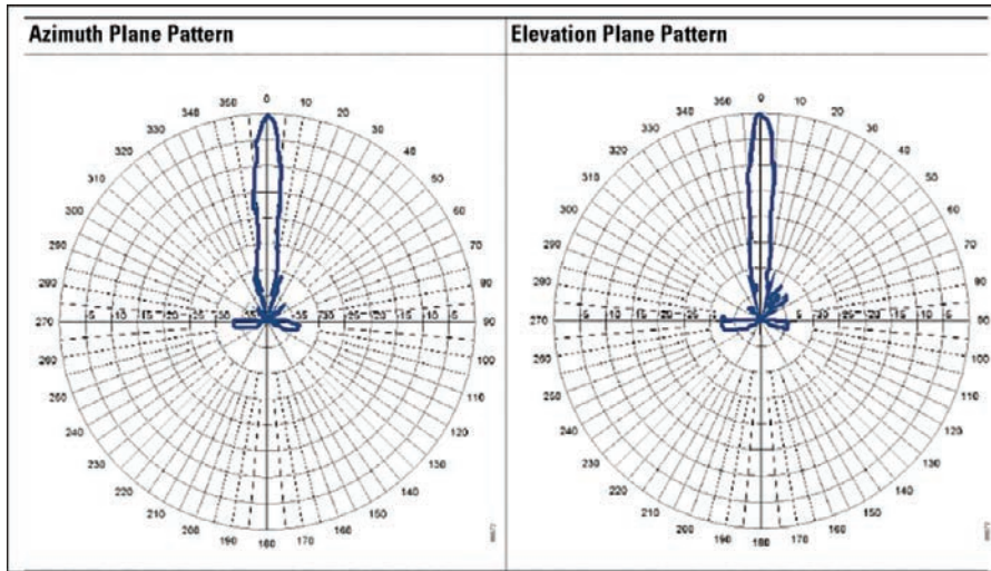
Figure 18-28 E and H Radiation Patterns for a Parabolic Dish Antenna
