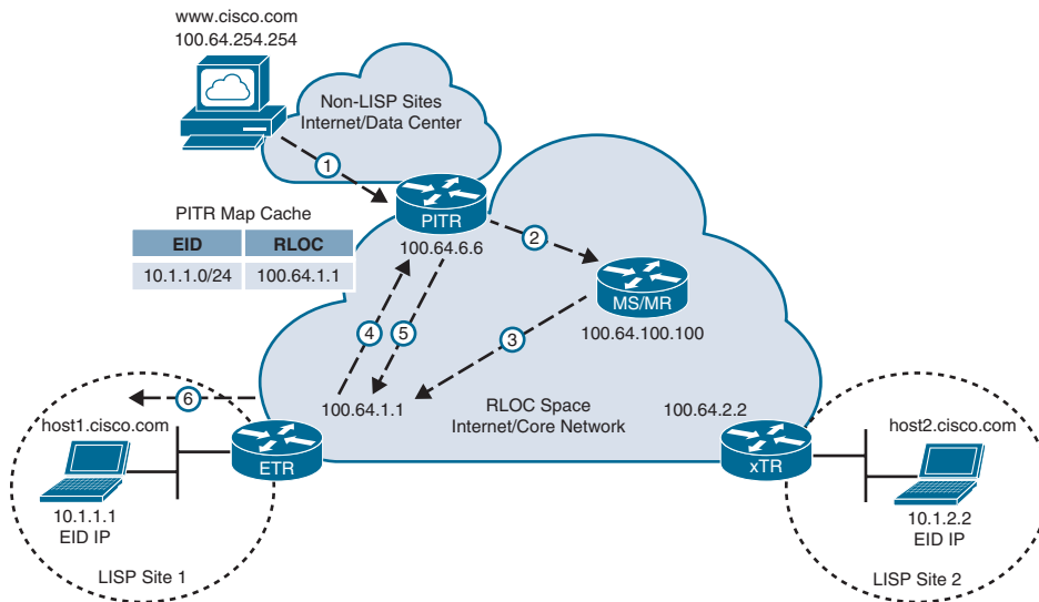
Figure 16-12 Proxy ITR Process
