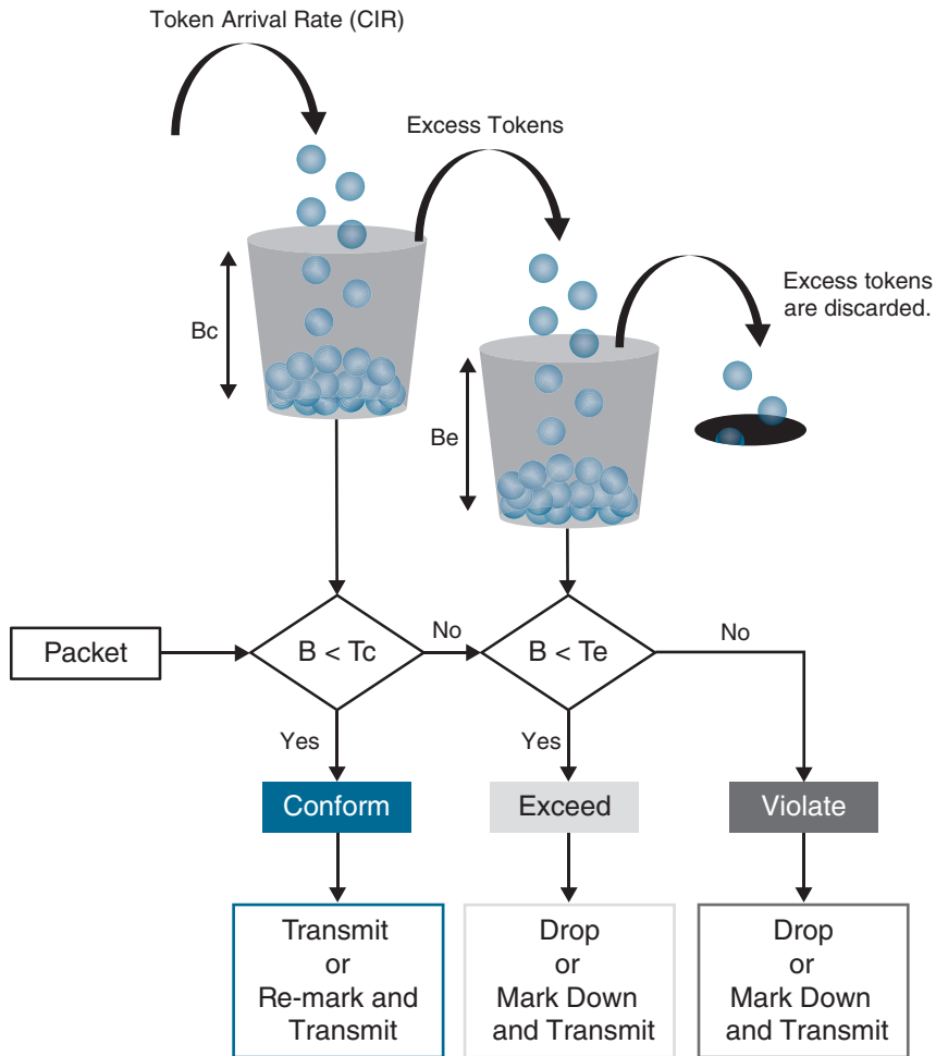
Figure 14-16 Single-Rate Three-Color Marker/Policer Token Bucket Algorithm
