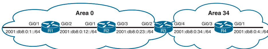
Figure 10-1 OSPFv3 Topology
