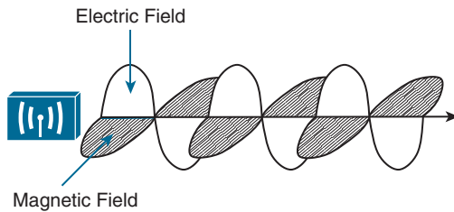
Figure 17-3 Traveling Electric and Magnetic Waves
