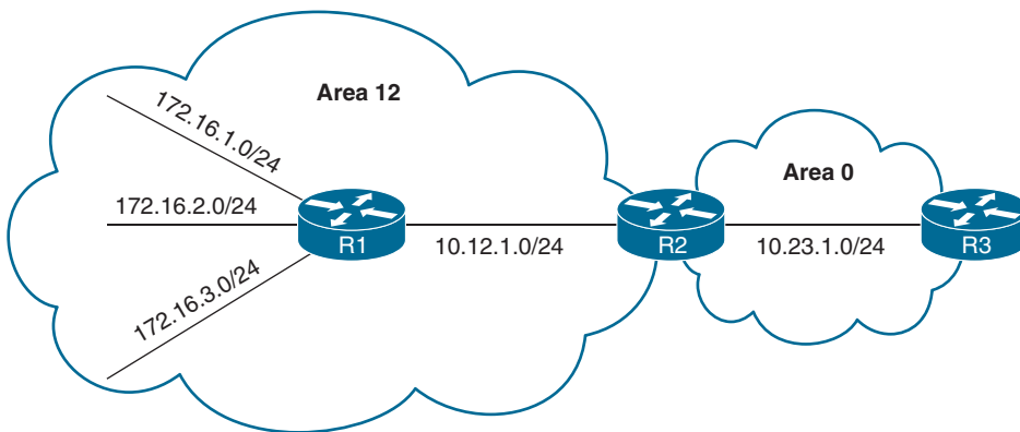
Figure 9-21 OSPF Inter-Area Summarization Example
