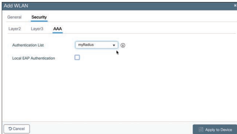
Figure 20-11 Selecting the Authentication Group to Authenticate Clients in the WLAN
