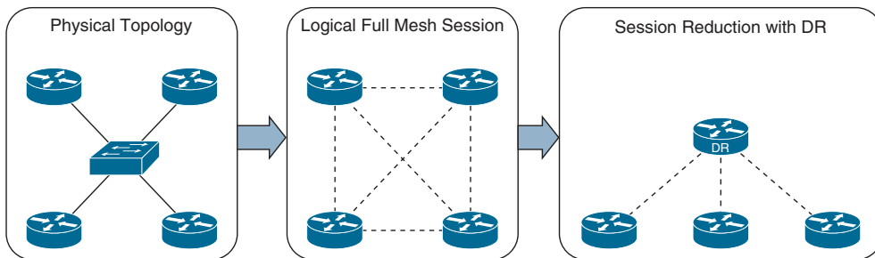
Figure 8-5 OSPF DR Concept
