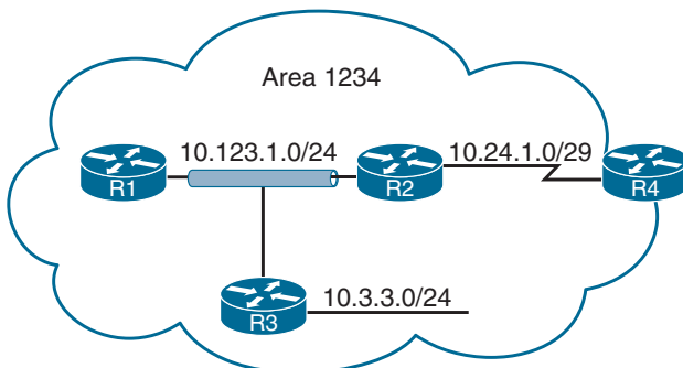
Figure 9-6 Type 1 LSA Flooding Reference Topology
