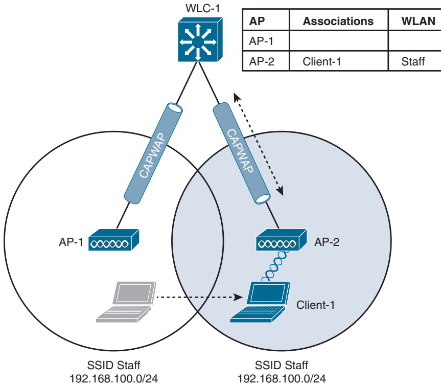
Figure 19-5 Cisco Wireless Network After an Intracontroller Roam
