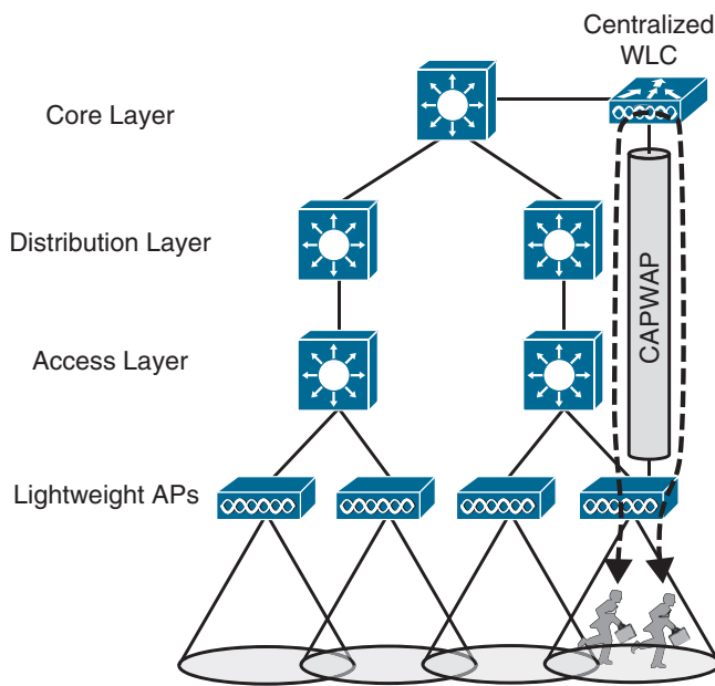
Figure 18-4 Shortest Data Path Through a Centralized Wireless Deployment
