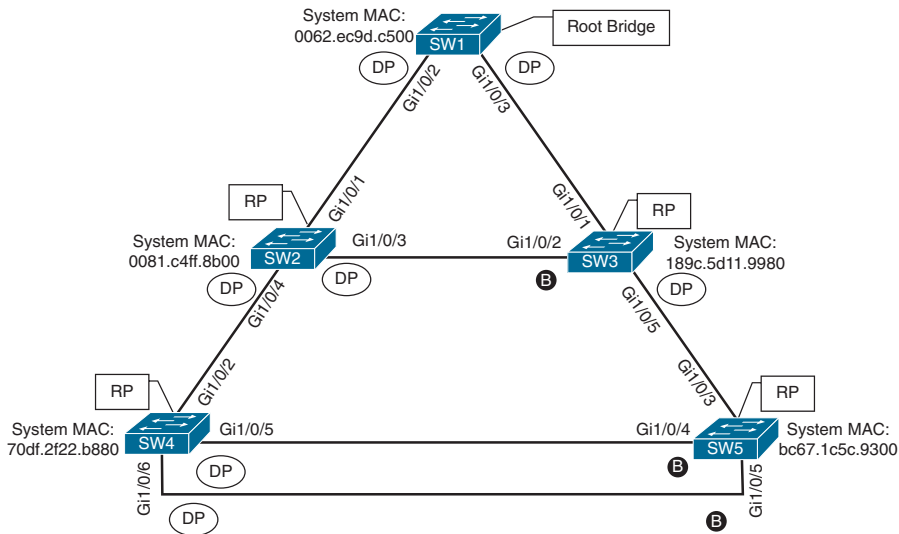
Figure 3-1 STP Topology for Tuning
