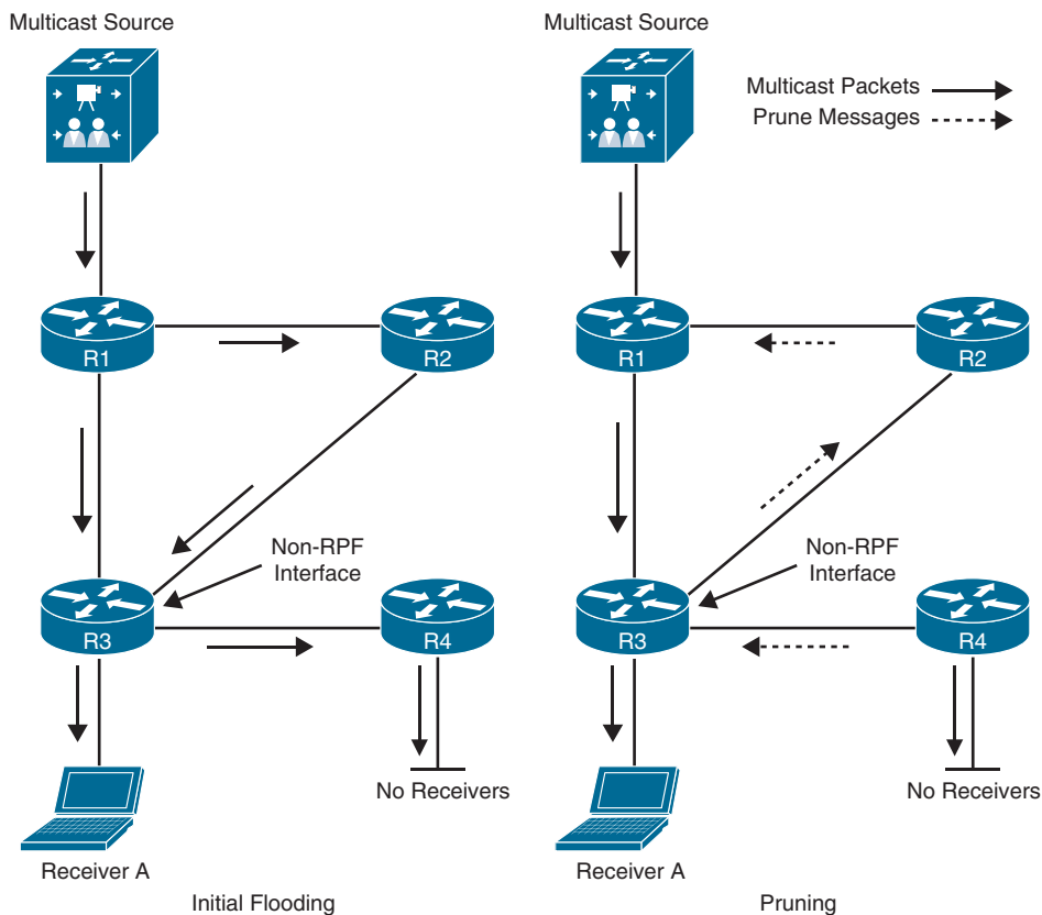
Figure 13-15 PIM-DM Flood and Prune Operation
