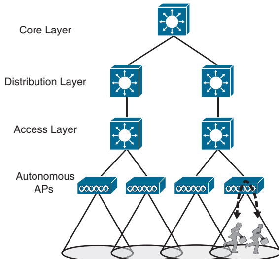
Figure 18-2 Shortest Data Path Through an Autonomous AP Topology
