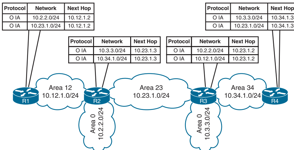
Figure 9-13 OSPF Routes for Discontiguous Network
