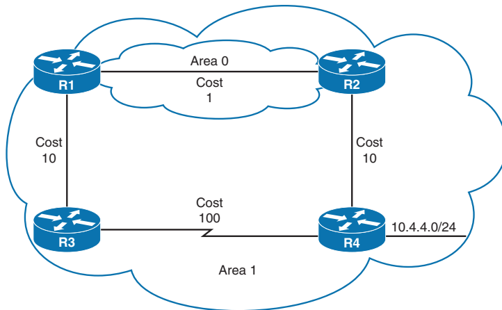
Figure 9-14 Intra-Area Routes over Inter-Area Routes
