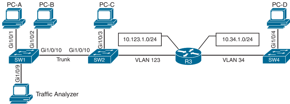
Figure 24-4 Sample Topology for Packet Captures
