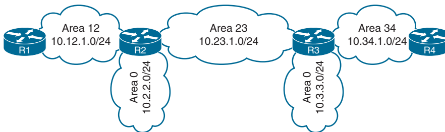
Figure 9-12 Discontiguous Network
