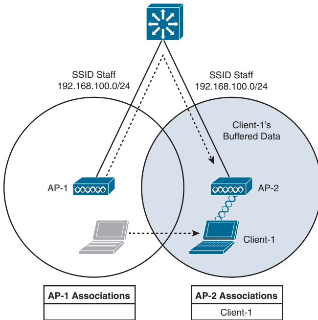
Figure 19-2 After Roaming Between Autonomous APs
