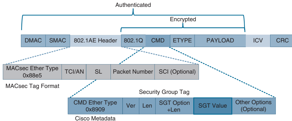
Figure 25-17 MACsec Ethernet Frame with SGT
