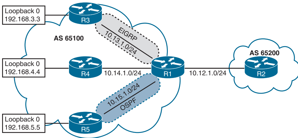
Figure 11-10 Multiple BGP Route Sources
