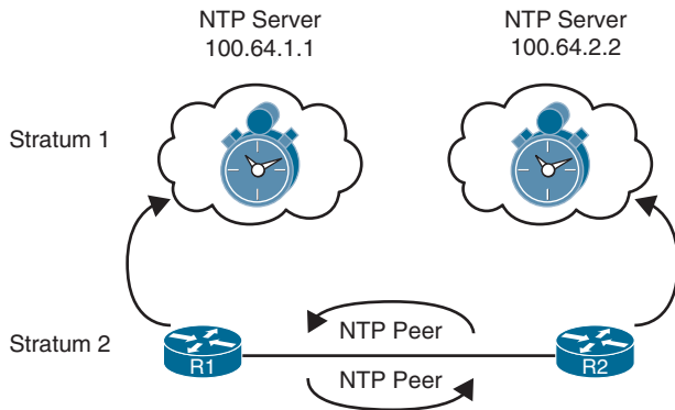
Figure 15-3 NTP Stratums
