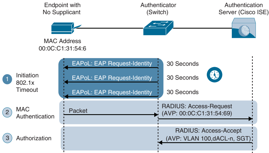
Figure 25-7 Successful MAB Authentication Process Flow
