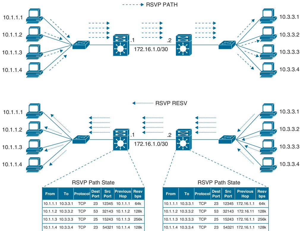
Figure 14-1 RSVP Reservation Establishment
