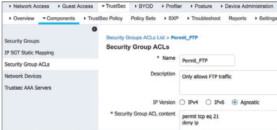
Figure 25-15 Permit FTP SGACL Contents
