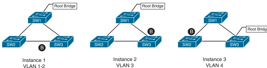
Figure 4-3 MST Topologies
