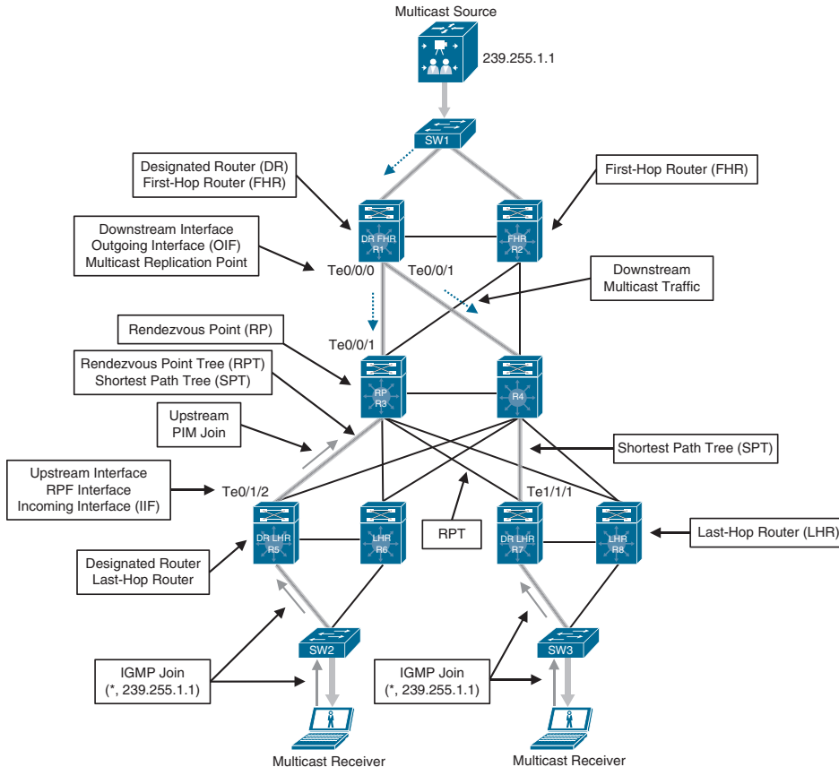
Figure 13-14 PIM Terminology Illustration
