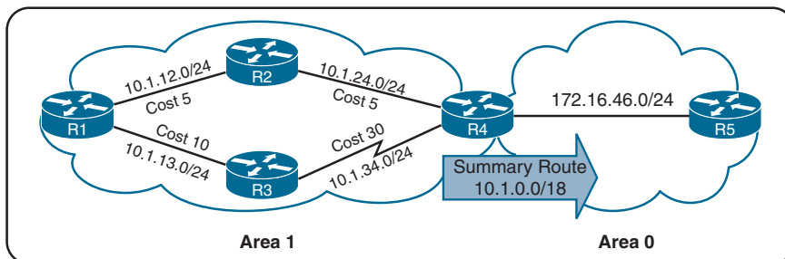
Figure 9-18 Topology Example with Summarization
