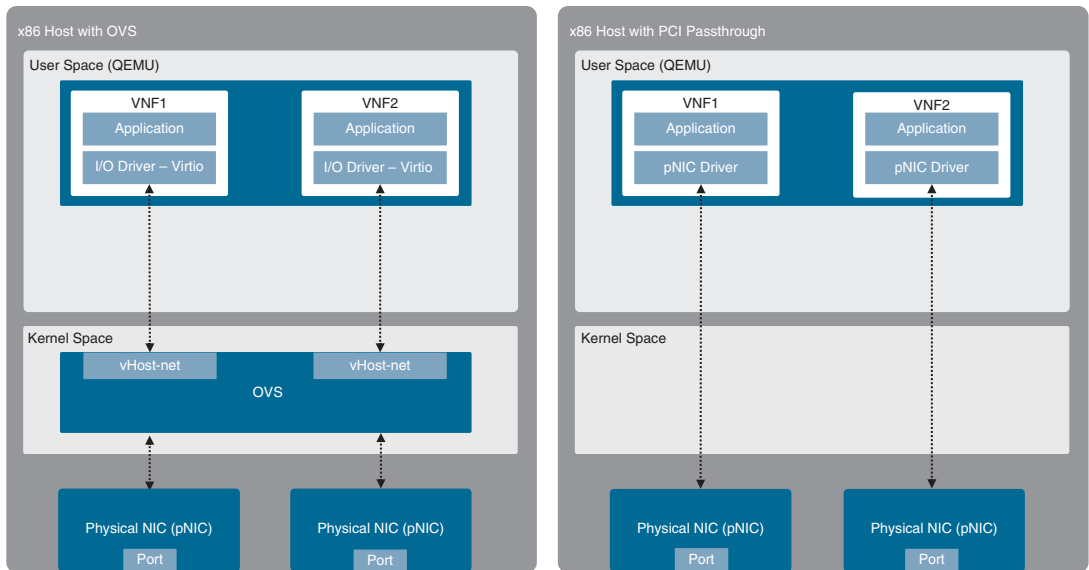
Figure 27-12 Standard OVS and PCI Passthrough
