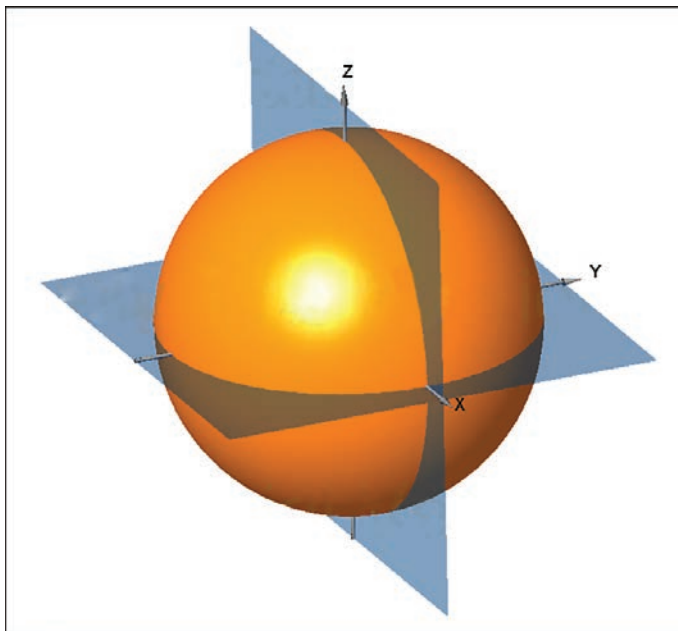
Figure 18-11 Plotting the Radiation Pattern of an Isotropic Antenna
