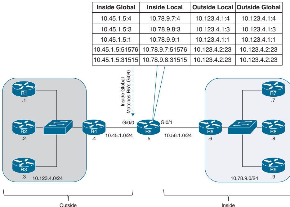
Figure 15-11 R5’s Translation Table for PAT
