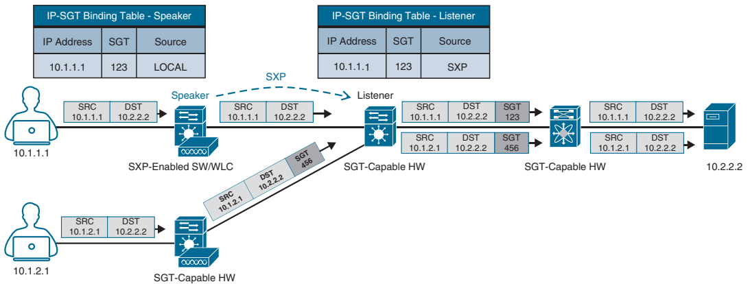
Figure 25-11 Inline Tagging and SXP Propagation
