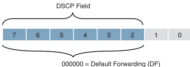
Figure 14-7 Default Forwarding (DF) PHB
