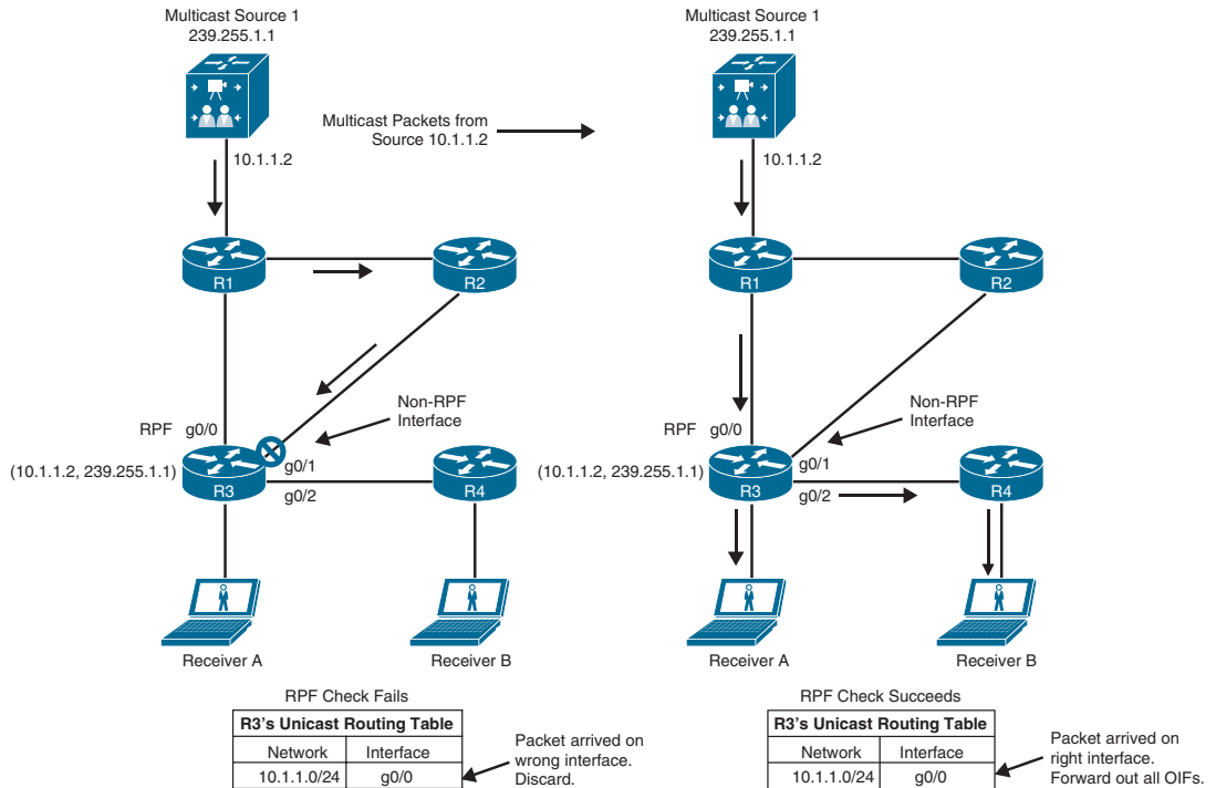
Figure 13-19 RPF Check
