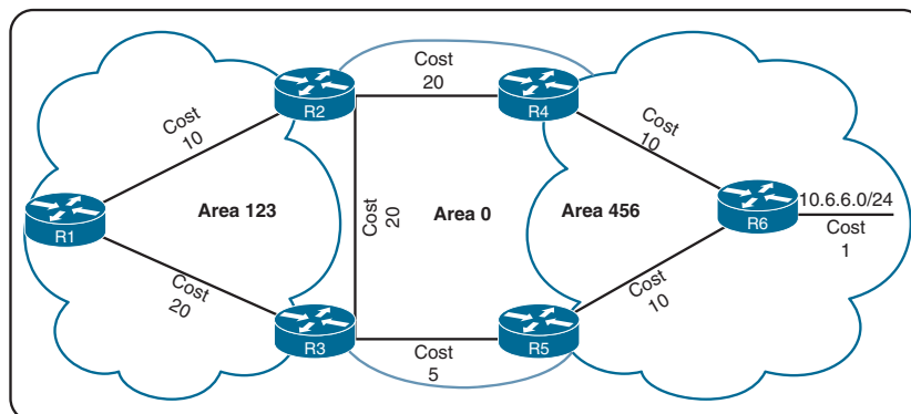
Figure 9-15 Inter-Area Route Selection
