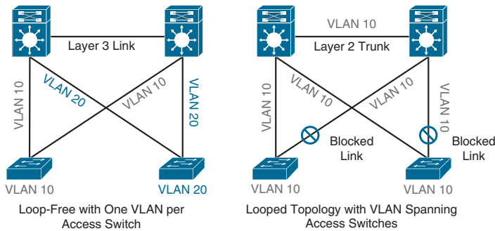
Figure 22-9 Loop-Free Topology and Looped Topology
