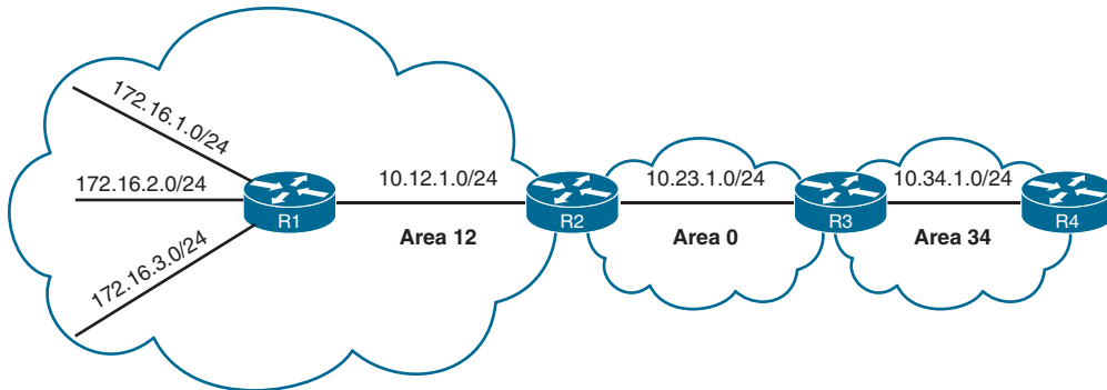
Figure 9-22 Expanded Topology for Filtering Routes
