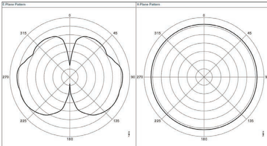
Figure 18-17 E and H Radiation Patterns for a Typical Dipole Antenna
