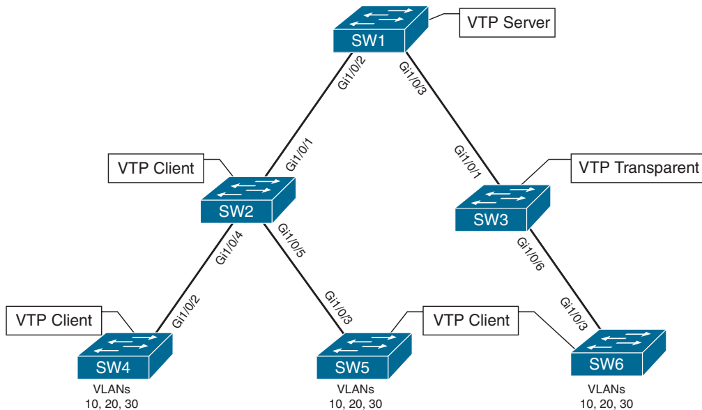
Figure 5-1 Sample Topology for VTP
