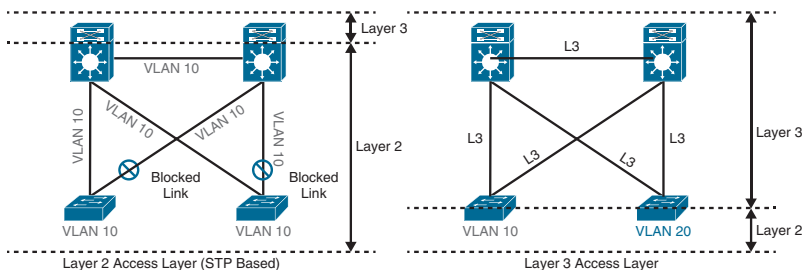
Figure 22-10 Layer 2 Access Layer and Layer 3 Access Layer
