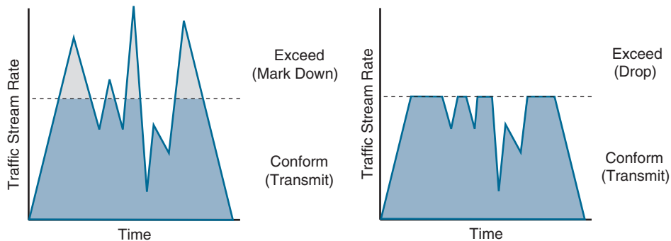
Figure 14-14 Single-Rate Two-Color Marker/Policer
