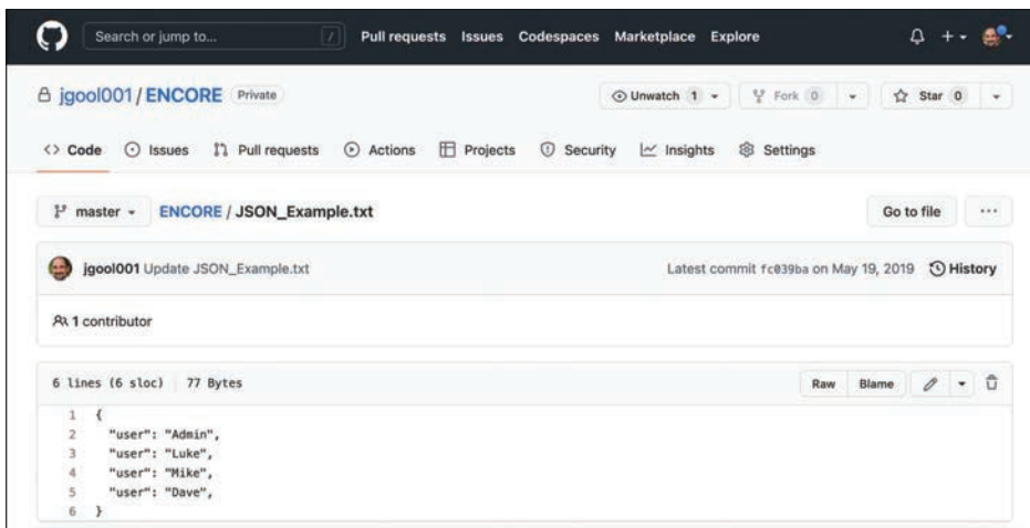
Figure 28-22 JSON_Example.txt Contents
