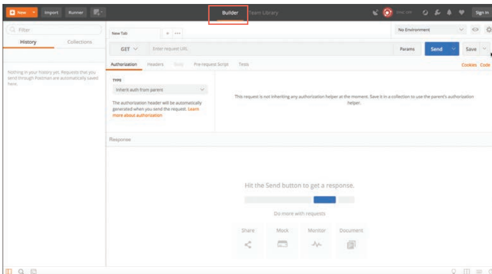
Figure 28-2 Postman Dashboard
