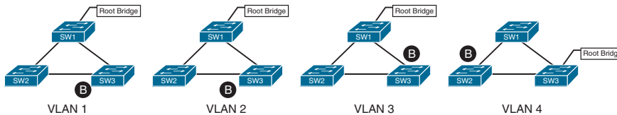
Figure 4-2 Per-VLAN Spanning Tree (PVST) Topologies
