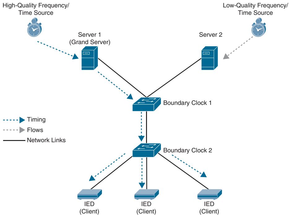
Figure 15-4 PTP Hierarchy
