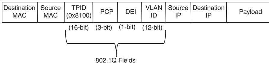
Figure 1-4 VLAN Packet Structure
