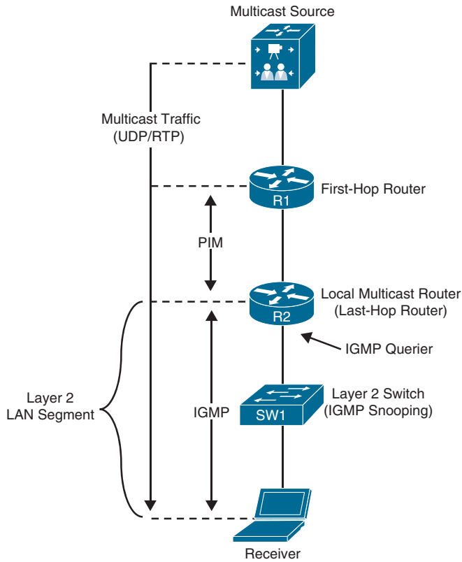
Figure 13-1 Multicast Architecture
