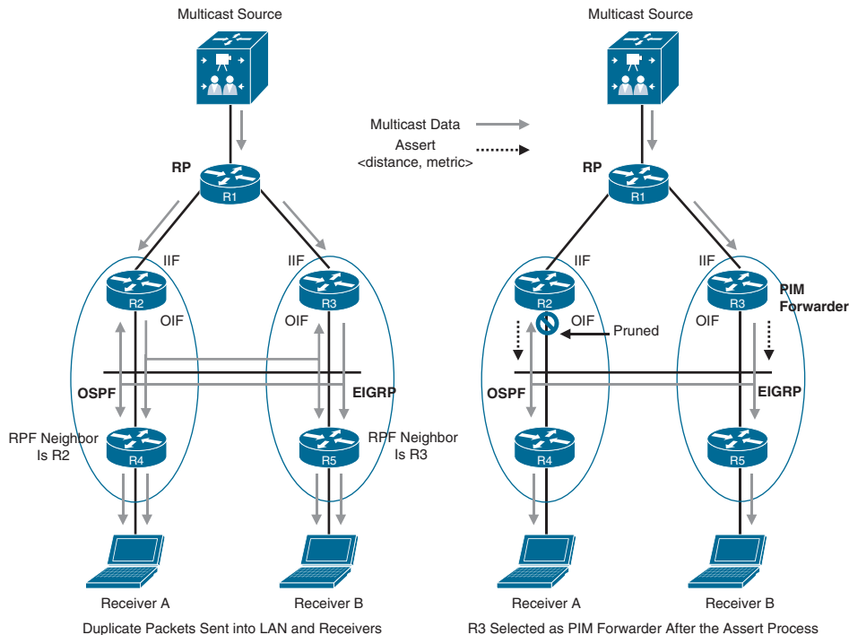
Figure 13-21 PIM-SM PIM Forwarder Example
