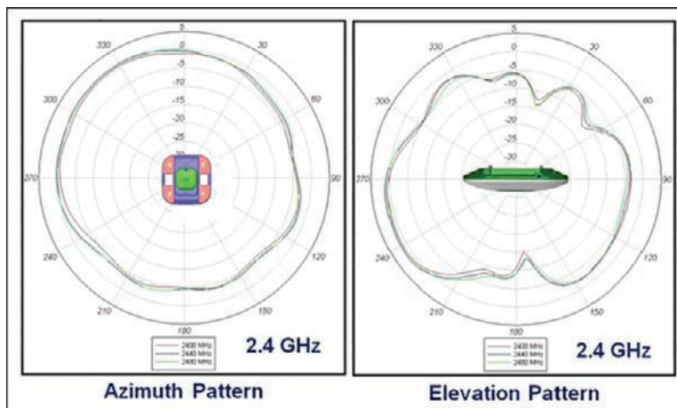
Figure 18-20 E and H Radiation Patterns for a Typical Integrated Omnidirectional Antenna
