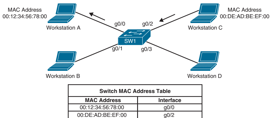
Figure 13-9 Known Destination Is Not Flooded
