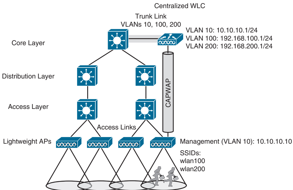
Figure 18-3 WLC Location in a Centralized Wireless Deployment
