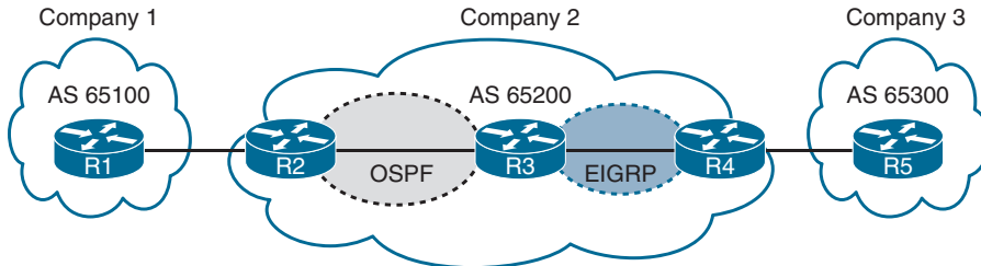
Figure 11-3 AS 65200 Providing Transit Connectivity
