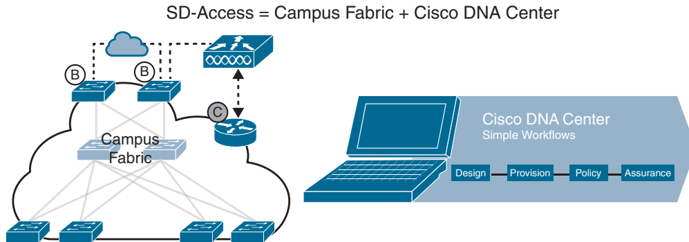
Figure 23-1 SD-Access Solution
