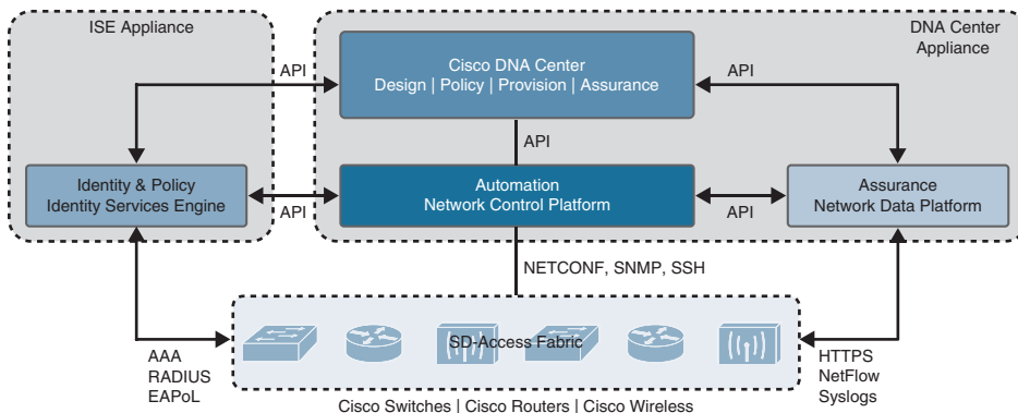
Figure 23-8 SD-Access Main Components
