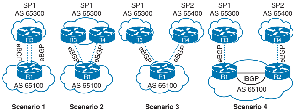
Figure 12-1 Common BGP Multihoming Scenarios
