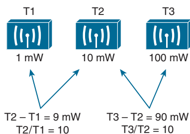
Figure 17-14 Comparing Power Levels Between Transmitters
