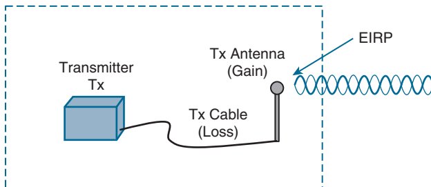
Figure 17-20 Calculating EIRP
