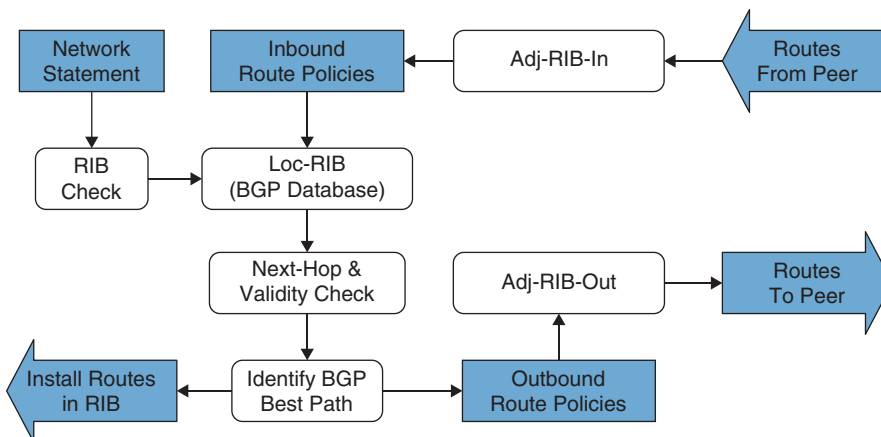
Figure 12-9 BGP Route Policy Processing
