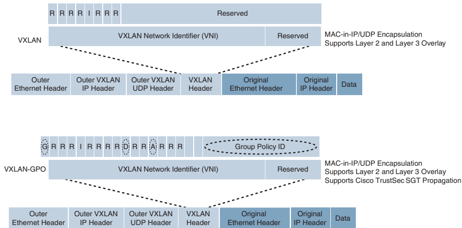
Figure 23-5 VXLAN and VXLAN-GPO Packet Format Comparison
