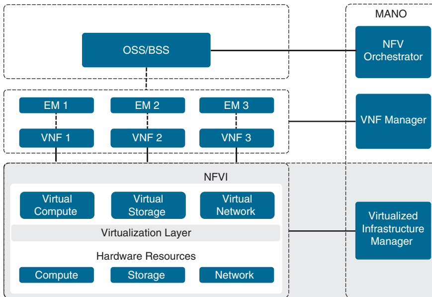
Figure 27-7 ETSI NFV Architectural Framework
