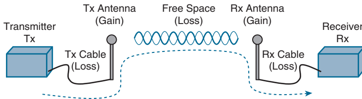
Figure 17-21 Calculating Received Signal Strength Over the Path of an RF Signal
