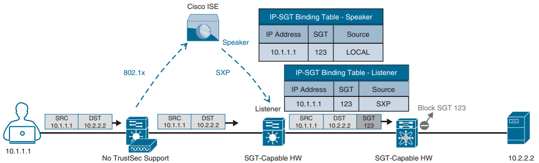
Figure 25-13 TrustSec Enforcement with SGACL
