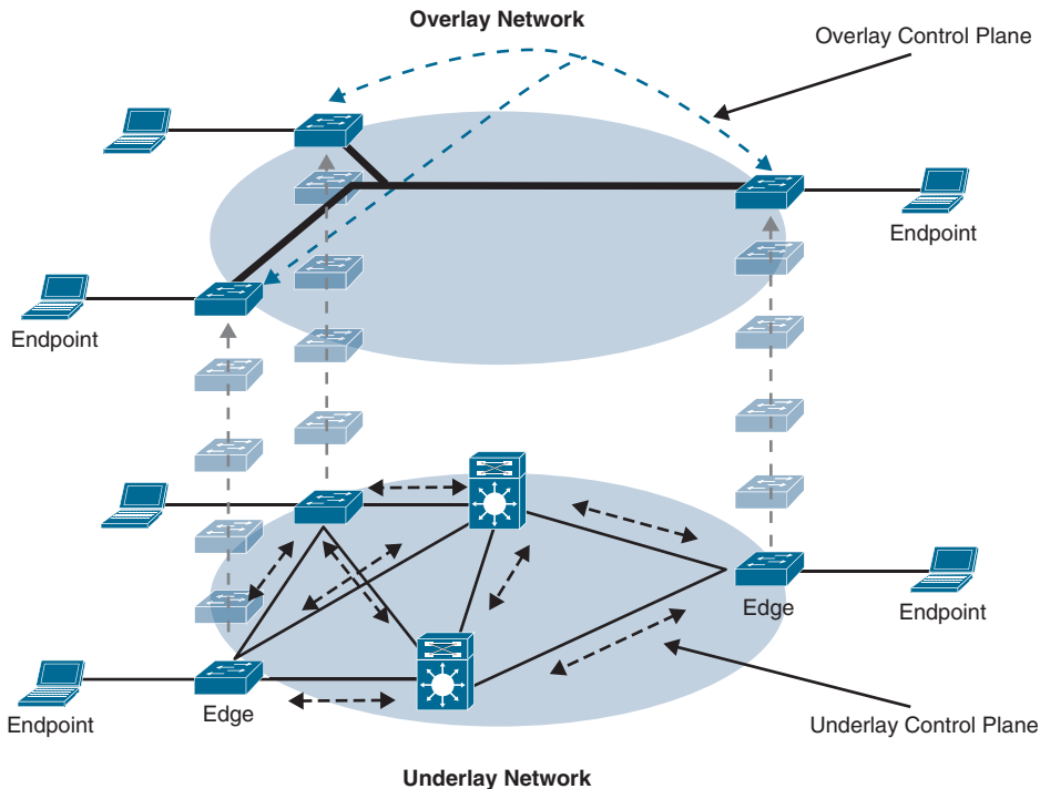
Figure 23-3 Underlay and Overlay Networks
