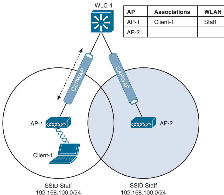
Figure 19-4 Cisco Wireless Network Before an Intracontroller Roam
