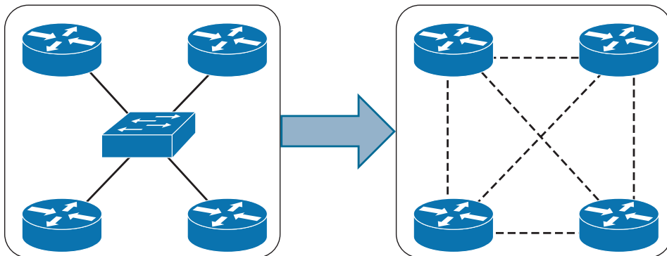
Figure 8-3 Multi-Access Physical Topology Versus Logical Topology
