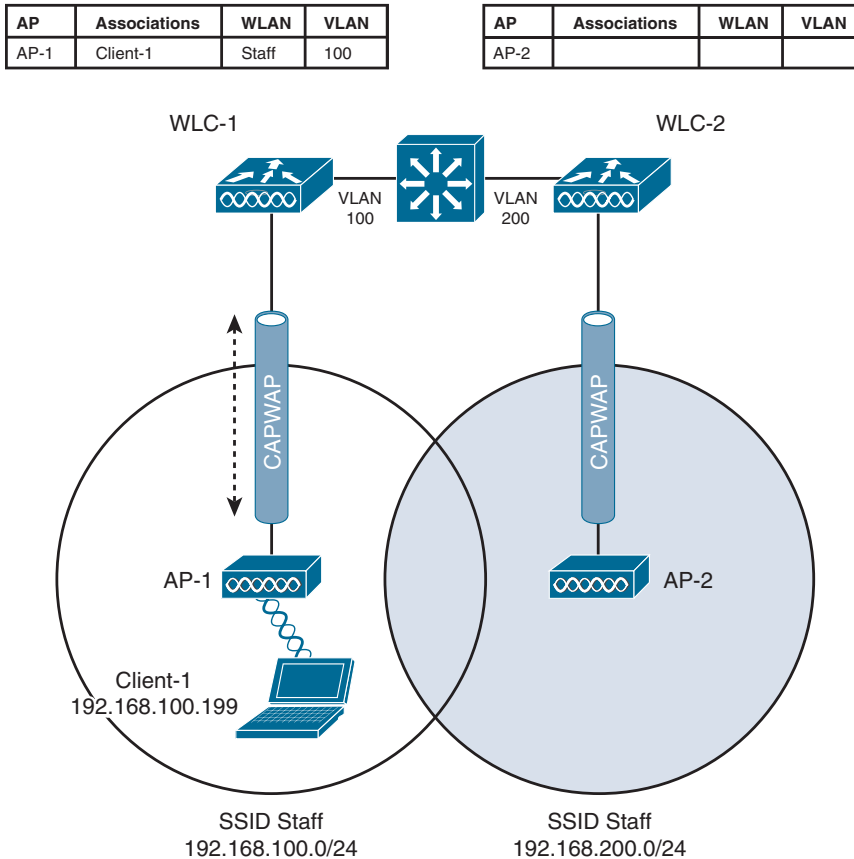
Figure 19-8 Before a Layer 3 Intercontroller Roam
