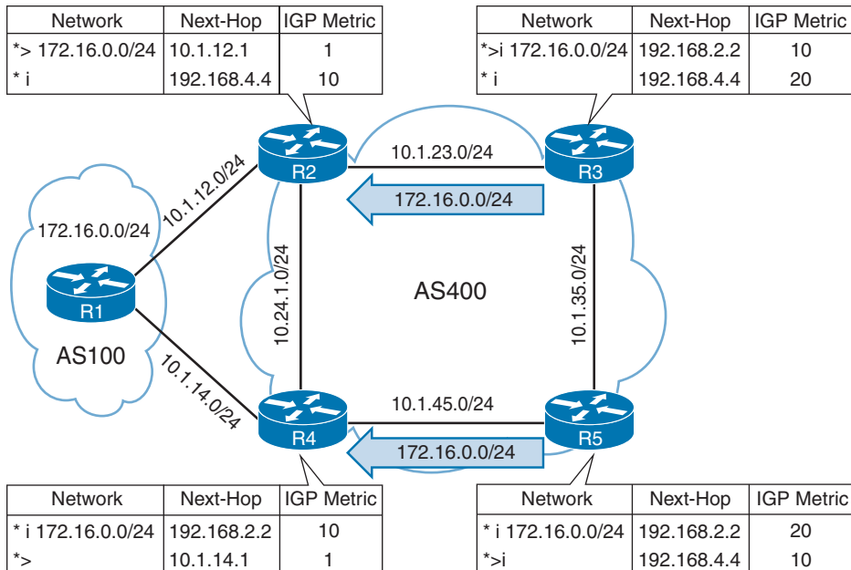
Figure 12-12 Lowest IGP Metric Topology
