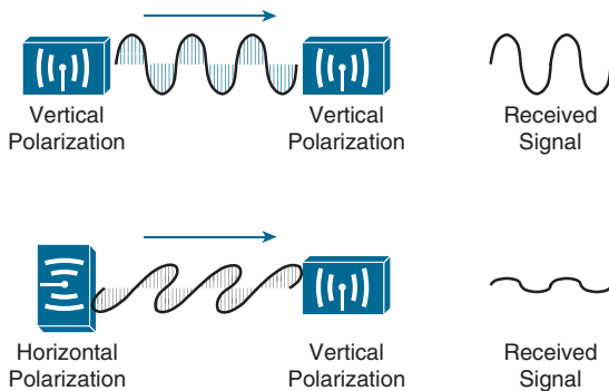
Figure 18-15 Matching the Antenna Polarization Between Transmitter and Receiver
