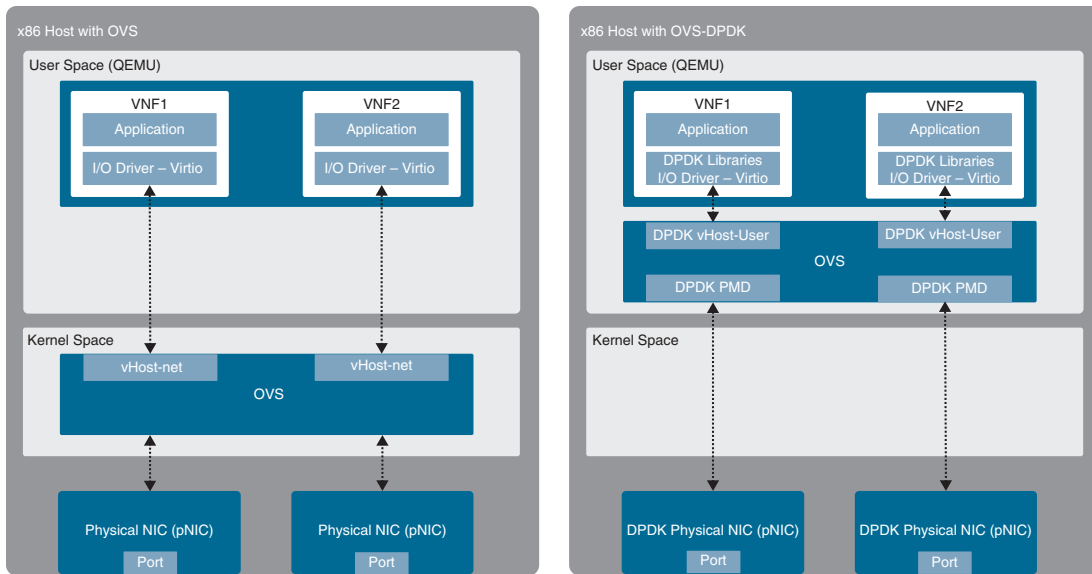
Figure 27-11 Standard OVS and OVS-DPDK
