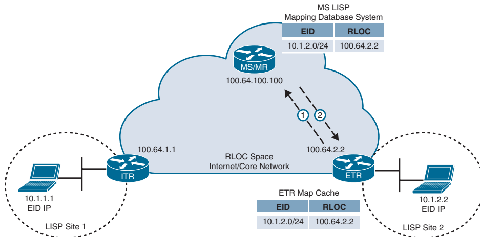
Figure 16-8 Map Registration and Notification
