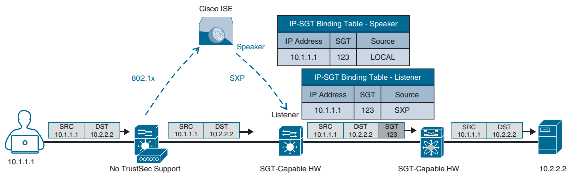
Figure 25-12 SXP Peering Between Cisco ISE and TrustSec-Capable Devices
