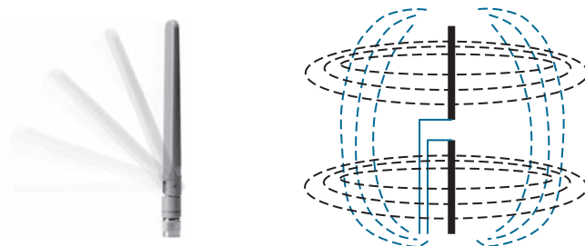
Figure 18-16 Cisco Dipole Antenna
