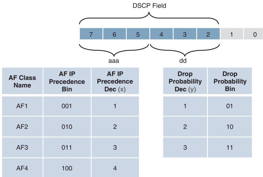
Figure 14-8 Assured Forwarding (AF) PHB
