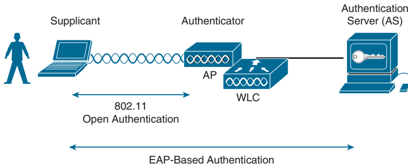
Figure 20-6 802.1x Client Authentication Roles
