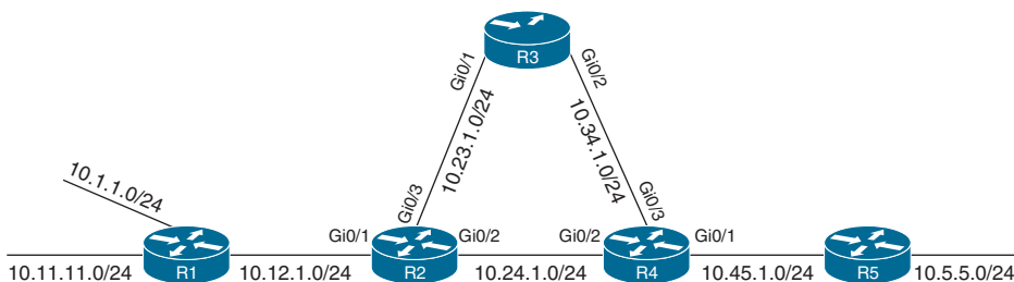
Figure 6-14 PBR Next-Hop Topology
