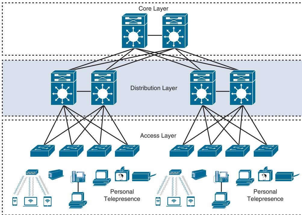
Figure 22-4 Distribution Layer Connectivity
