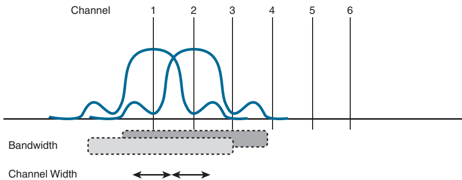
Figure 17-10 Overlapping Channel Spacing
