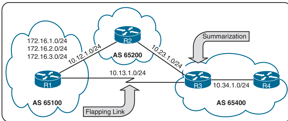
Figure 11-11 BGP Route Summarization Hiding Link Flaps
