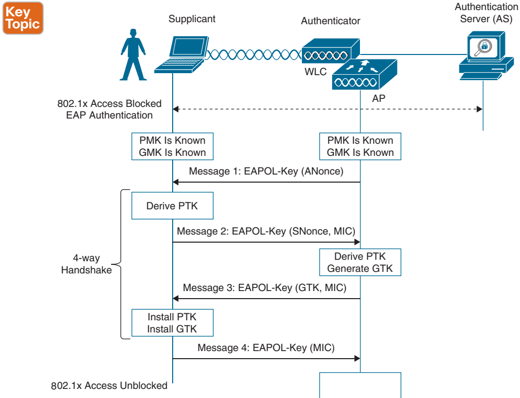
Figure 20-7 Message Exchange During the Four-Way EAPOL Handshake
