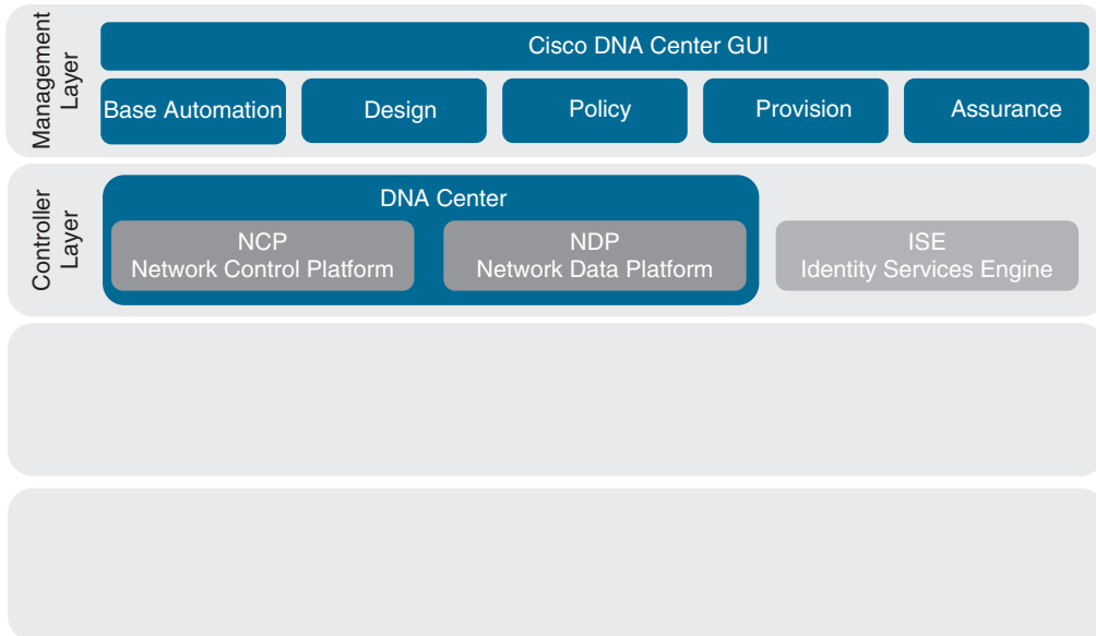
Figure 23-2 Cisco SD-Access Architecture
