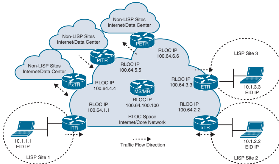
Figure 16-5 LISP Architecture Reference Topology
