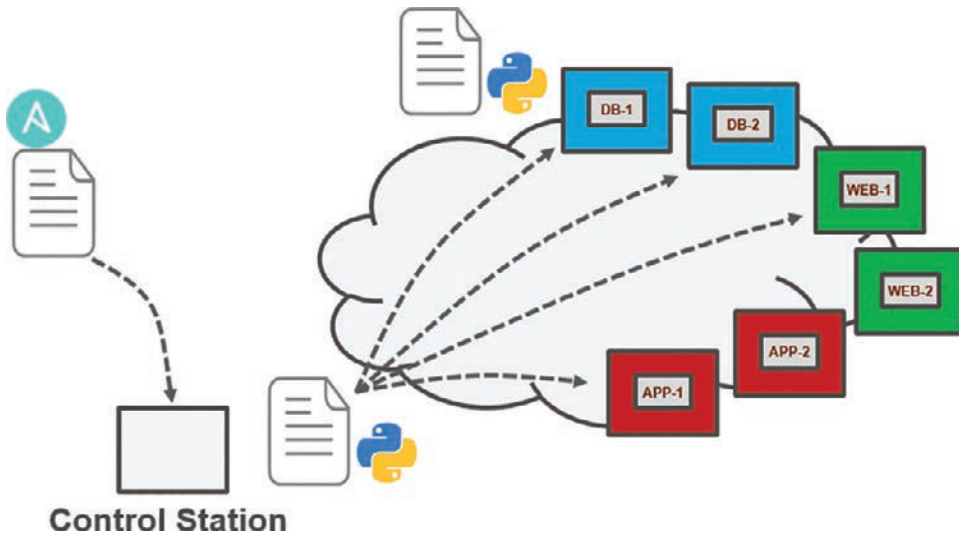
Figure 29-8 Ansible Workflow
