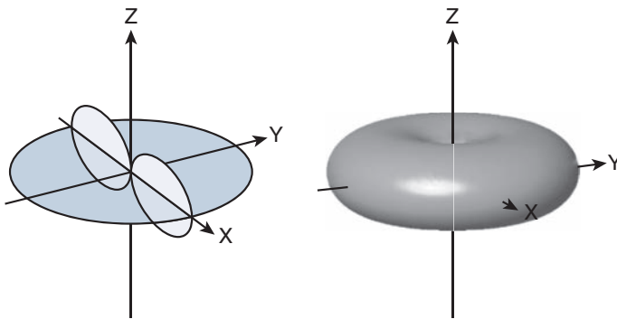
Figure 18-18 Dipole Radiation Pattern in Three Dimensions
