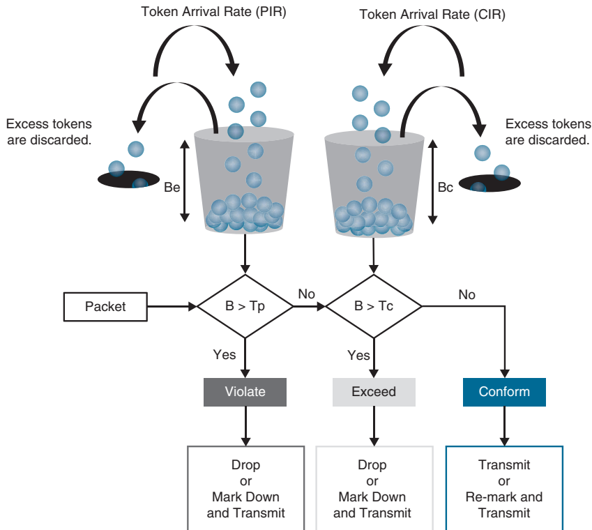
Figure 14-18 Two-Rate Three-Color Marker/Policer Token Bucket Algorithm
