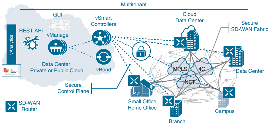
Figure 23-13 SD-WAN Solution Architecture
