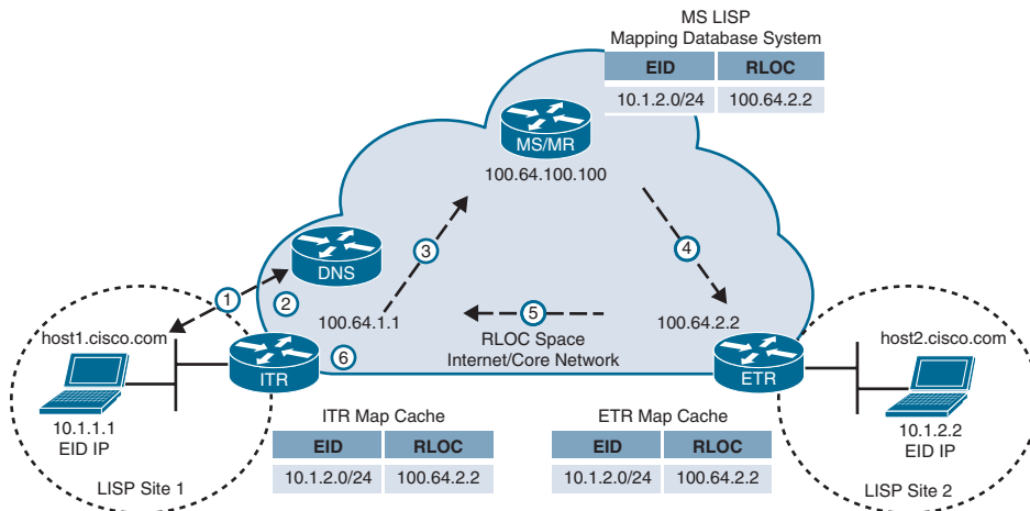
Figure 16-9 Map Request and Reply
