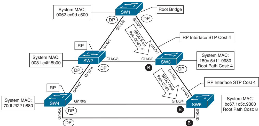
Figure 3-2 STP Path Cost Calculation
