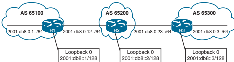
Figure 11-13 IPv6 Sample Topology
