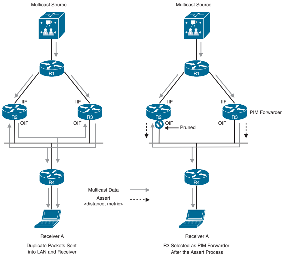
Figure 13-20 PIM Forwarder Example
