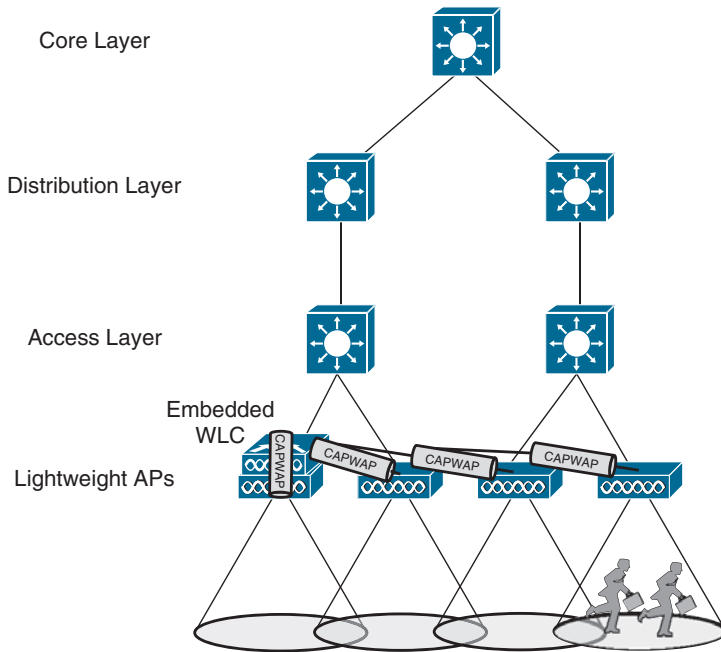
Figure 18-7 WLC Location in a Controller-less Deployment Using EWC
