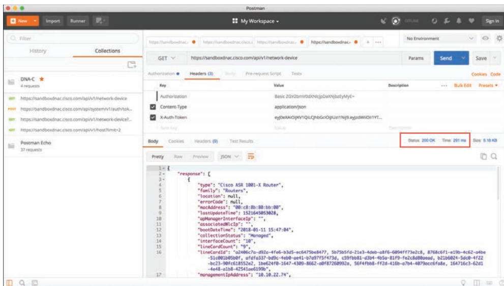
Figure 28-9 Postman Setup for Retrieving the Network Device Inventory with an API Call
