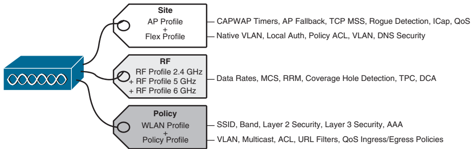
Figure 18-9 AP Configuration with Profiles and Tags with an IOS XE Controller
