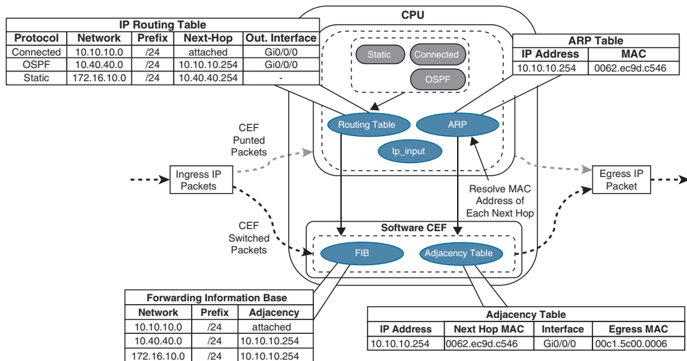
Figure 1-8 CEF Switching
