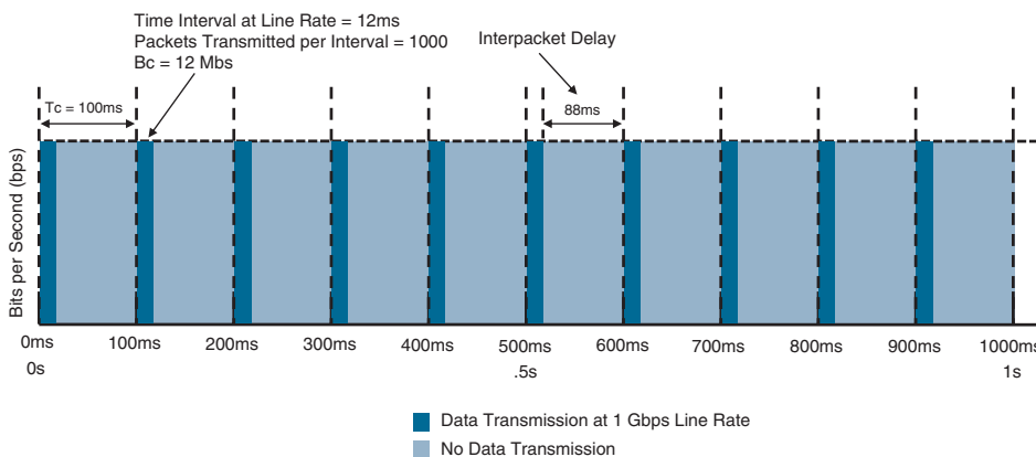
Figure 14-13 Token Bucket Operation
