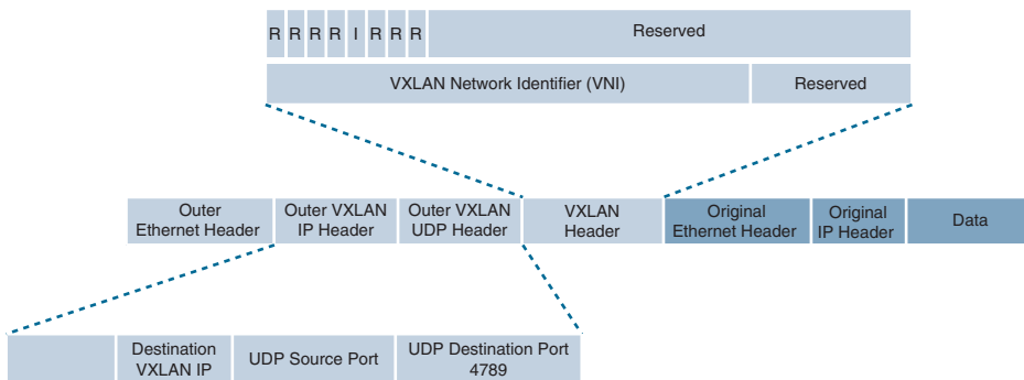
Figure 16-13 VXLAN Packet Format
