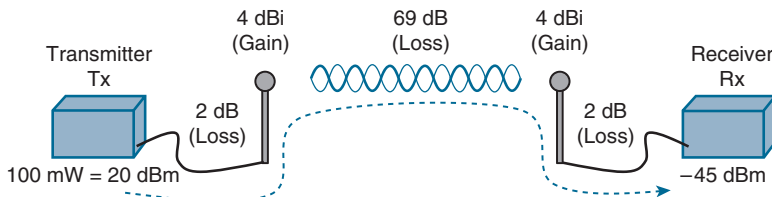
Figure 17-22 Example of Calculating Received Signal Strength
