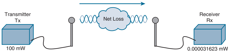
Figure 17-18 Example of RF Signal Power Loss
