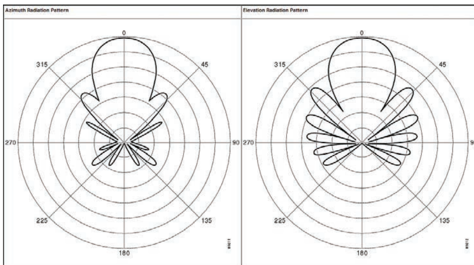
Figure 18-25 E and H Radiation Patterns for a Typical Yagi Antenna
