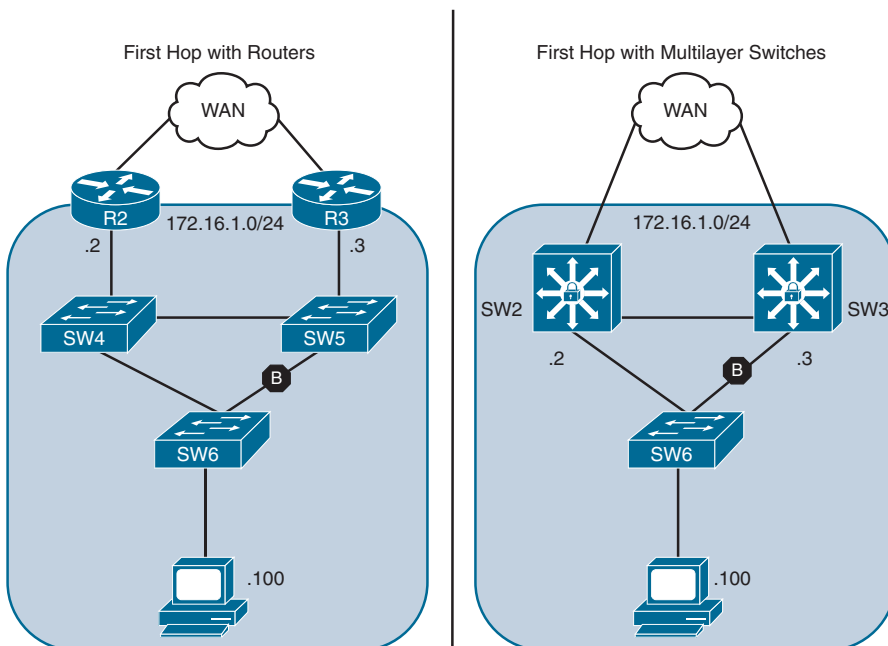
Figure 15-5 Resiliency with Redundancy with Layer 2 and Layer 3 Devices
