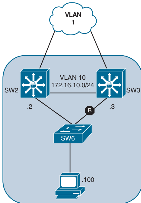
Figure 15-7 Sample HSRP Topology
