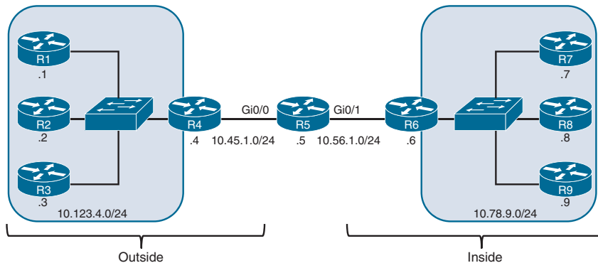
Figure 15-8 NAT Topology
