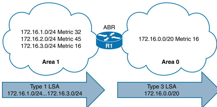
Figure 9-20 Inter-Area Summarization Metric
