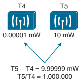
Figure 17-15 Comparing Power Levels That Differ by Orders of Magnitude
