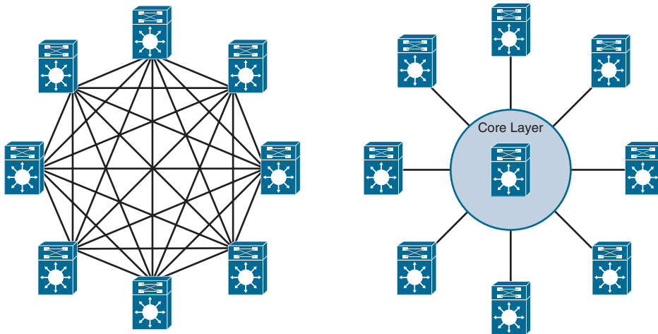
Figure 22-6 Core Layer Reduces Large Network Complexity
