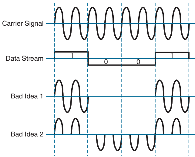
Figure 17-27 Poor Attempts at Sending Data over an RF Signal
