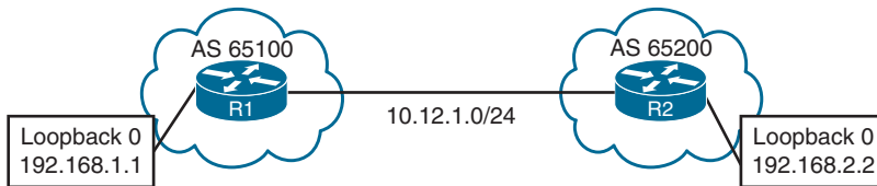
Figure 11-7 Simple BGP Topology
