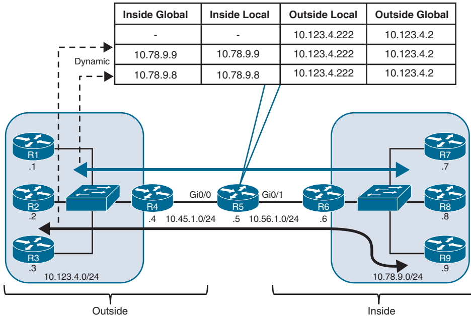
Figure 15-10 Outside Static NAT Topology for R2 as 10.123.4.222
