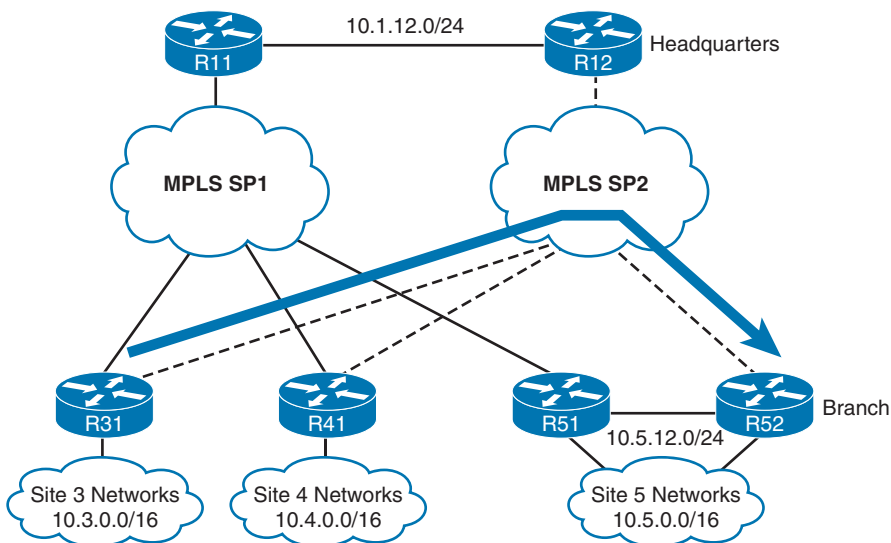
Figure 12-3 Deterministic Routing
