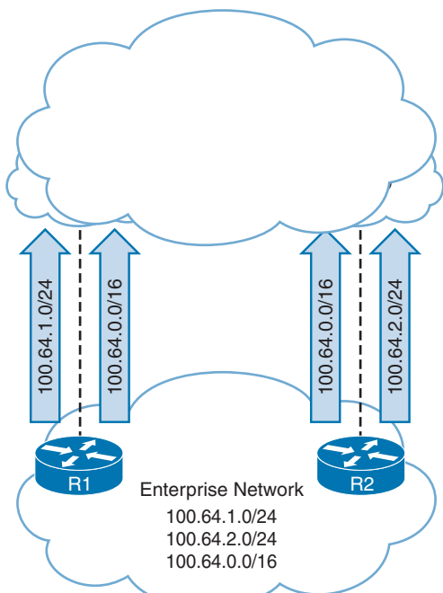
Figure 12-10 BGP Path Selection Using Longest Match
