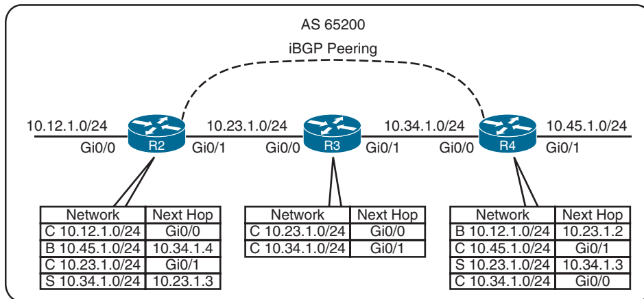
Figure 11-4 iBGP Prefix Advertisement Behavior
