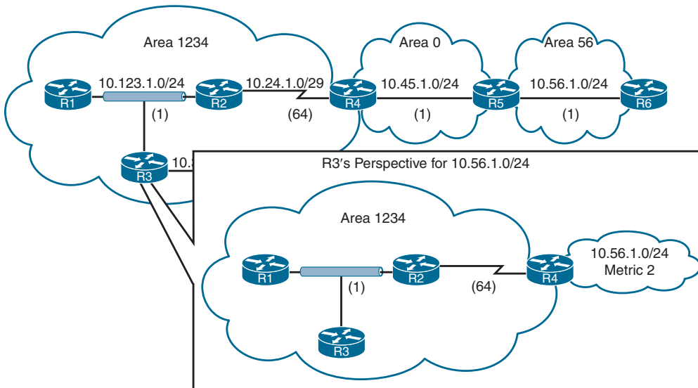
Figure 9-11 Visualization of 10.56.1.0/24 Type 3 LSA from Area 1234
