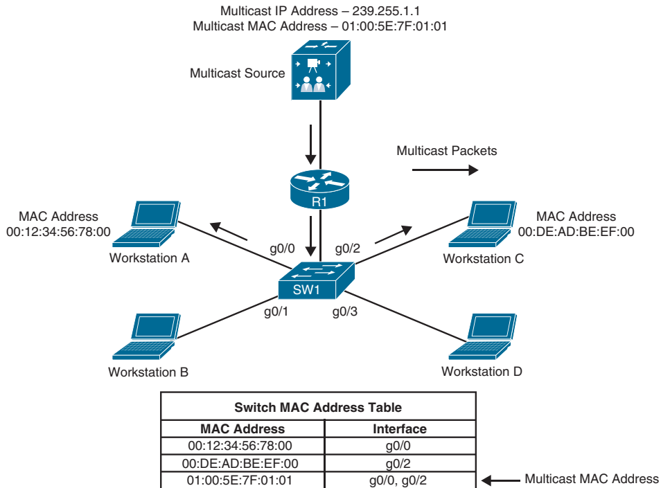
Figure 13-11 No Flooding with IGMP Snooping
