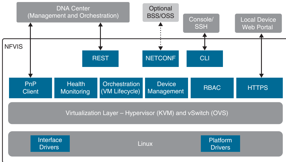
Figure 27-16 NFVIS Components
