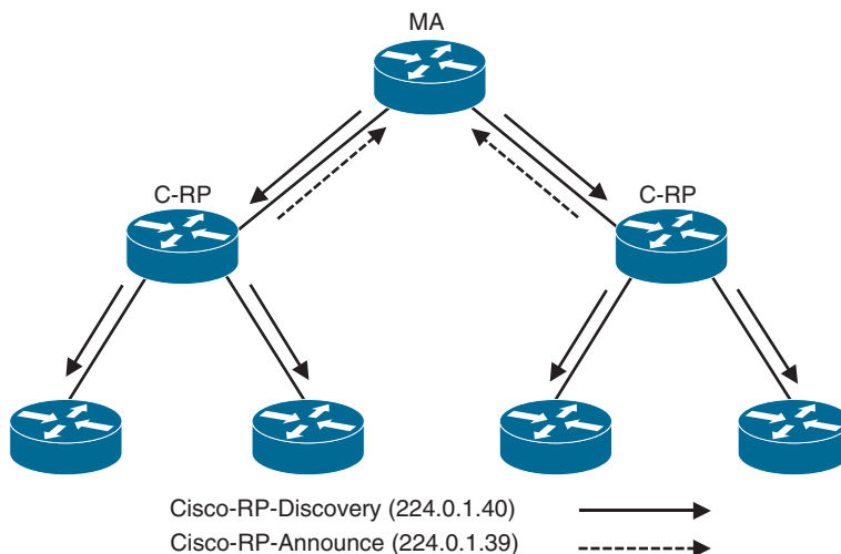
Figure 13-22 Auto-RP Mechanism
