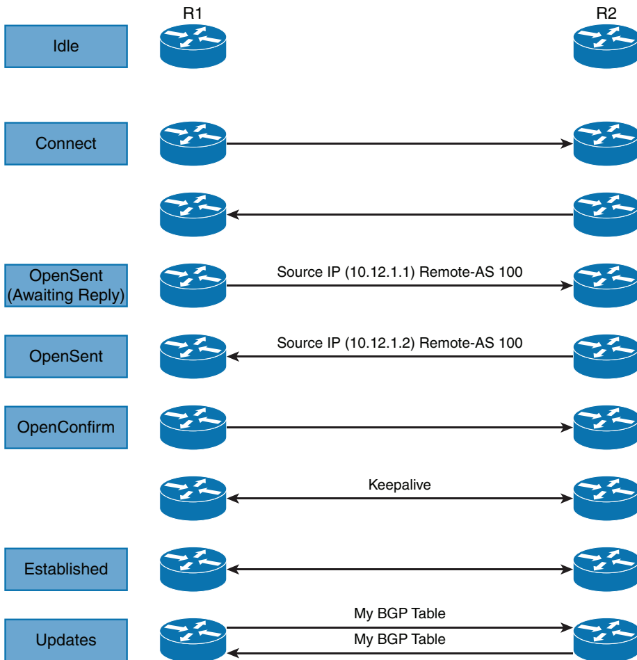
Figure 11-6 BGP Neighbor States with Session Establishment
