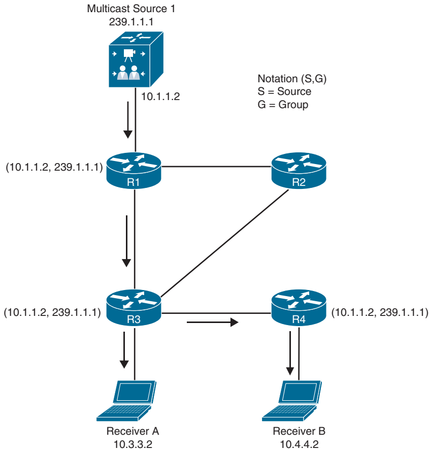
Figure 13-12 Source Tree Example
