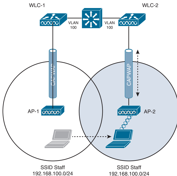
Figure 19-7 After an Intercontroller Roam
