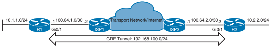
Figure 16-2 GRE Tunnel Topology
