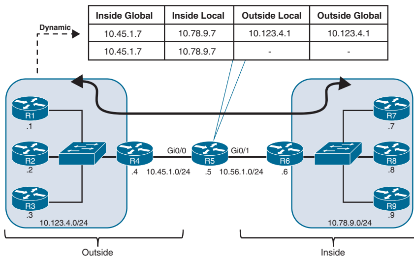
Figure 15-9 Inside Static NAT Topology for R7 as 10.45.1.7
