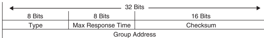
Figure 13-7 IGMP Message Format
