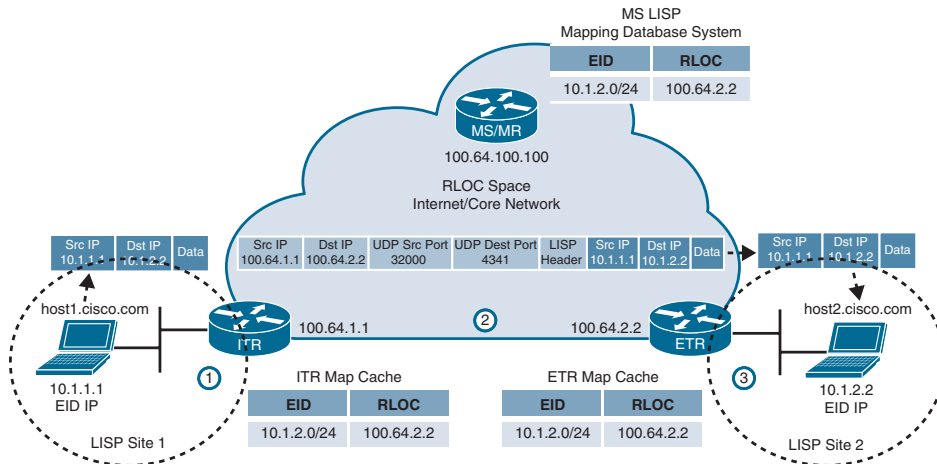
Figure 16-10 LISP Data Path
