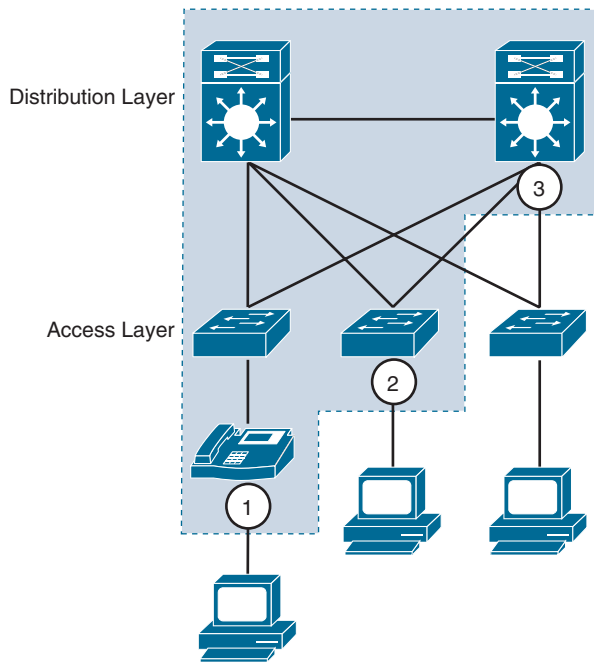
Figure 14-9 Trust Boundaries
