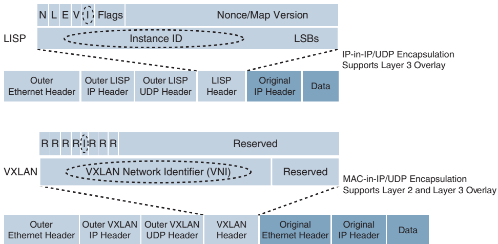
Figure 23-4 LISP and VXLAN Packet Format Comparison
