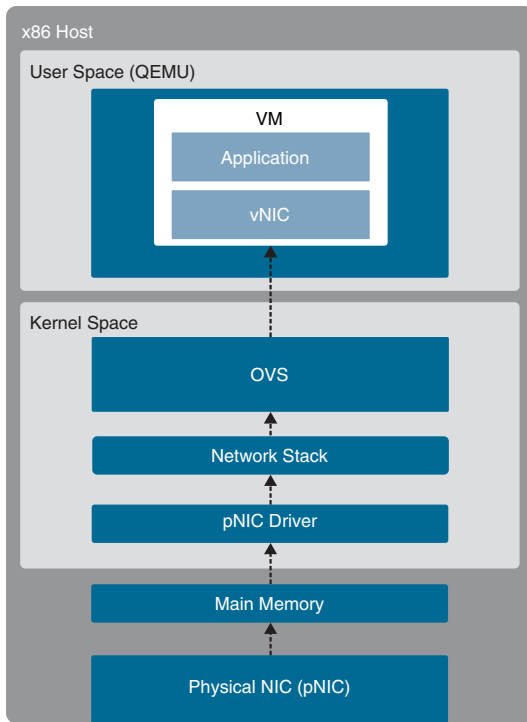
Figure 27-10 x86 Host with OVS
