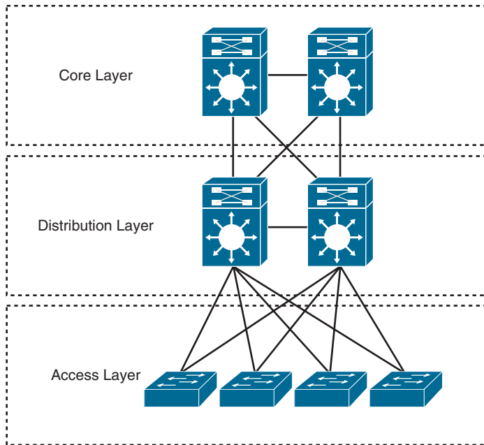
Figure 22-1 Hierarchical LAN Design
