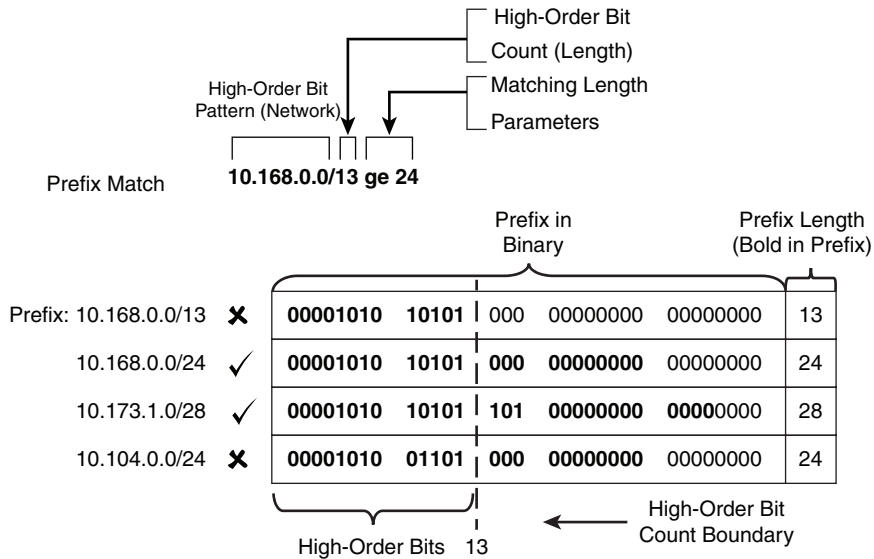
Figure 12-7 Prefix Match Pattern with Matching Length Parameters
