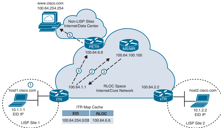
Figure 16-11 Proxy ETR Process
