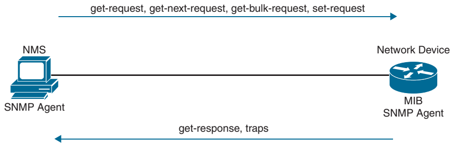
Figure 24-3 SNMP Communication Between NMS Host and Network Device
