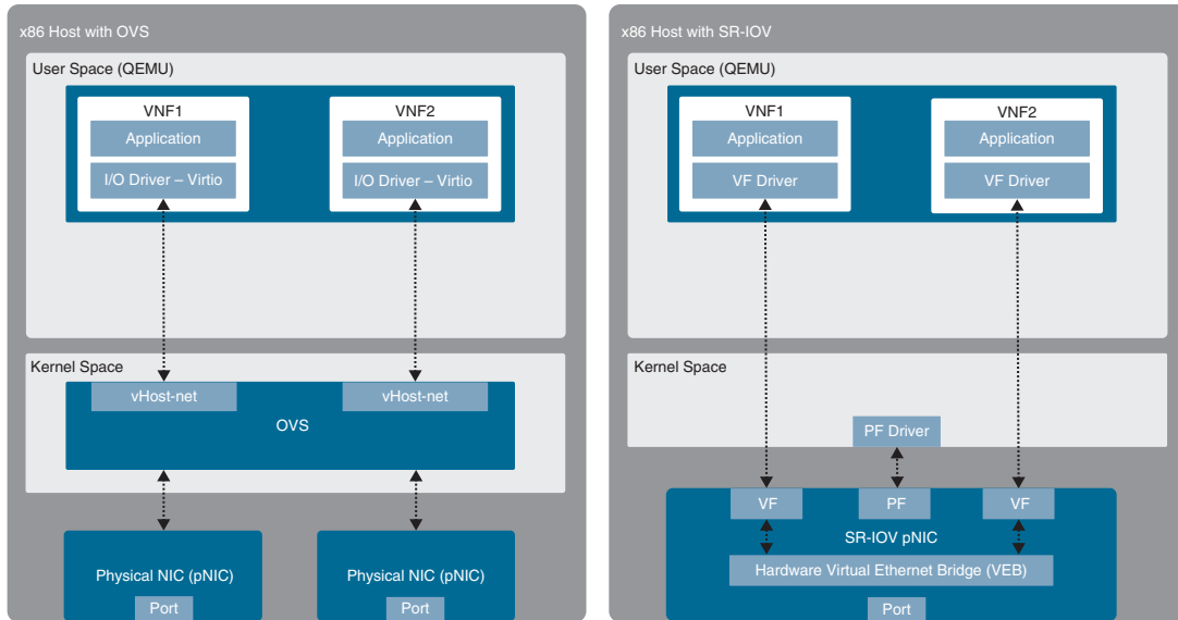
Figure 27-13 Standard OVS and SR-IOV
