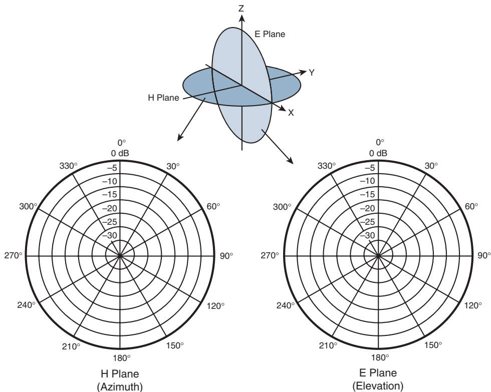
Figure 18-12 Recording an Isotropic Antenna Pattern on E and H Polar Plots
