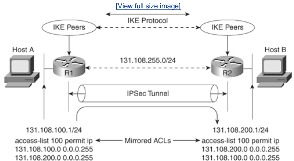
Figure 4-16. Typical IPsec Topology Between Two Remote Routers
