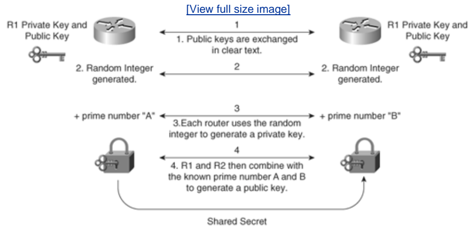
Figure 4-7. Diffie-Hellman Key Exchange
