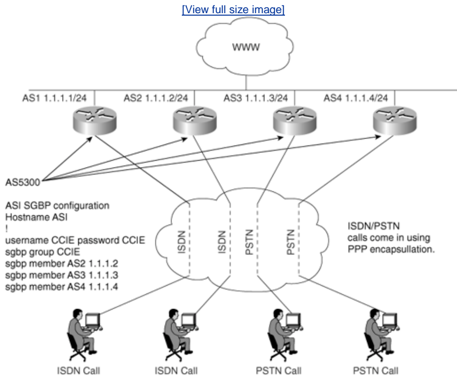
Figure 1-20. AS5300 Typical Design Scenario
