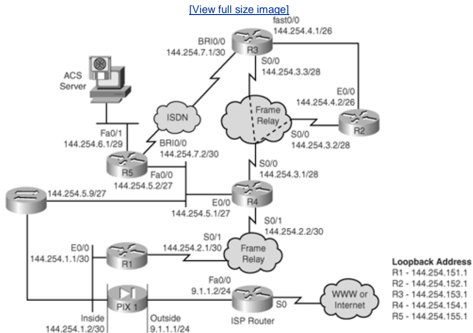
Figure 8-1. Lab Topology
