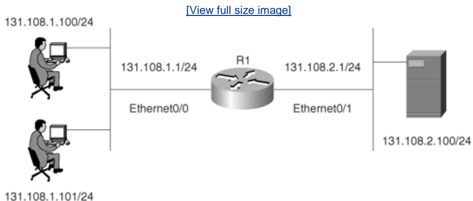
Figure 3-10. Scenario Physical Topology
