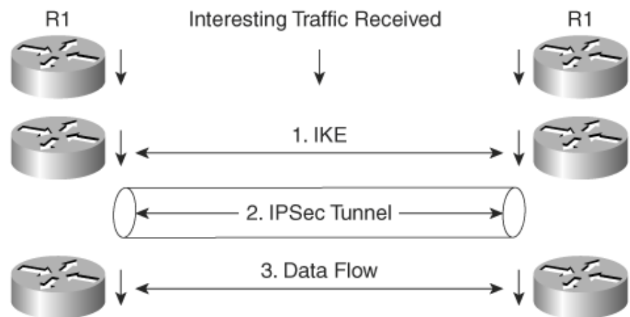
Figure 4-15. IPsec Flow
