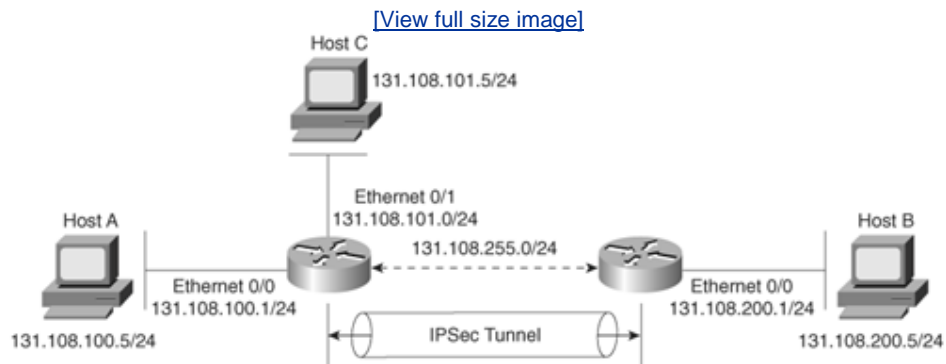
Figure 4-21. Scenario Topology
