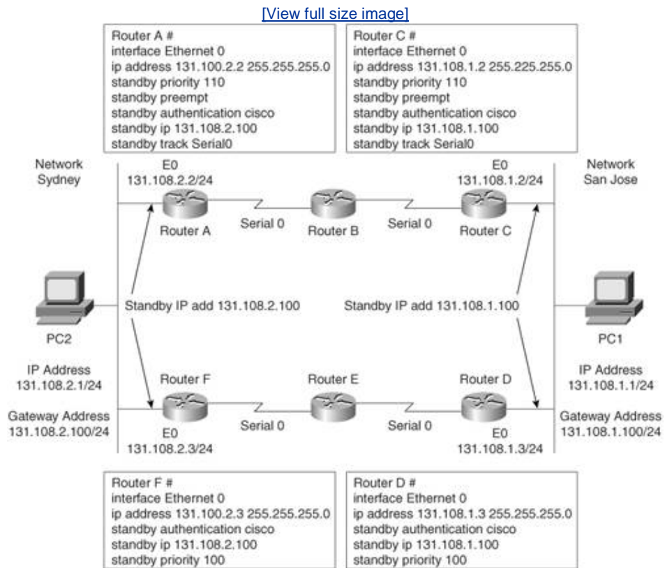
Figure 1-12. HSRP Example
