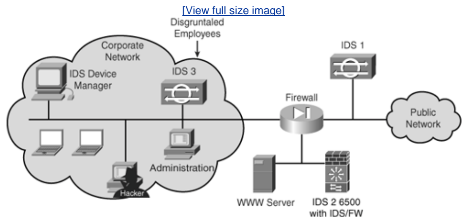
Figure 5-2. IDS Placement
