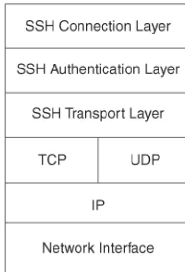
Figure 2-9. SSH Protocol Layers
