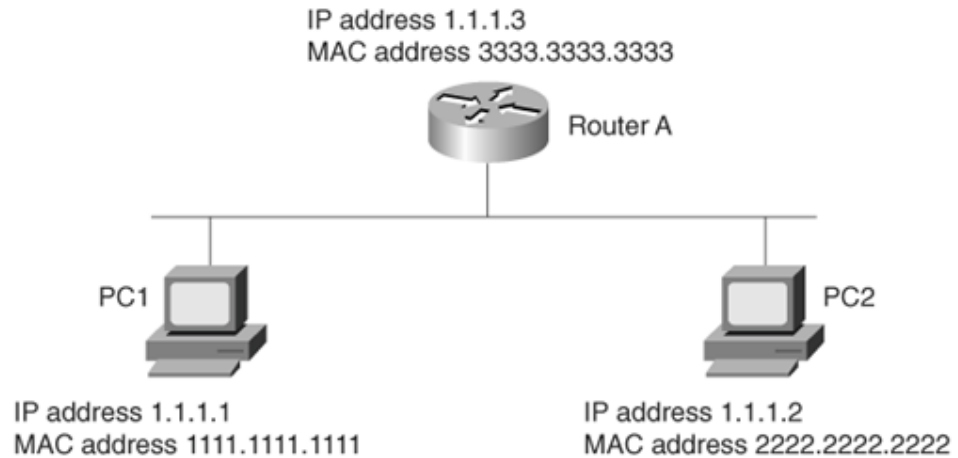
Figure 1-11. ARP Request
