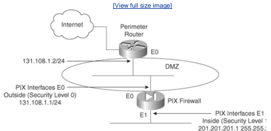
Figure 6-5. Typical PIX Firewall Logical Setup
