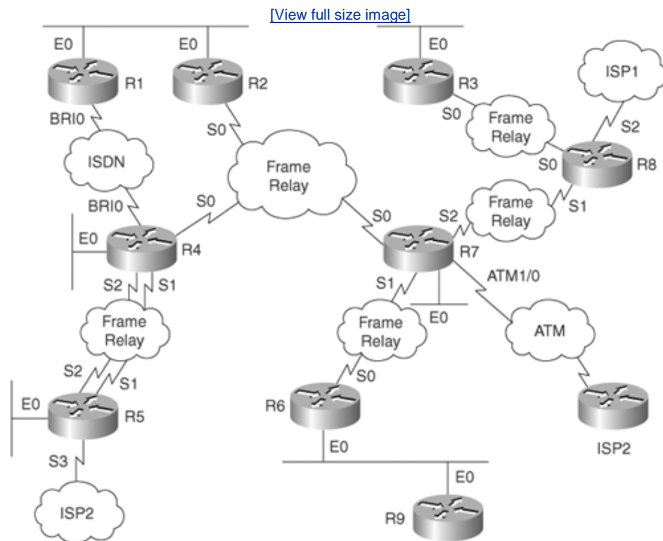
Figure C-1. CCIE Lab Topology
