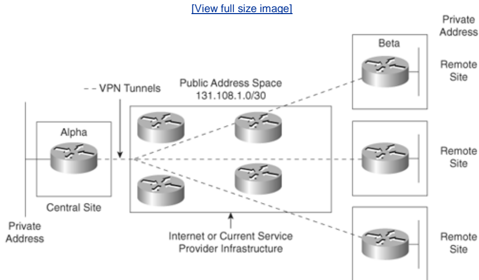
Figure 6-6. VPN Model
