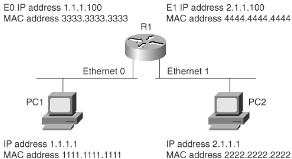
Figure 1-21. Scenario Diagram
