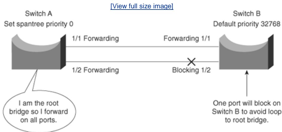
Figure 1-4. Spanning Tree Loop Avoidance
