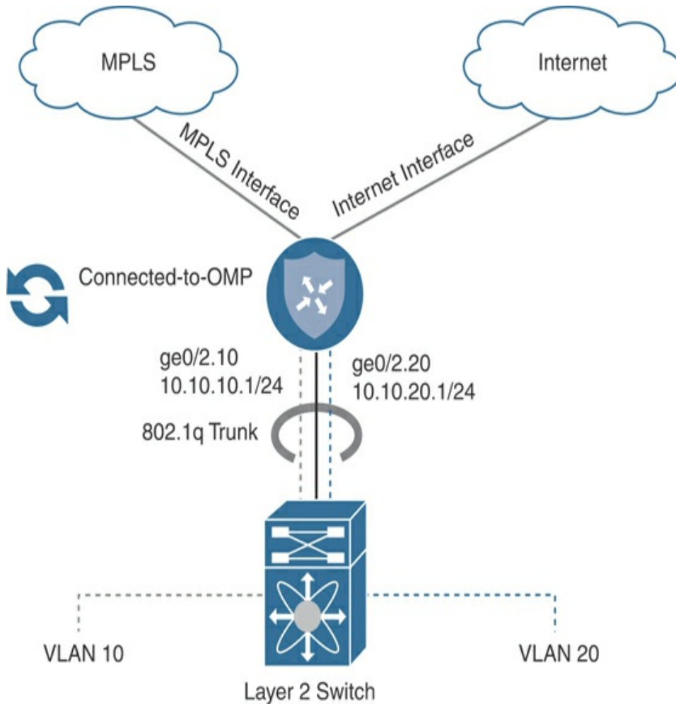
Figure 12-9 Complete CE Replacement—Single Router L2 Branch
