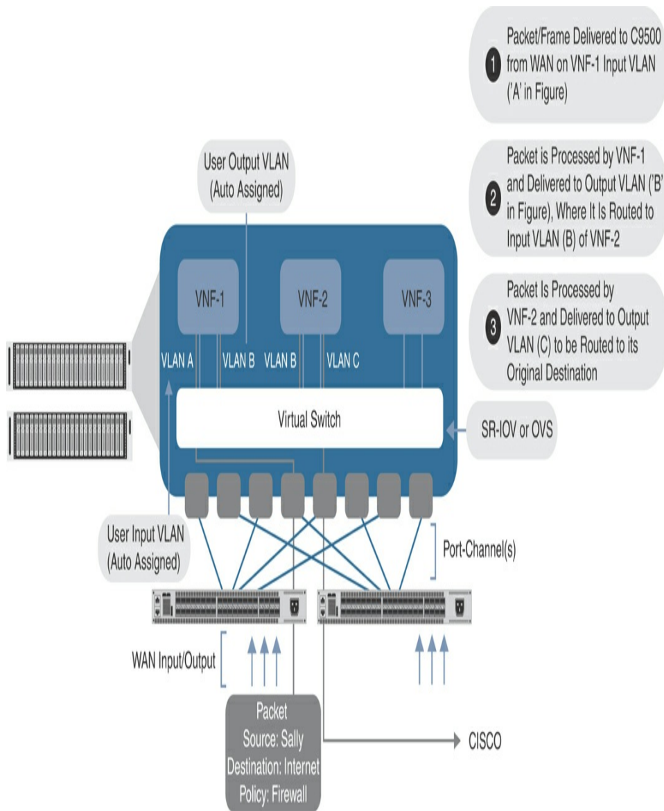
Figure 11-53 Detailed Packet Walkthrough
