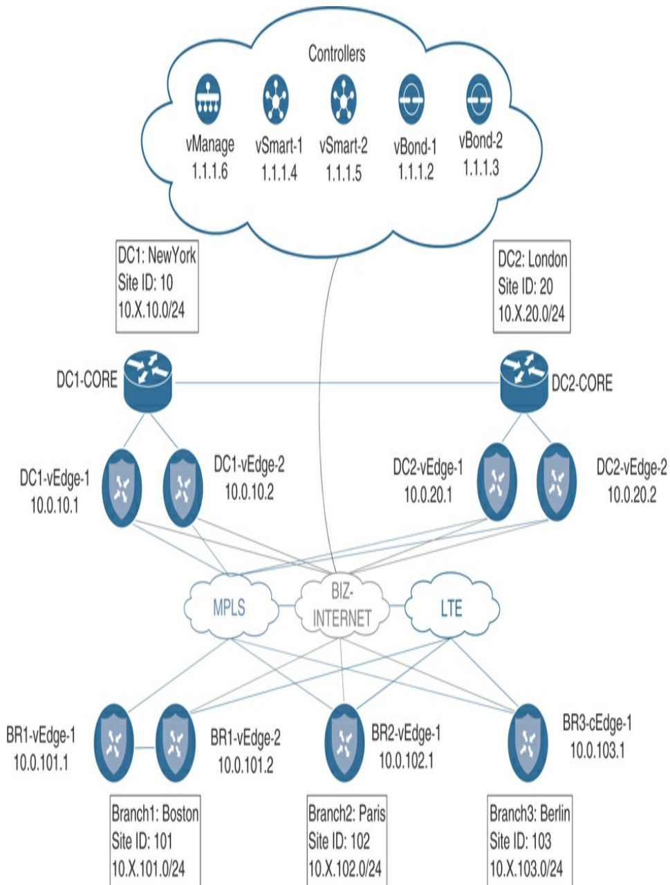
Figure 6-1 Network Topology Overview
