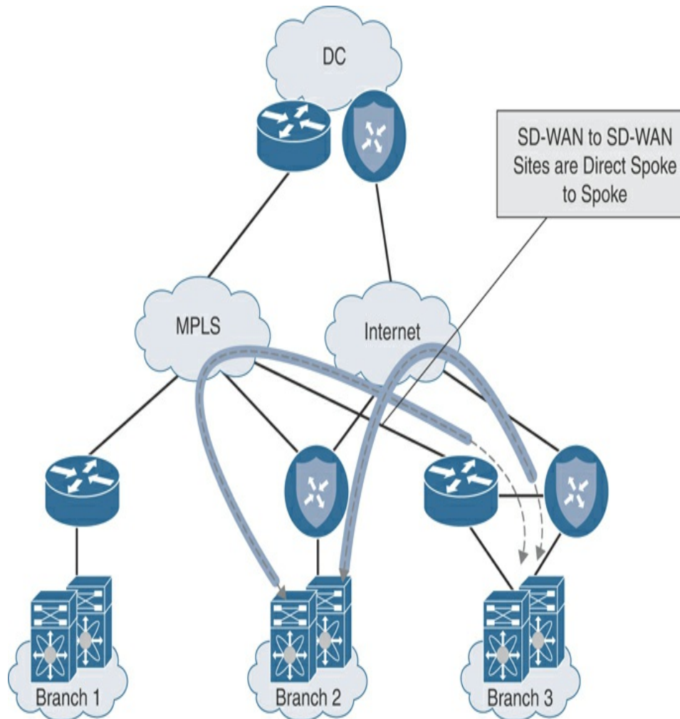
Figure 12-33 Full Overlay with Underlay Routing Cisco SD-WAN Site to Cisco SD-WAN Site Traffic Flow
