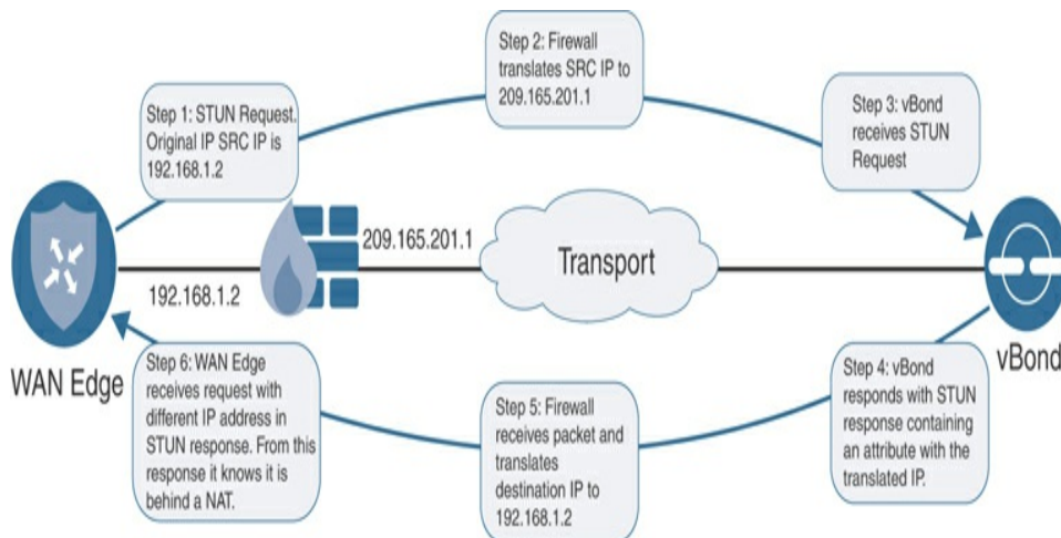
Figure 2-9 STUN NAT Detection Method
