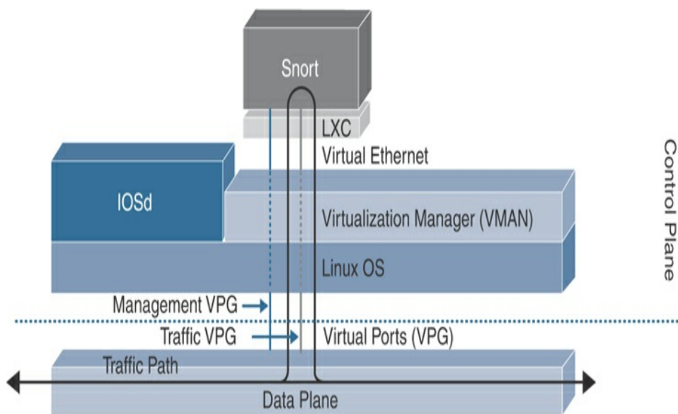
Figure 10-19 Snort Traffic Engine
