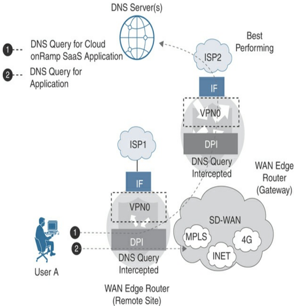
Figure 11-10 Cloud onRamp for SaaS DNS Interception
