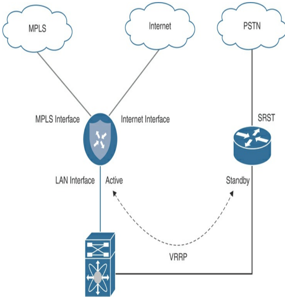
Figure 12-21 Voice Services Integration—L2
