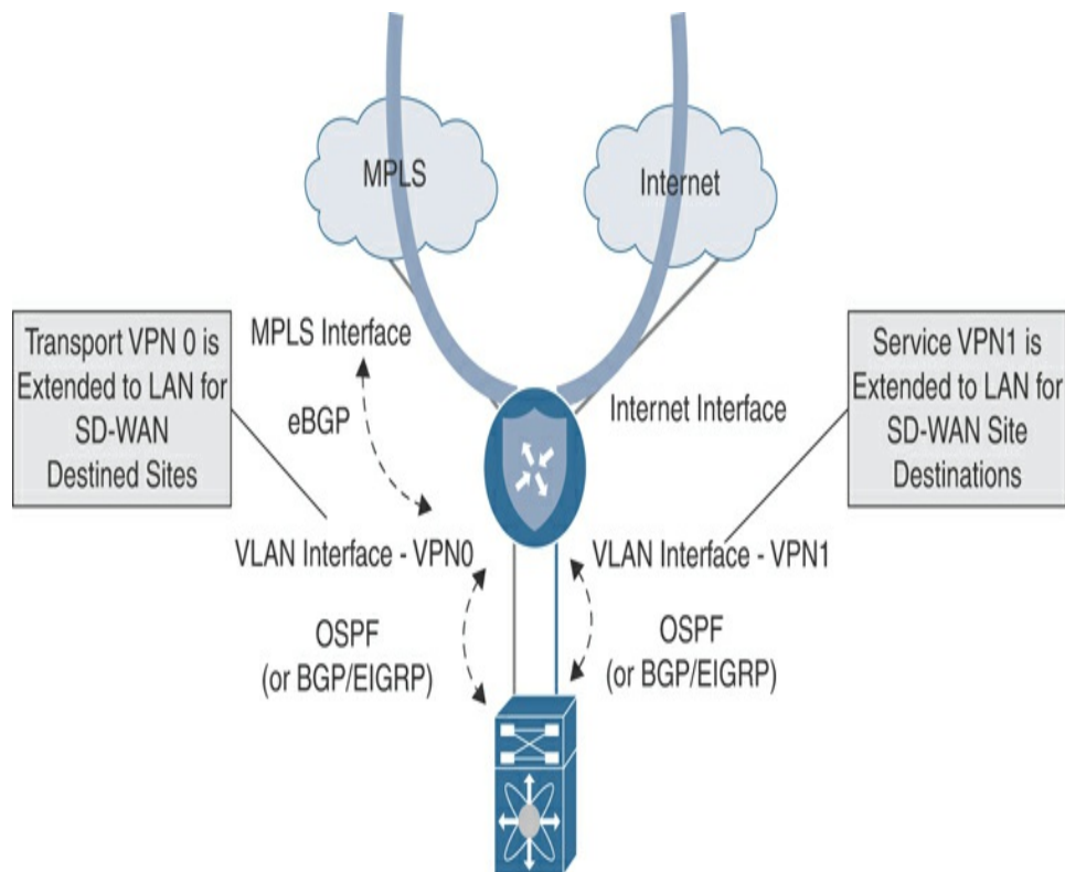
Figure 12-36 Full Overlay with Underlay Routing Without CE Integration
