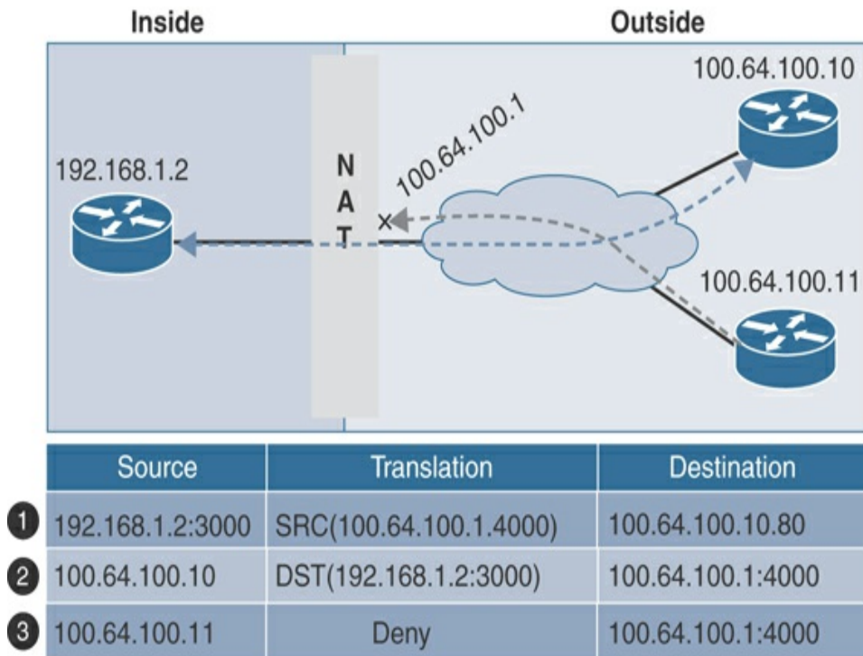
Figure 3-21 Address Restricted Cone NAT
