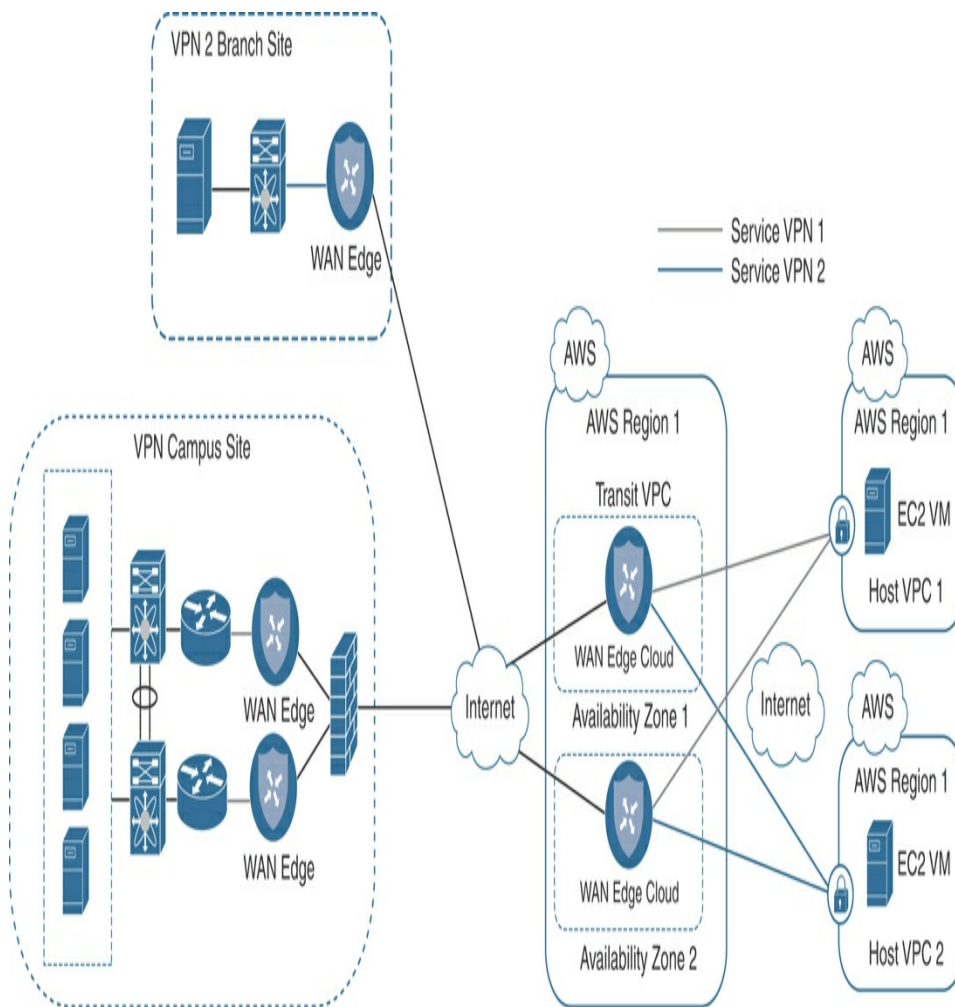
Figure 11-30 Cloud onRamp for IaaS Multi Segment
