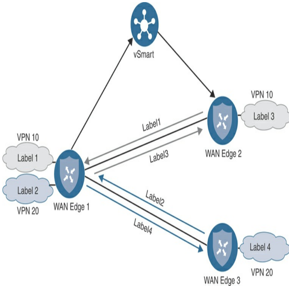
Figure 3-27 Overlay Label Switching
