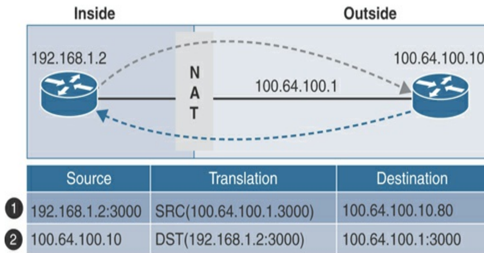
Figure 3-19 Full Cone NAT
