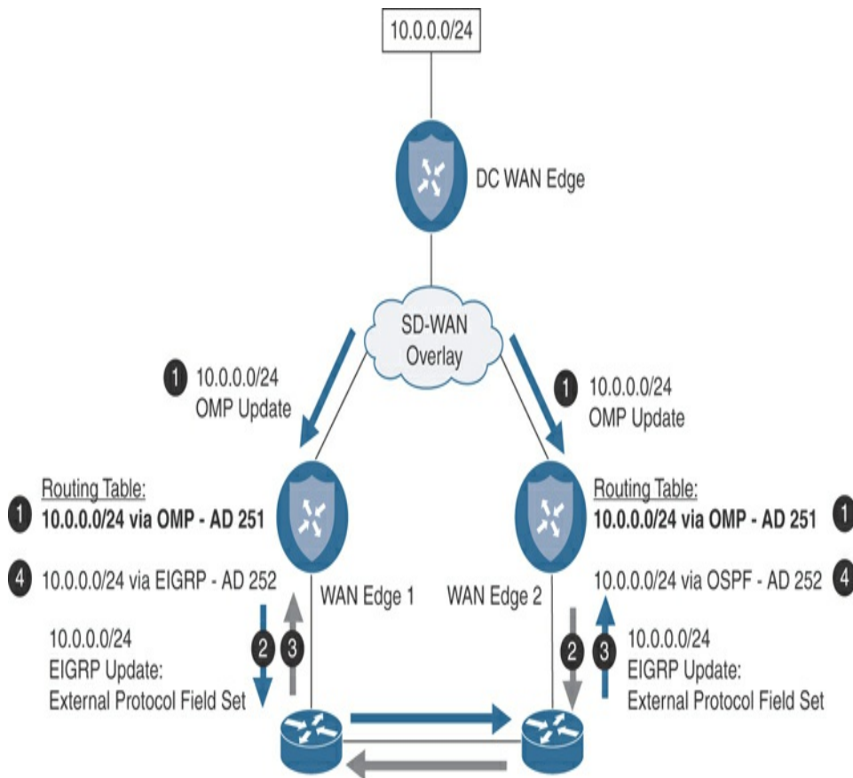
Figure 3-13 EIGRP Loop Prevention with External Protocol Field
