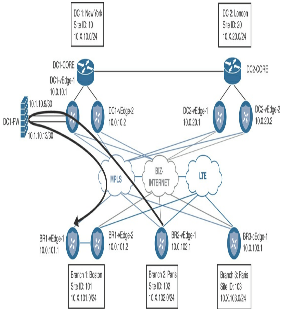
Figure 6-59 Using a Firewall at the Data Center to Inspect Flows Transiting Between Two Branch Sites
