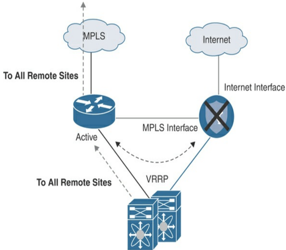
Figure 12-27 Overlay with Underlay Backup—L2 Design Traffic Flow During Failover
