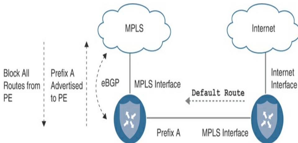
Figure 12-15 TLOC Extension Private
