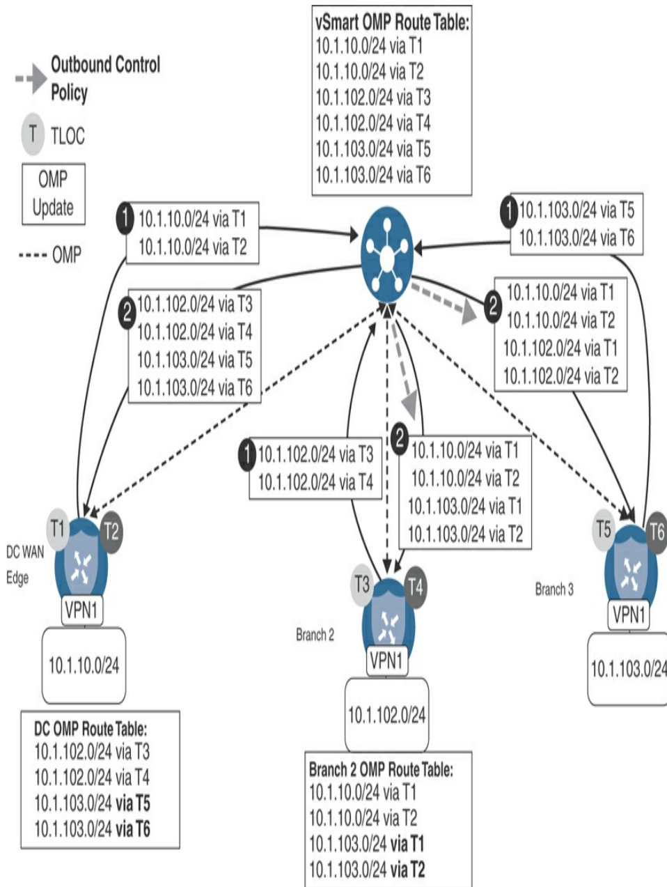
Figure 6-21 Enabling Branch-to-Branch Communication with TLOC Manipulation
