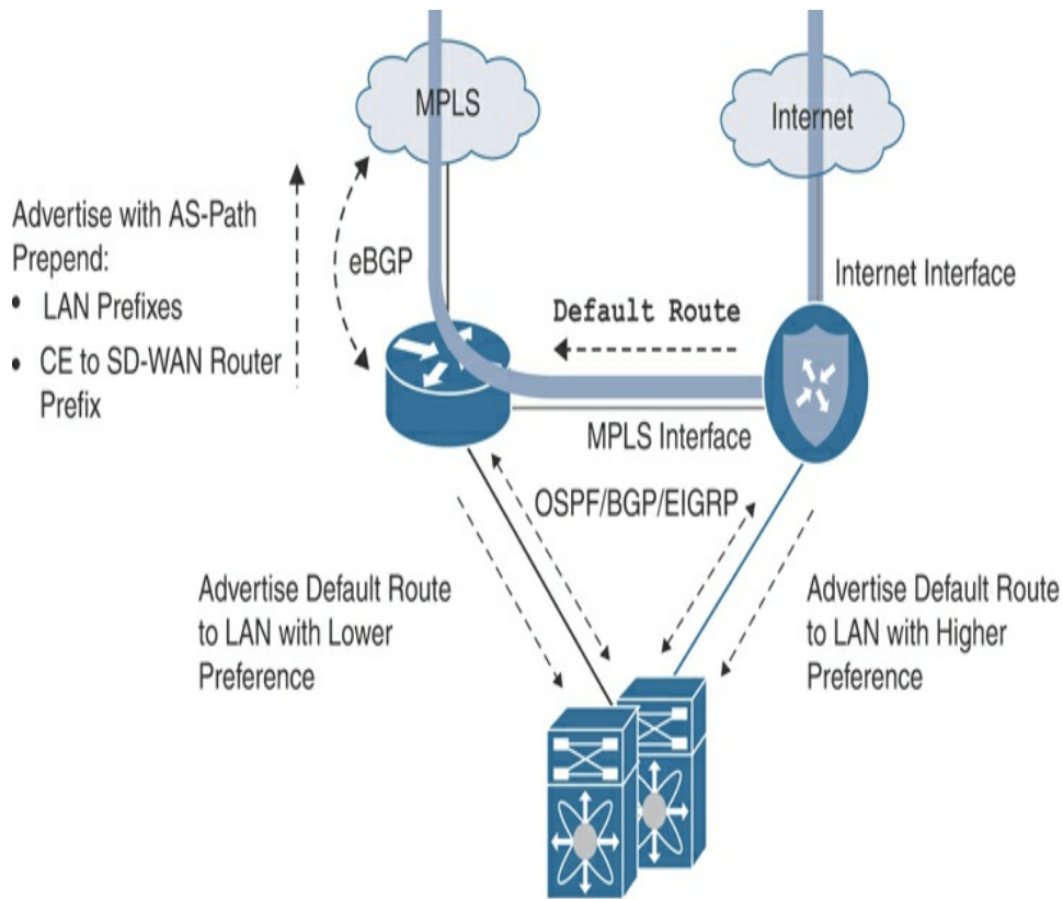
Figure 12-28 Overlay with Underlay Backup—L3 Design
