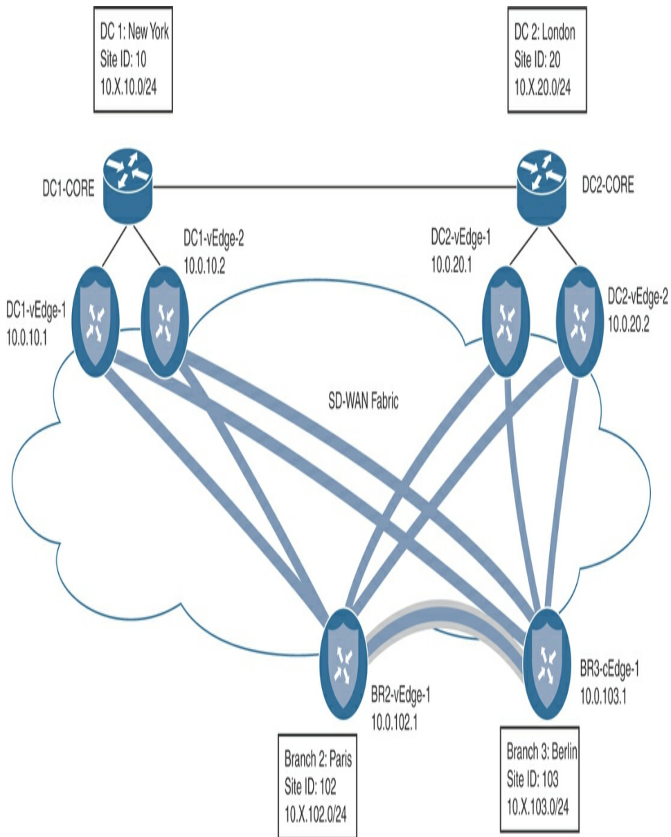
Figure 6-56 Network Topology with Regional Meshes
