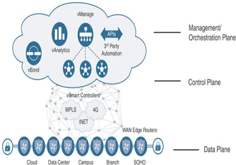
Figure 2-1 Cisco SD-WAN Distributed Architecture
