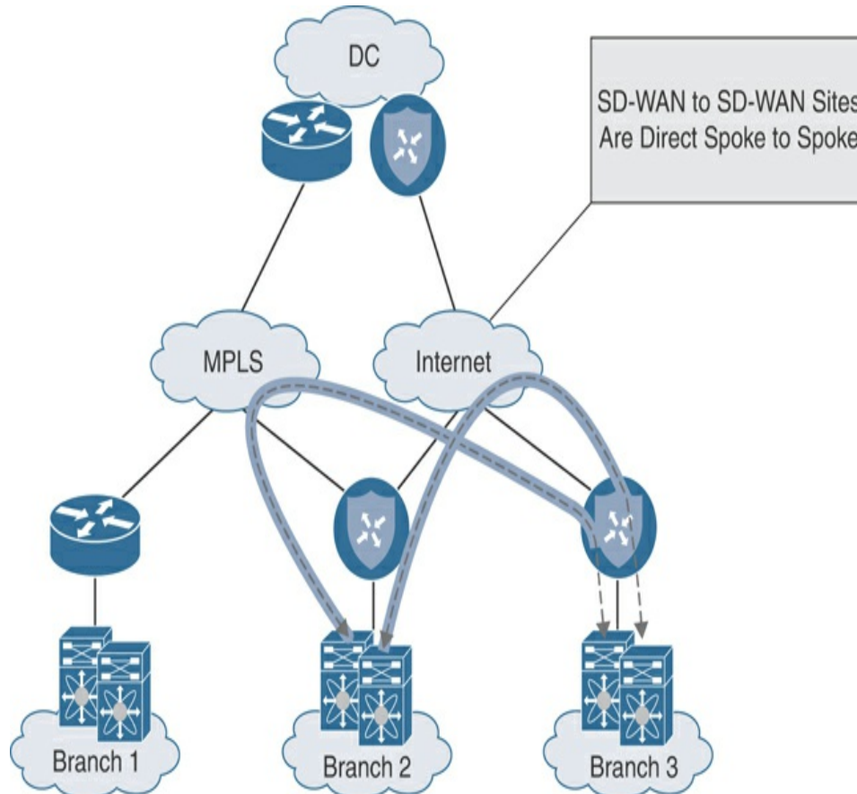
Figure 12-24 SD-WAN to SD-WAN Site Overlay-Only Traffic Flow
