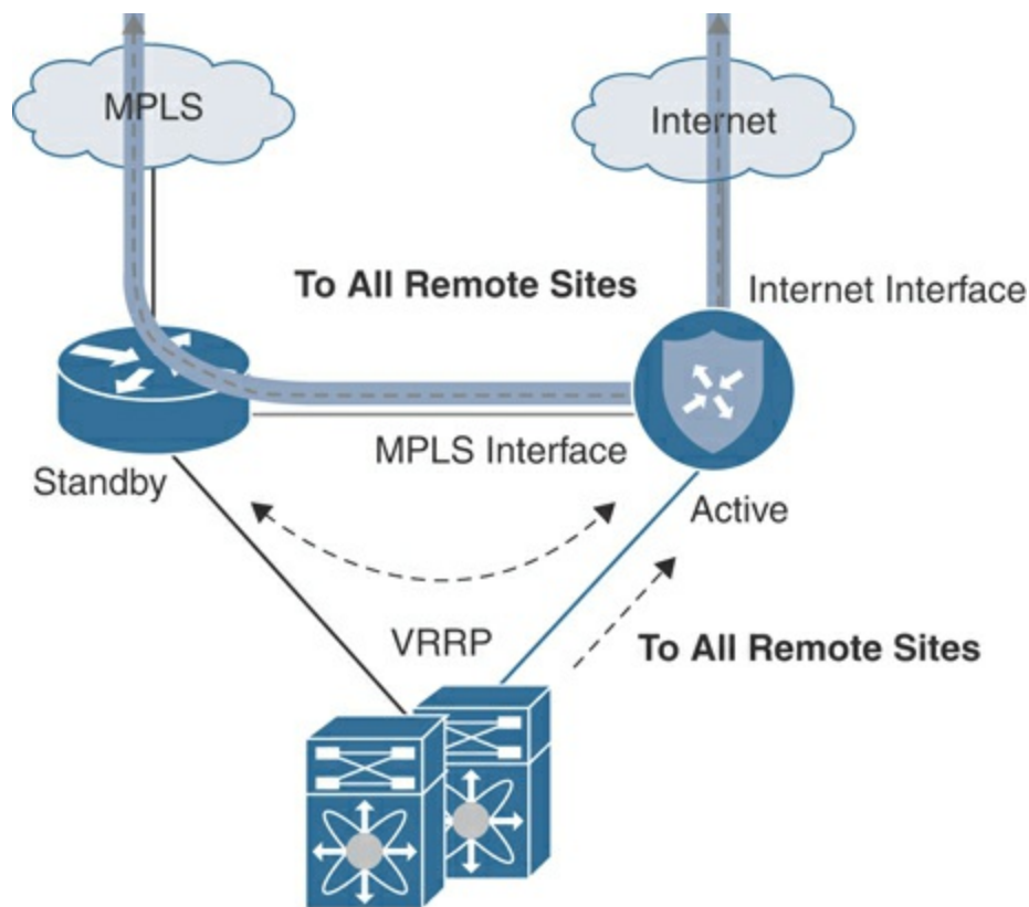
Figure 12-26 Overlay with Underlay Backup—L2 Design Traffic Flow
