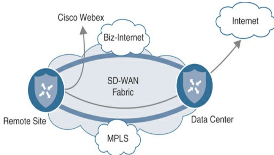
Figure 7-14 Desired Forwarding Paths Are Different per Application
