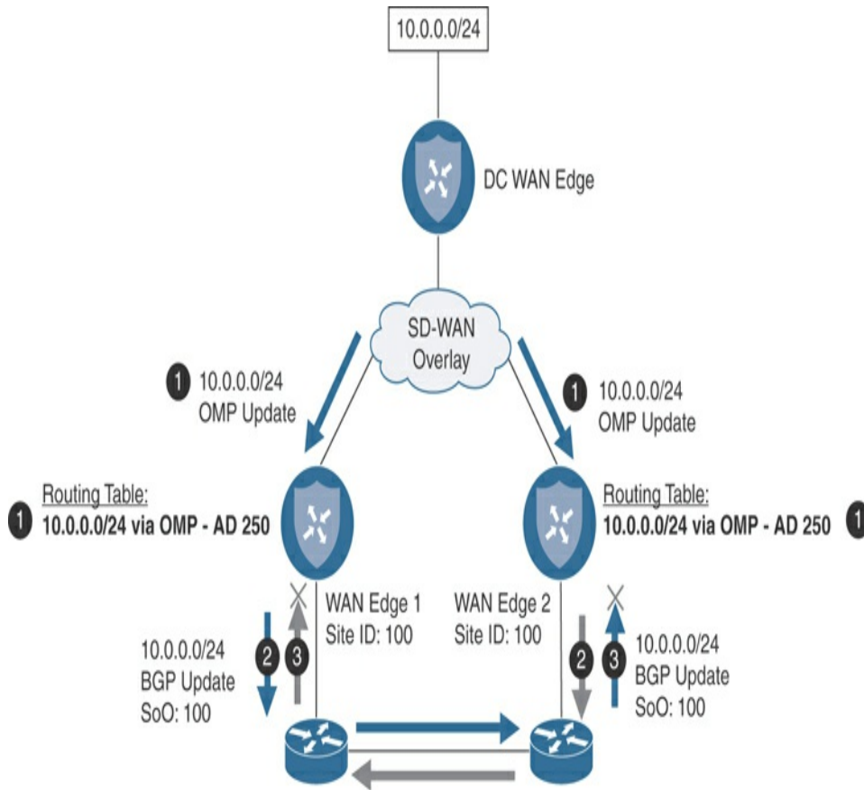
Figure 3-12 BGP Loop Prevention with Site of Origin
