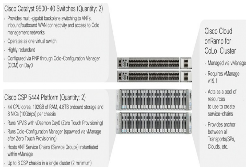
Figure 11-51 Cloud onRamp for Colocation Cluster
