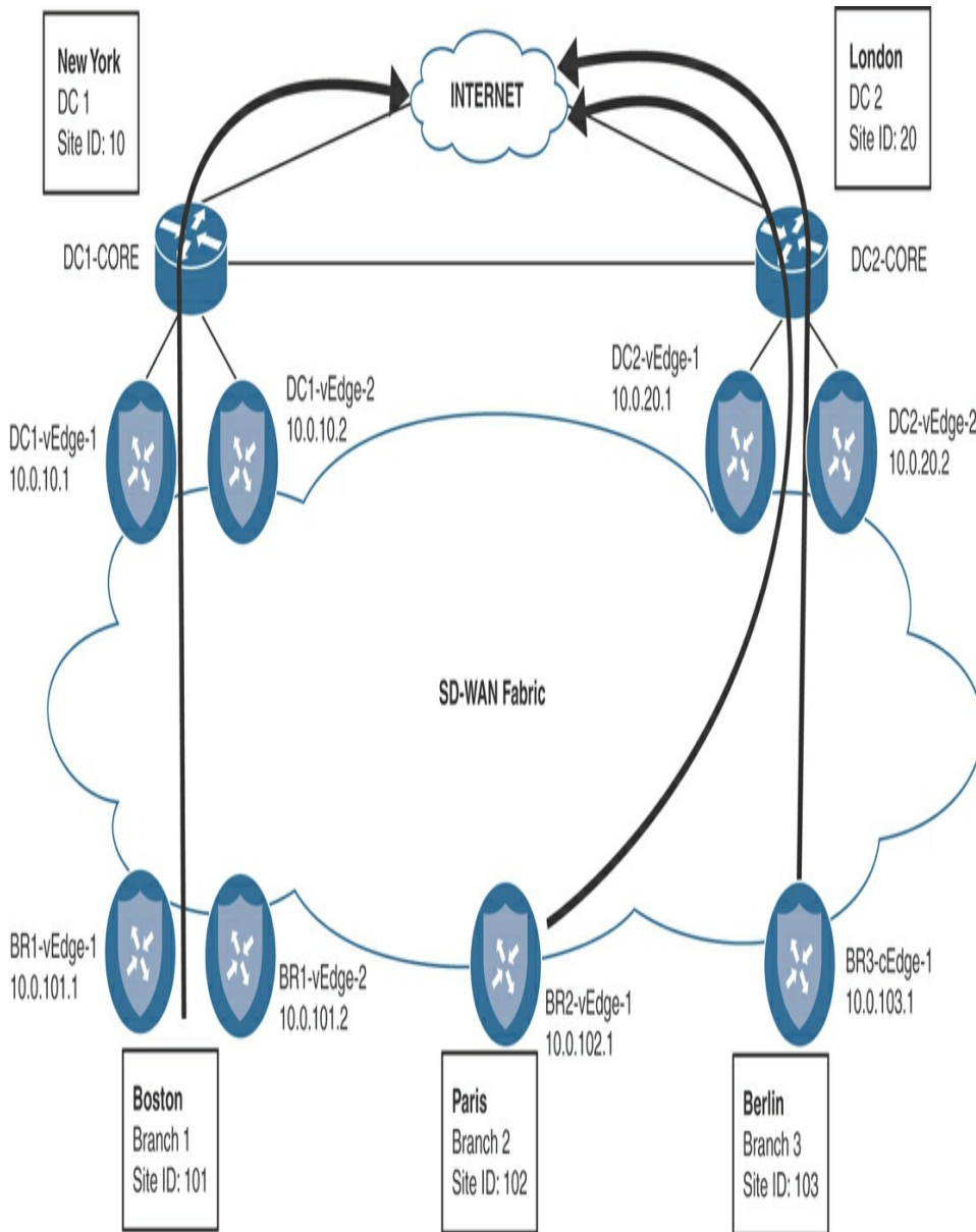
Figure 6-50 Regionalizing Access to a Service, such as Internet Egress
