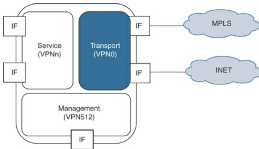
Figure 3-26 VPN Types
