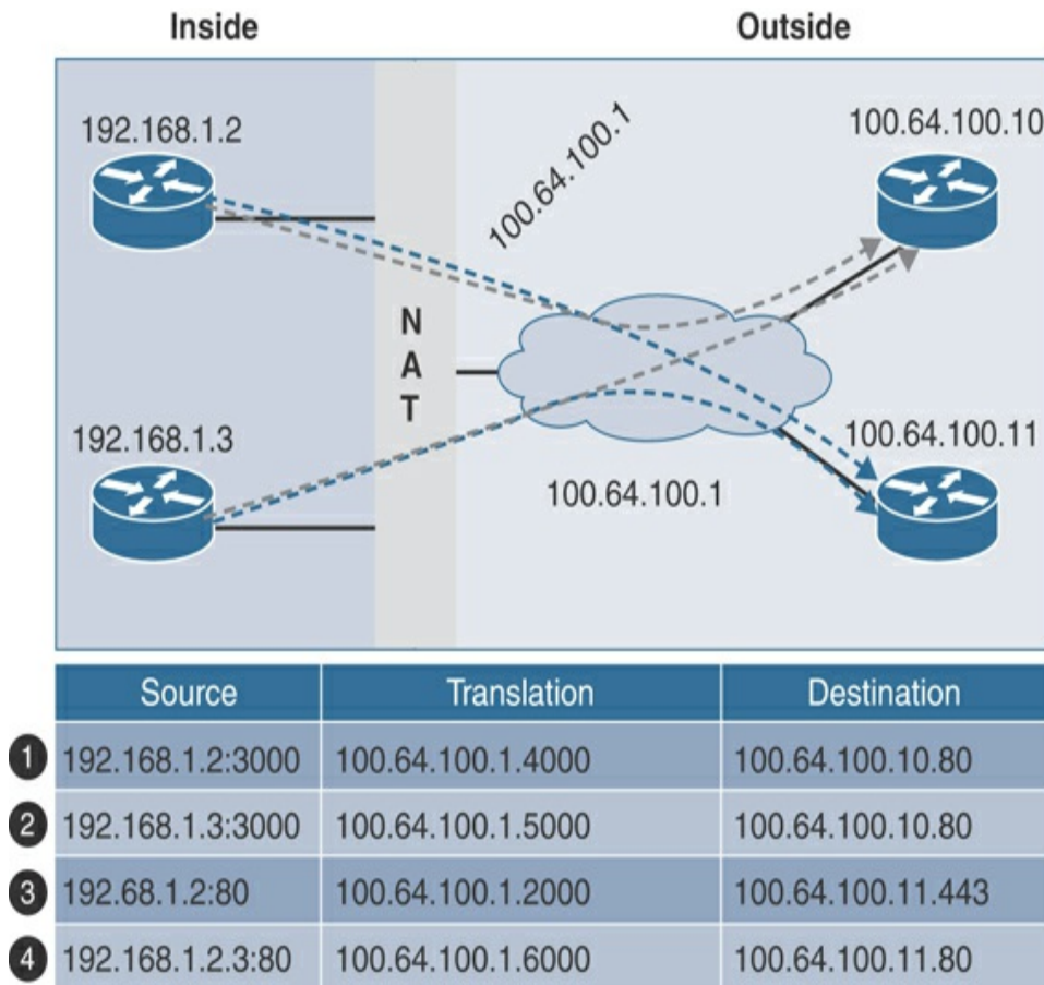
Figure 3-20 Symmetric NAT
