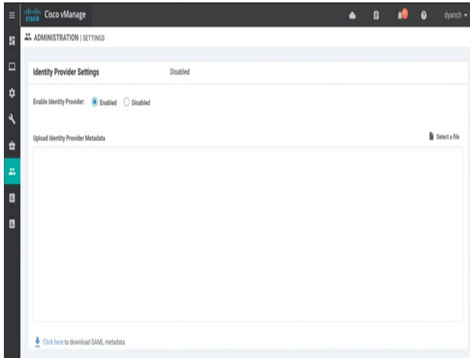
Figure 10-47 SSO Configuration
