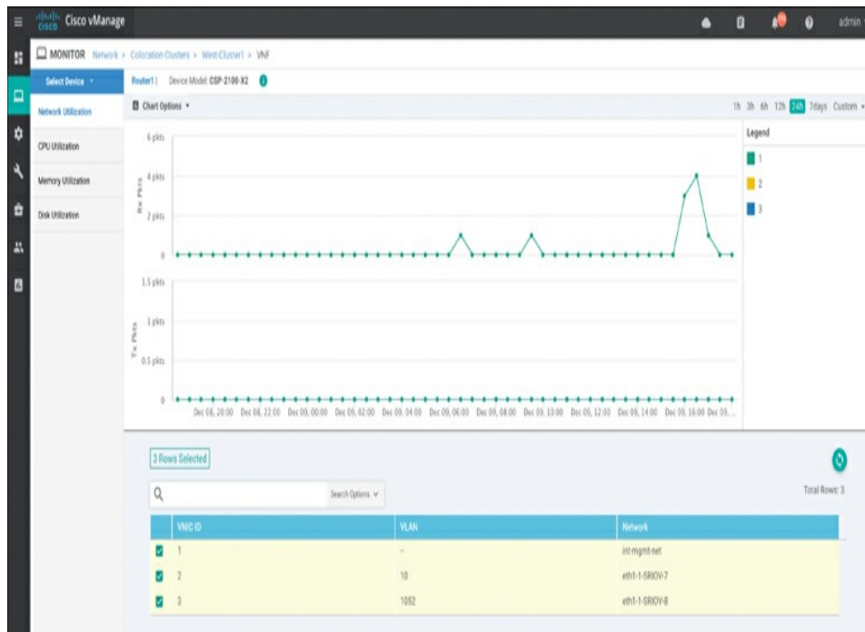
Figure 11-76 VNF Health
