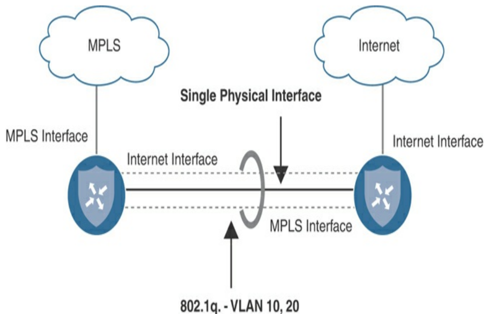
Figure 12-14 TLOC Extension Sub-Interfaces
