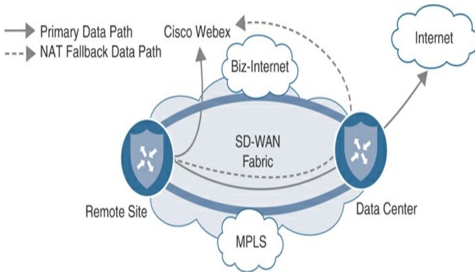
Figure 7-20 Illustrated NAT Fallback Data Path
