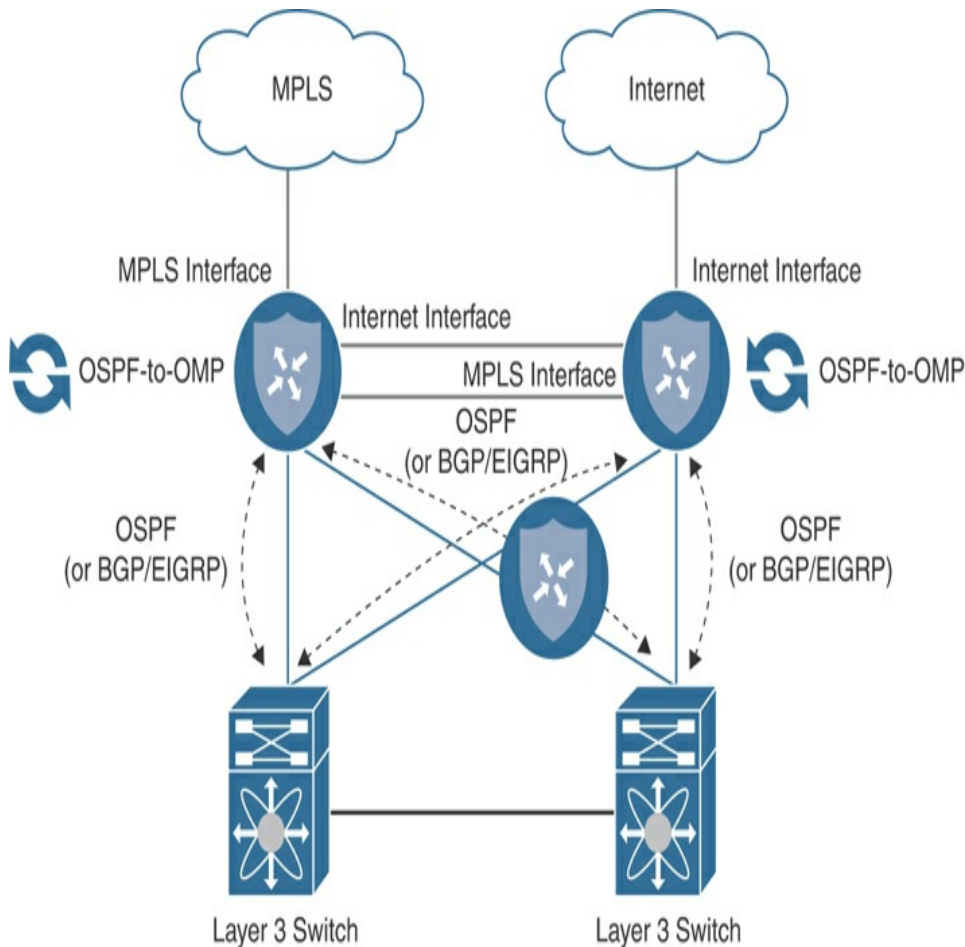
Figure 12-12 Complete CE Replacement—Dual Router L3 Branch
