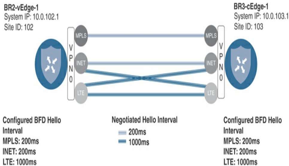
Figure 8-13 BFD Hello Interval Negotiation
