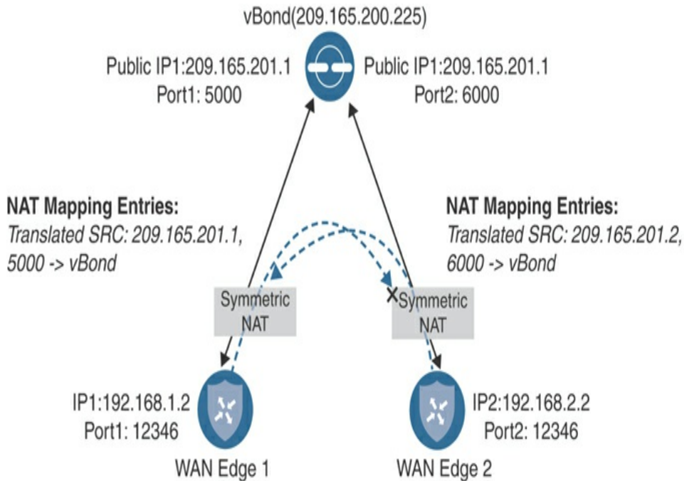
Figure 3-24 Symmetric NAT Restrictions
