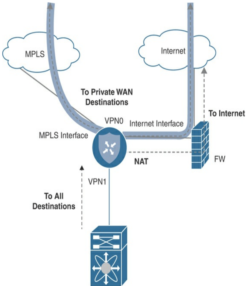
Figure 12-20 Transport and DIA Through Firewall Single Link
