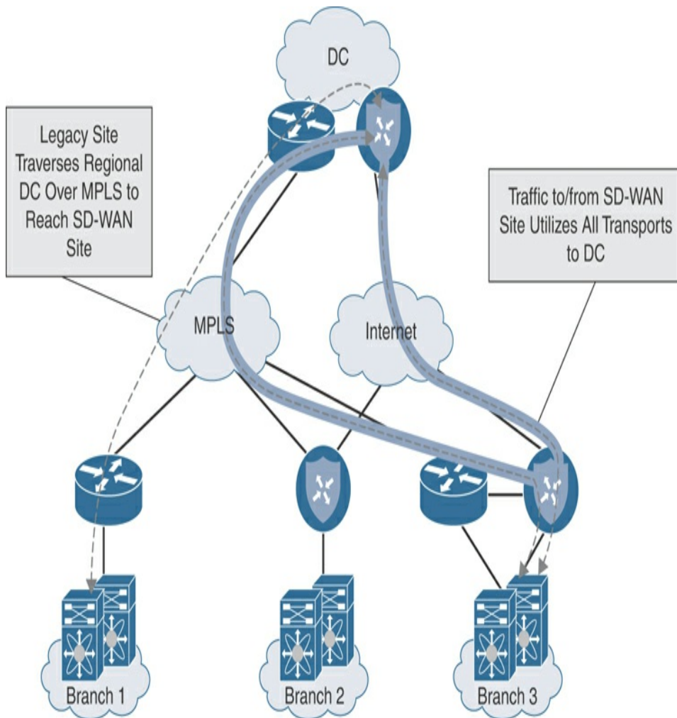
Figure 12-30 Overlay with Underlay Backup Traffic Flow
