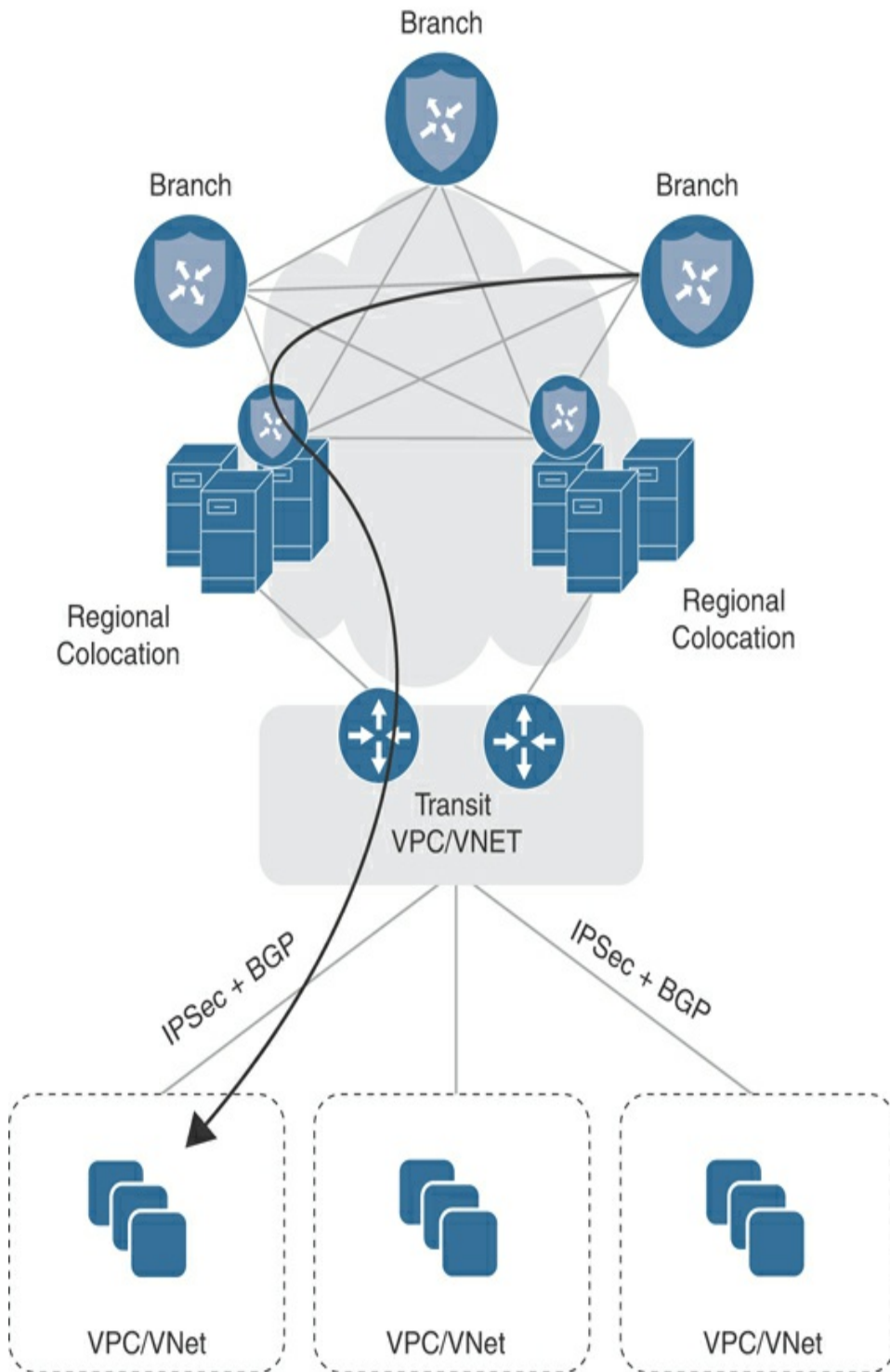
Figure 11-54 Infrastructure as a Service via Colocation
