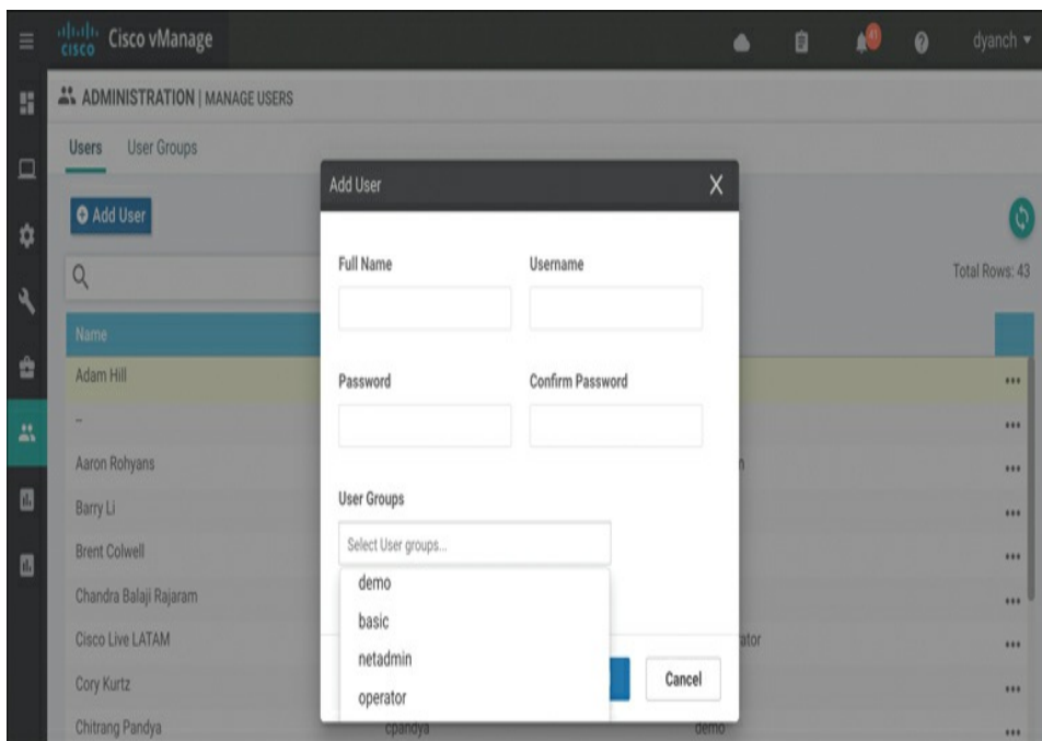
Figure 10-40 Add Users
