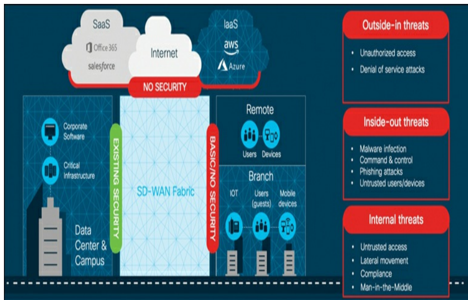
Figure 10-1 Threat Surface
