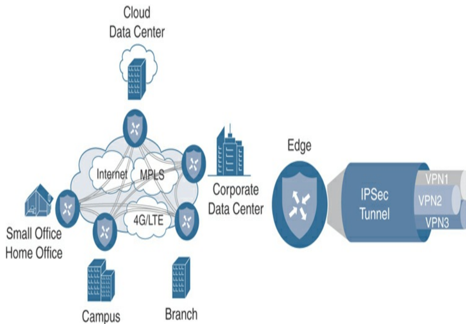
Figure 1-10 End-to-End Segmentation
