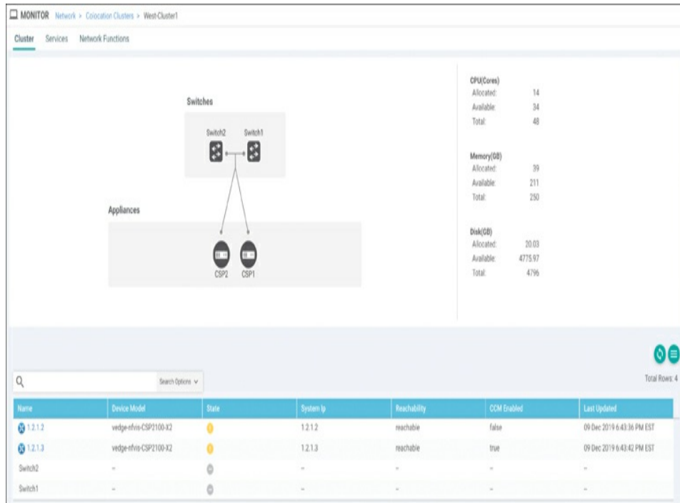
Figure 11-73 Colocation Cluster
