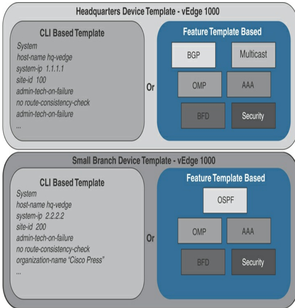
Figure 4-1 Device Templates
