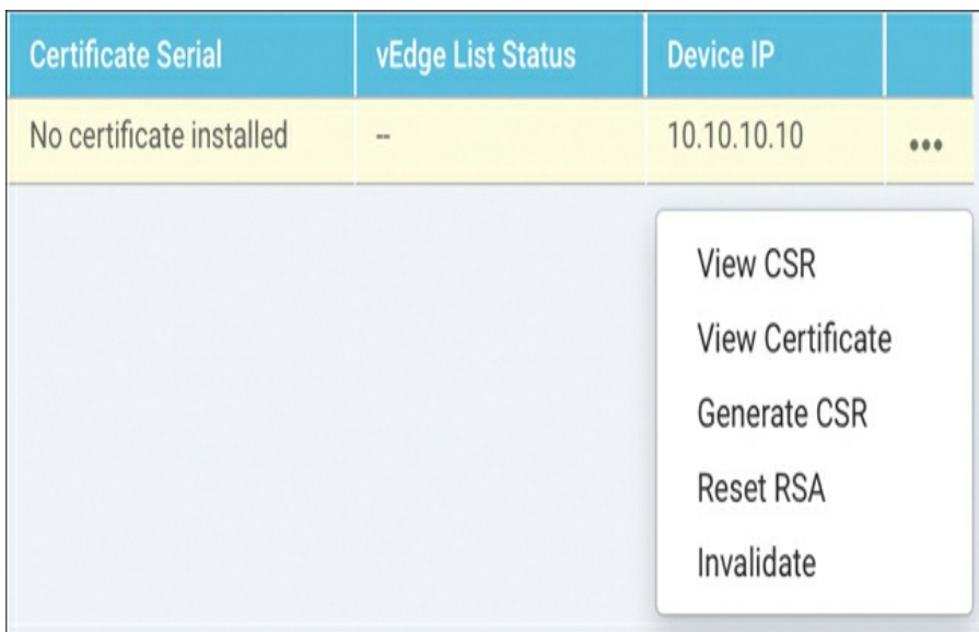
Figure 13-19 Download CSR
