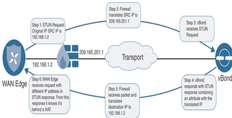
Figure 3-23 NAT Traversal with STUN
