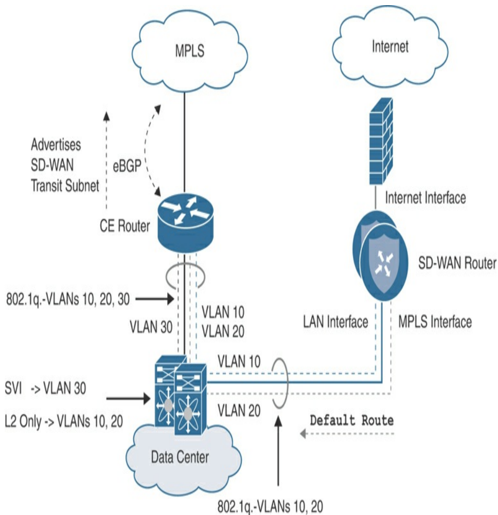
Figure 12-3 Data Center Indirect Transport Side
