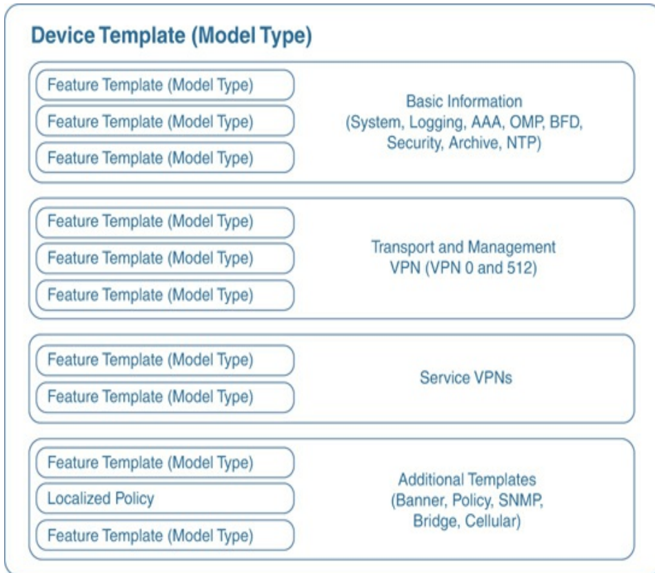
Figure 4-2 Device Template Structure
