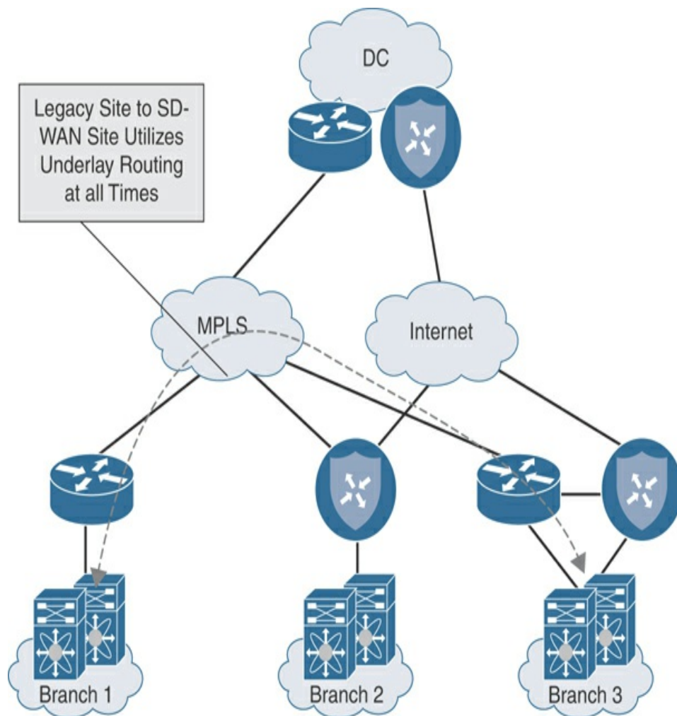
Figure 12-32 Full Overlay with Underlay Routing
