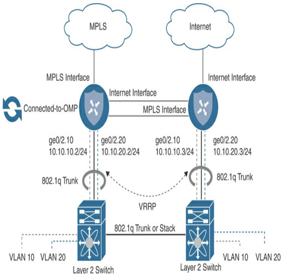
Figure 12-11 Complete CE Replacement—Dual
