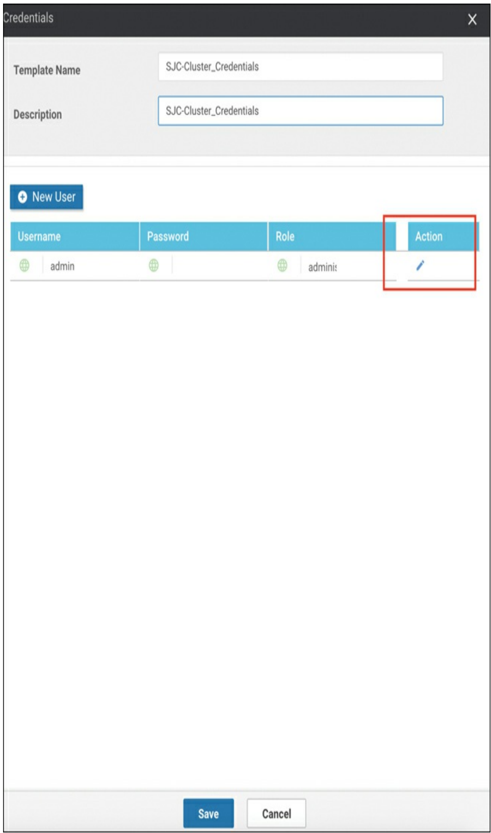
Figure 11-61 Cluster Credentials
