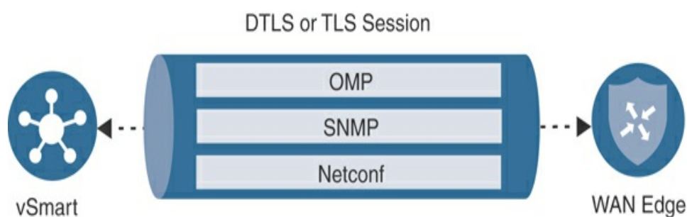
Figure 3-4 Protocol Communications
