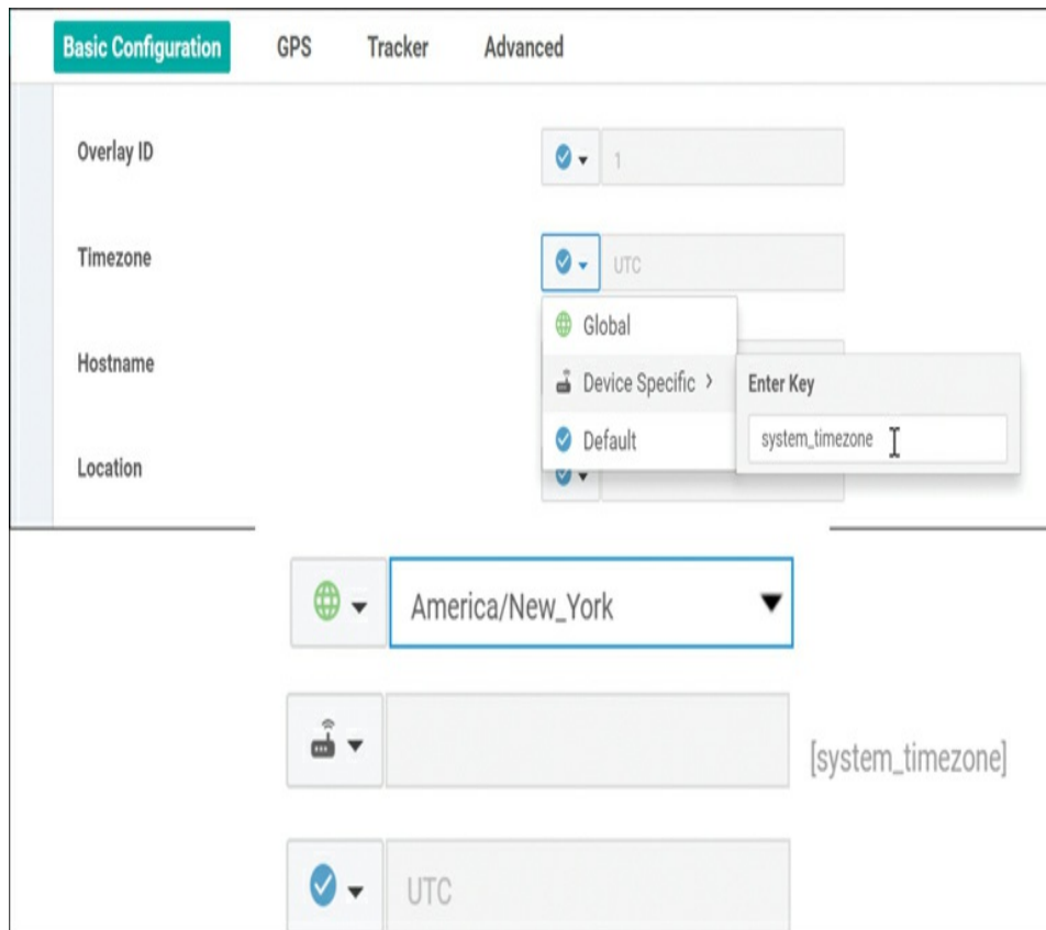
Figure 4-4 Setting Variables
