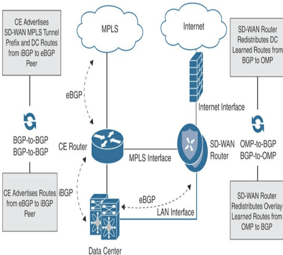
Figure 12-6 Service-Side BGP
