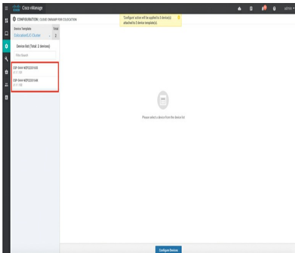
Figure 11-63 Cluster Activation
