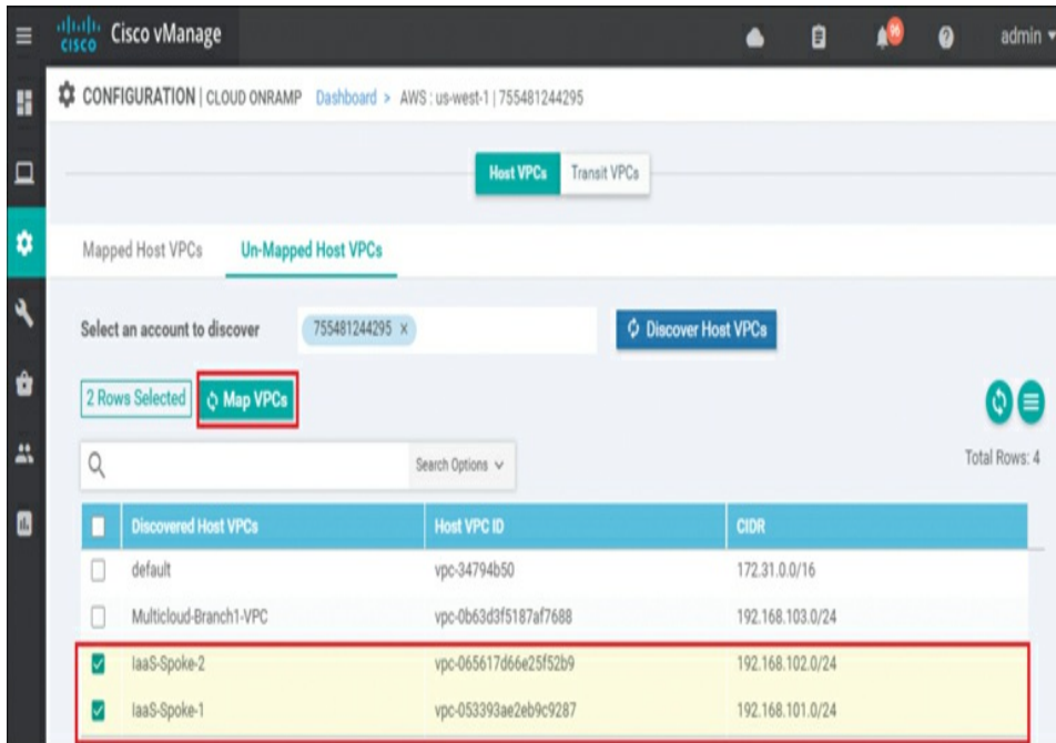
Figure 11-41 Map VPCs
