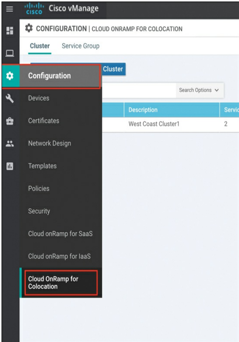
Figure 11-58 vManage Configuration
