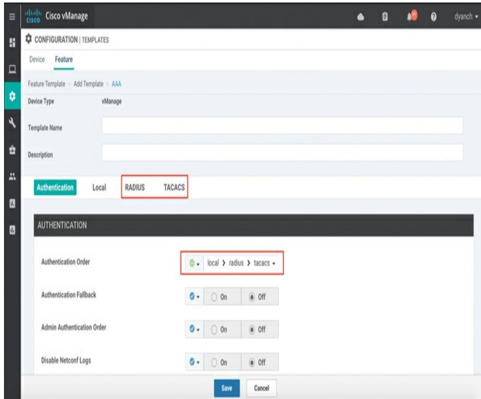
Figure 10-46 RADIUS/TACACS Configuration
