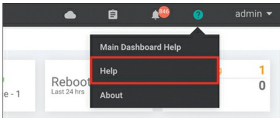
Figure 11-57 vManage Help
