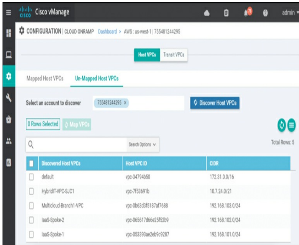
Figure 11-40 Discovered VPCs
