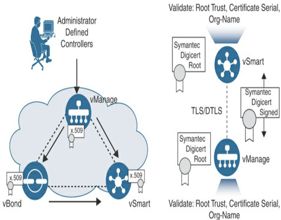
Figure 13-2 Controller-Based Connectivity
