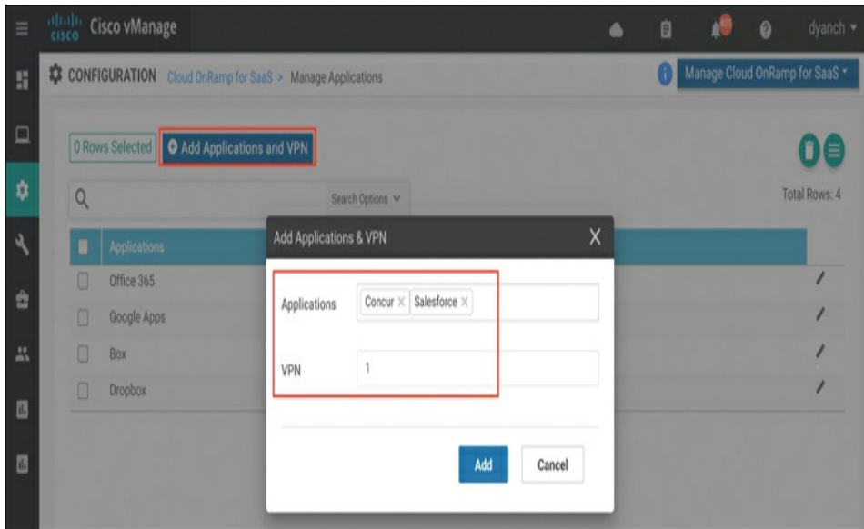
Figure 11-14 Defining Applications
