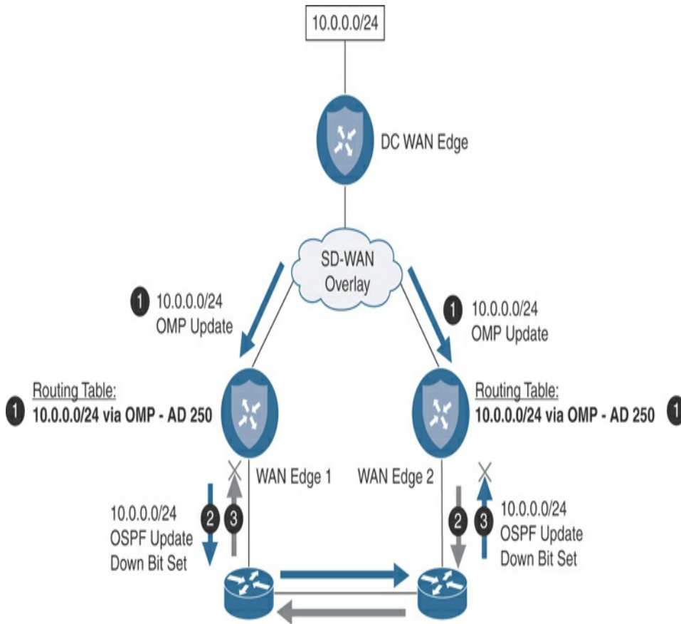
Figure 3-11 OSPF Loop Prevention with Down Bit
