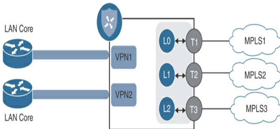
Figure 12-4 Loopback TLOC Bind Mode
