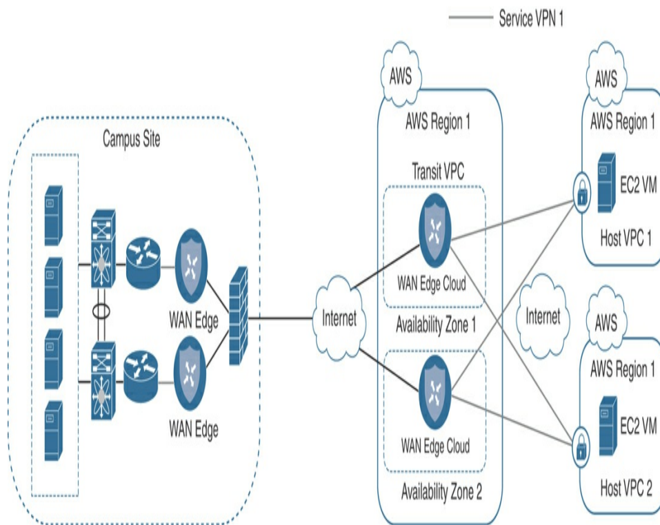
Figure 11-29 Cloud onRamp for IaaS Single Segment
