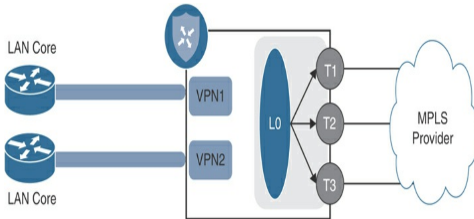
Figure 12-5 Loopback TLOC Standard Mode
