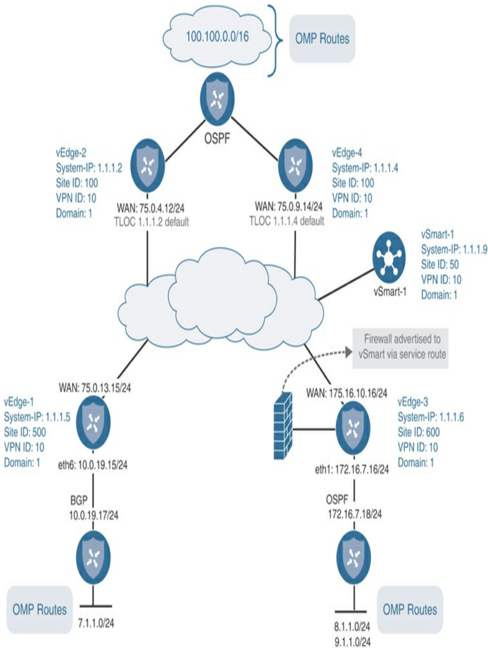
Figure 3-5 Examples of the Three Types of OMP Routes
