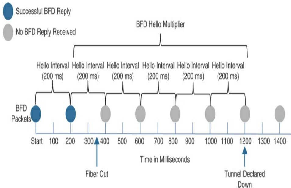
Figure 8-15 BFD Path Liveliness Detection
