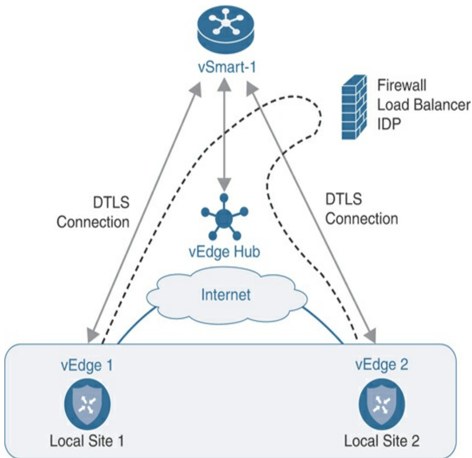
Figure 3-7 Service Chaining Example
