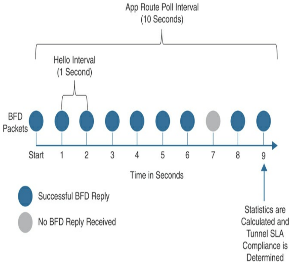
Figure 8-16 App-Route Poll Interval Illustration
