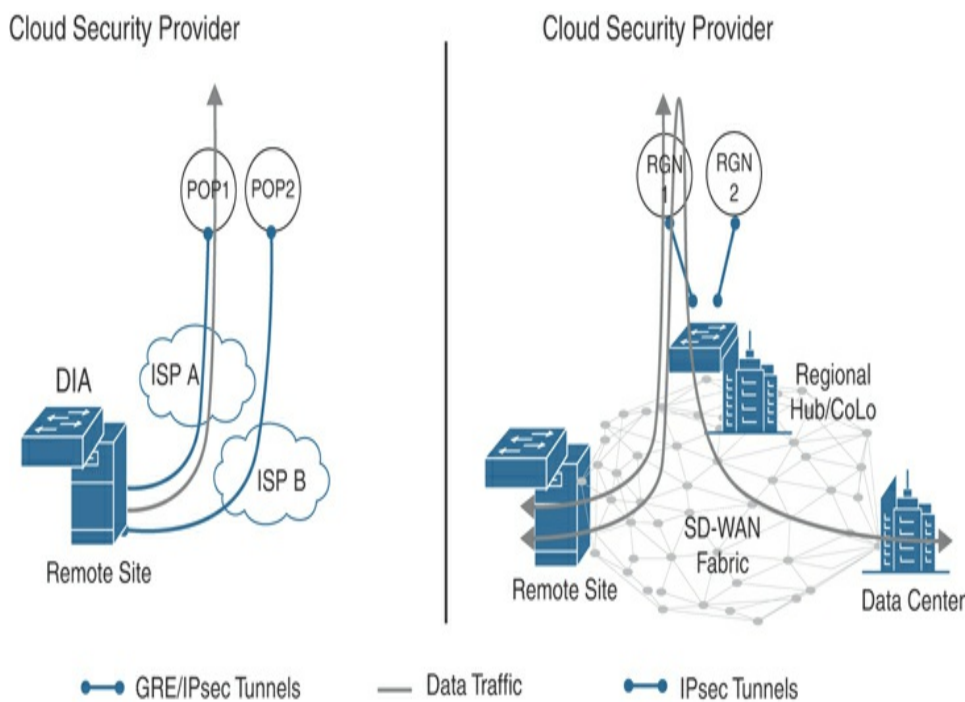
Figure 10-36 Cloud Security Connectivity
