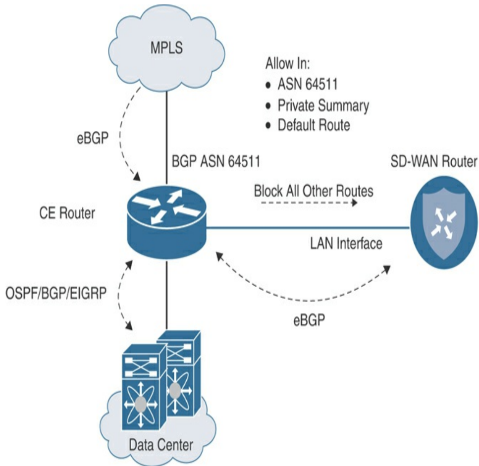
Figure 12-29 Overlay with Underlay Backup—Data Center Considerations
