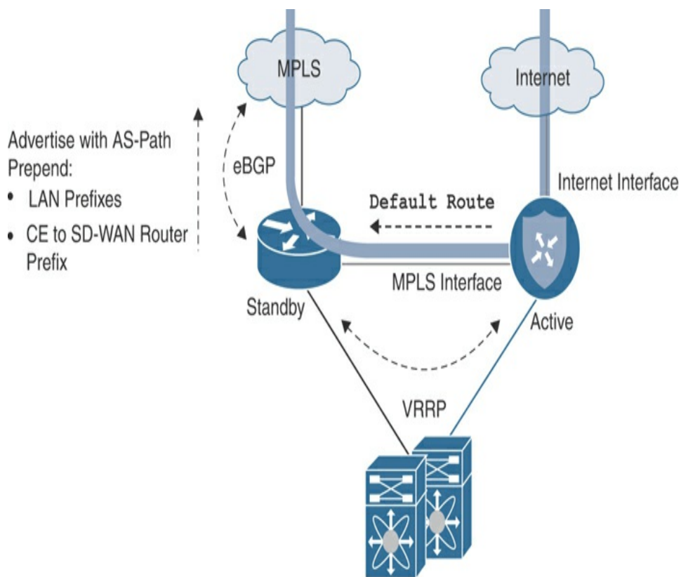
Figure 12-25 Overlay with Underlay Backup—L2 Design
