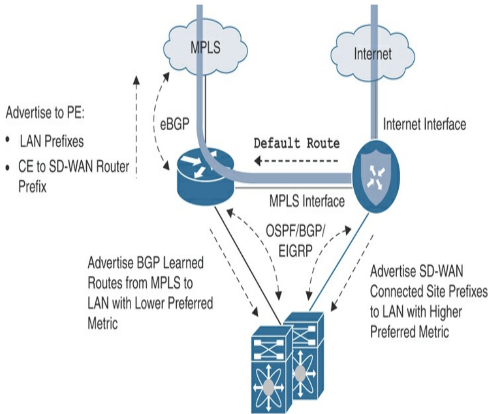
Figure 12-34 Full Overlay with Underlay Routing CE Integration
