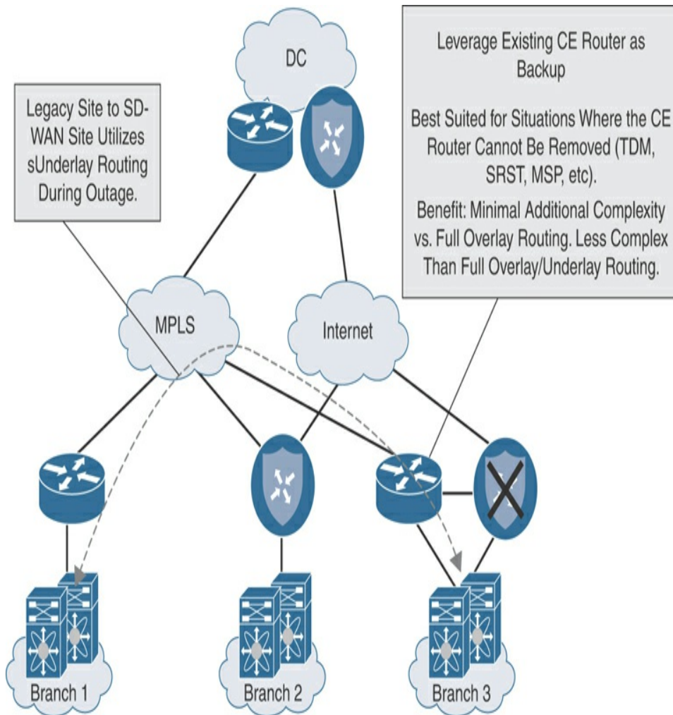
Figure 12-31 Overlay with Underlay Backup Traffic Flow During Failover
