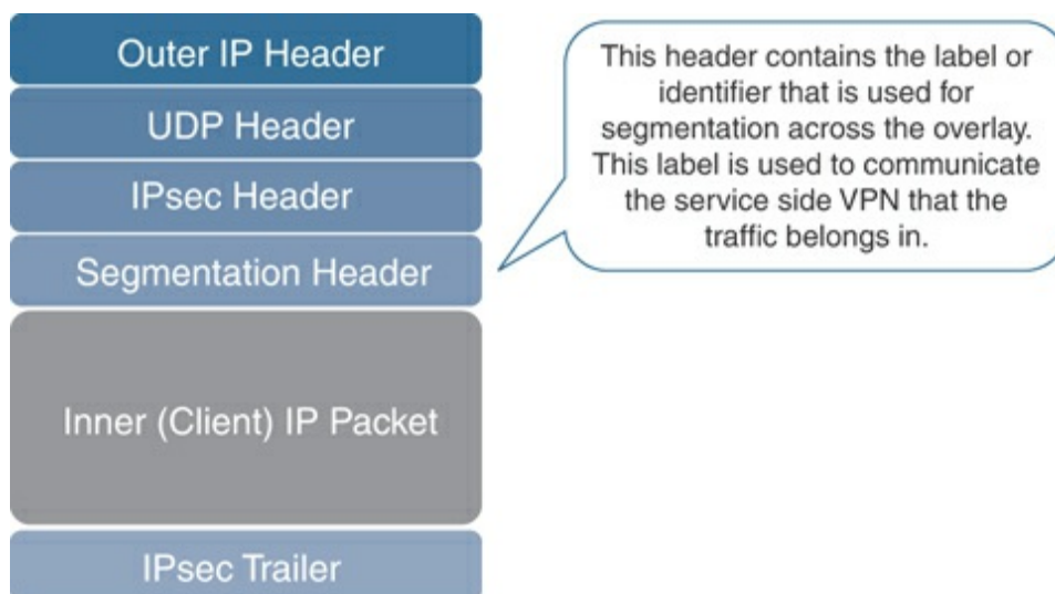
Figure 2-2 Cisco SD-WAN Packet Format
