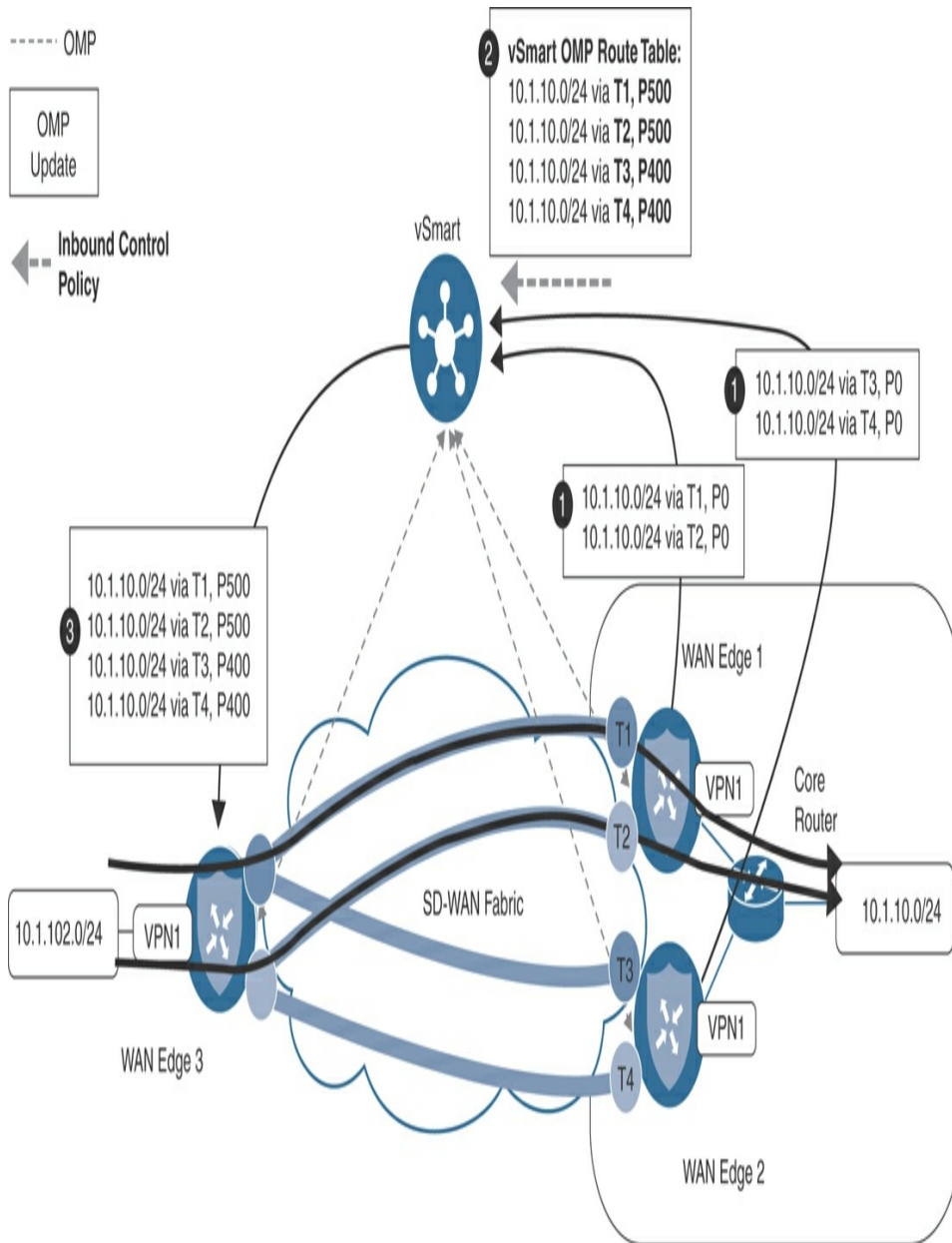
Figure 6-48 Illustration of the Effects of Different Preference Values on the Forwarding Plane
