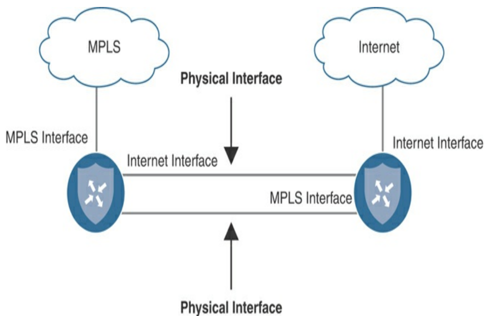
Figure 12-13 TLOC Extension Dedicated Interfaces
