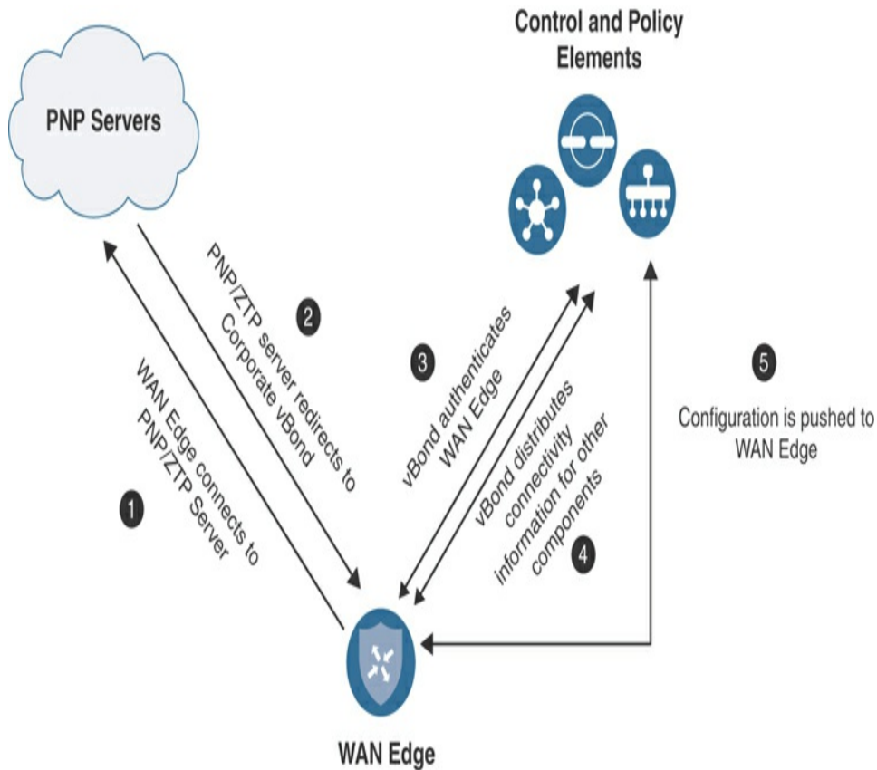
Figure 2-4 High-level Overview of the Plug and Play/Zero Touch Provisioning Process
