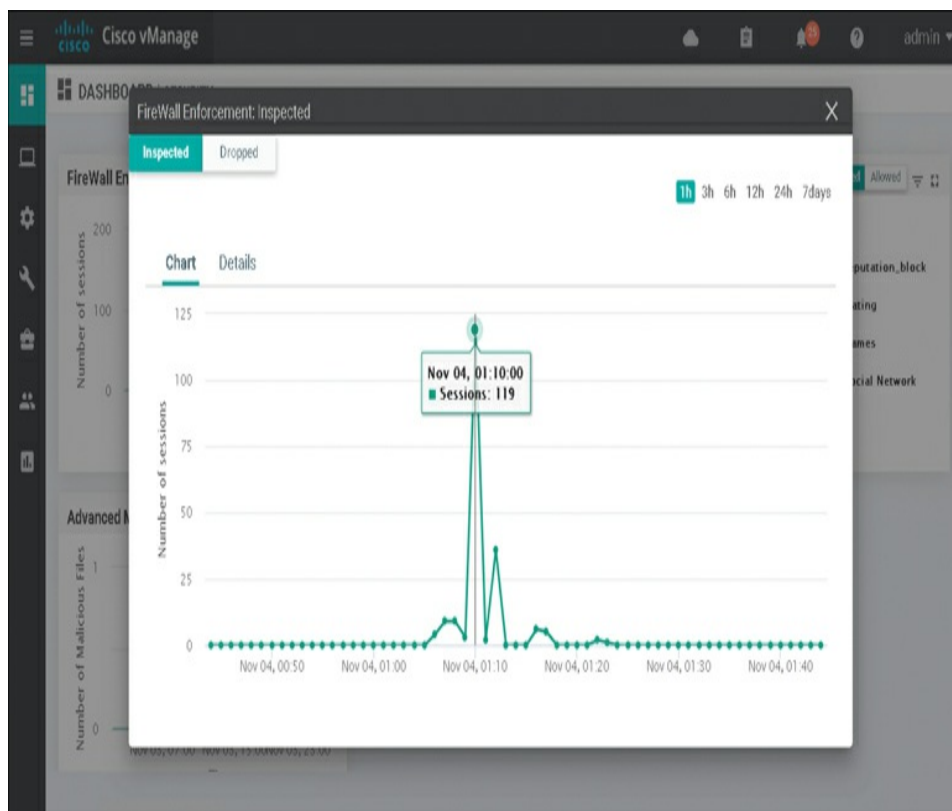
Figure 10-13 Security Dashboard
