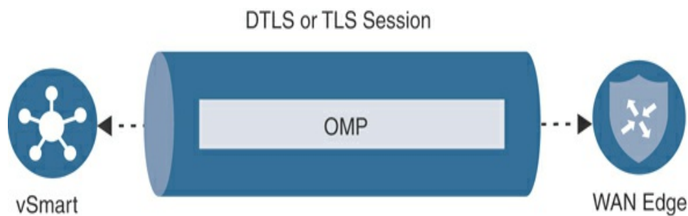
Figure 3-2 DTLS Tunnel
