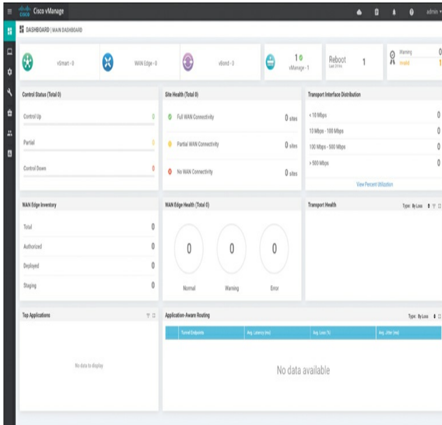
Figure 13-14 vManage Dashboard
