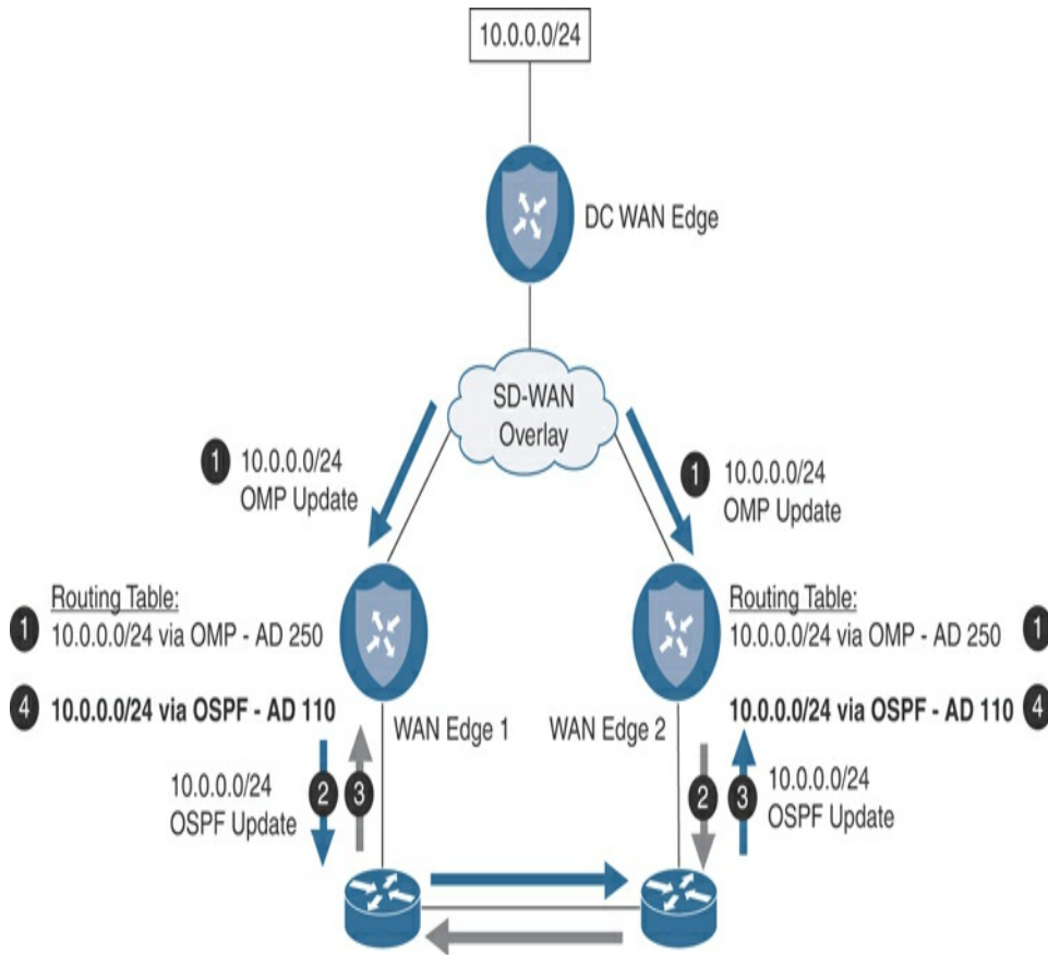
Figure 3-10 Routing Loop
