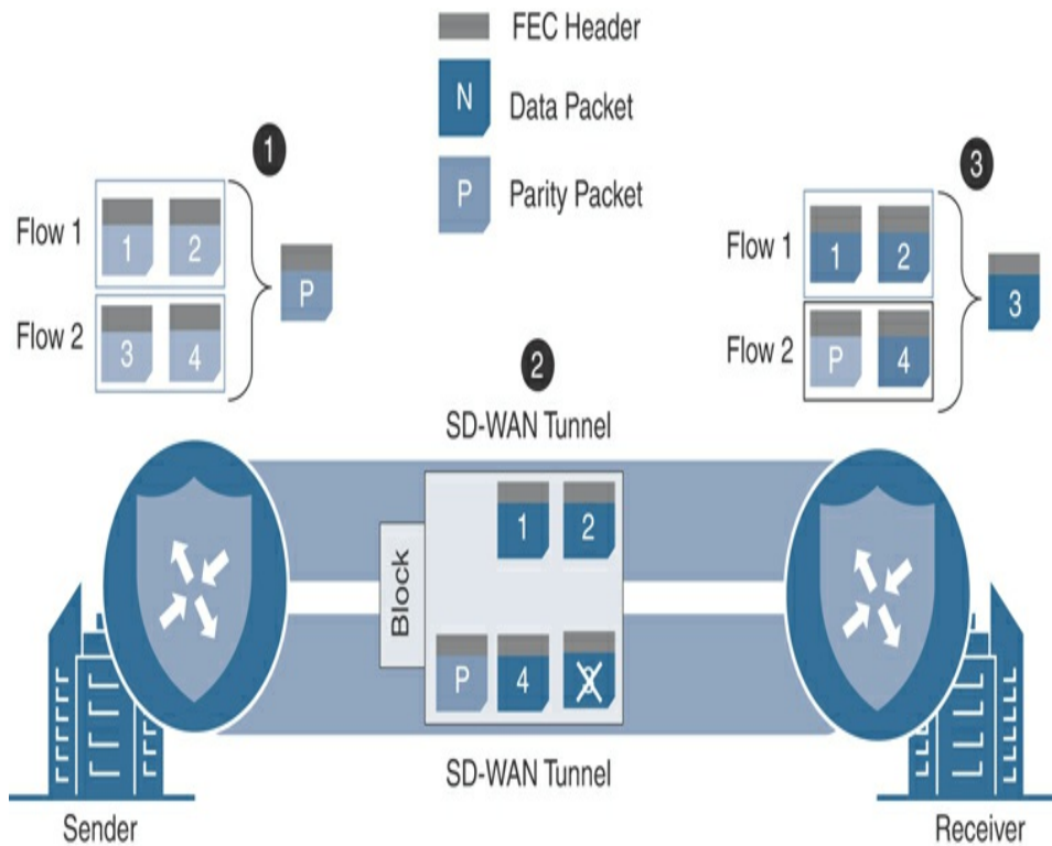
Figure 7-24 FEC Illustration
