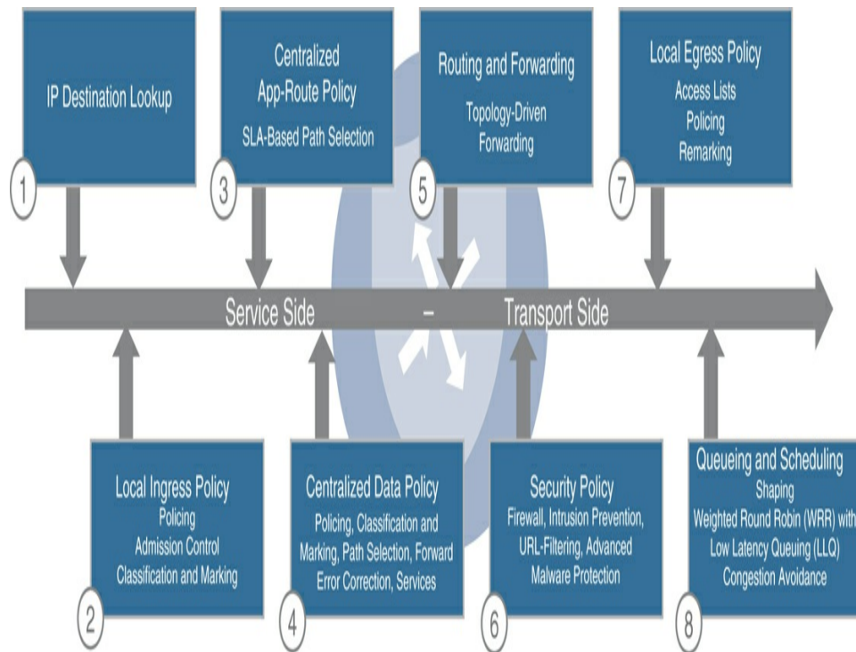
Figure 5-8 Packet Forwarding Order of Operations
