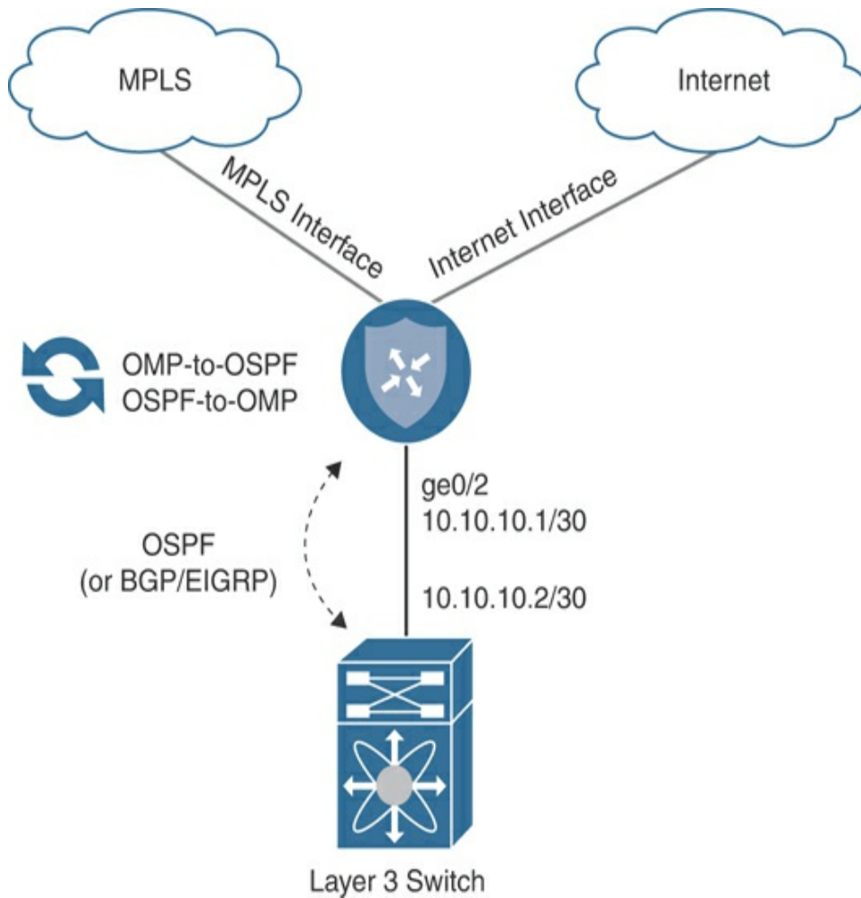
Figure 12-10 Complete CE Replacement—Dual Router L3 Branch
