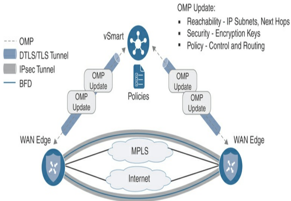
Figure 2-7 Cisco Control Plane and Data Plane Overview
