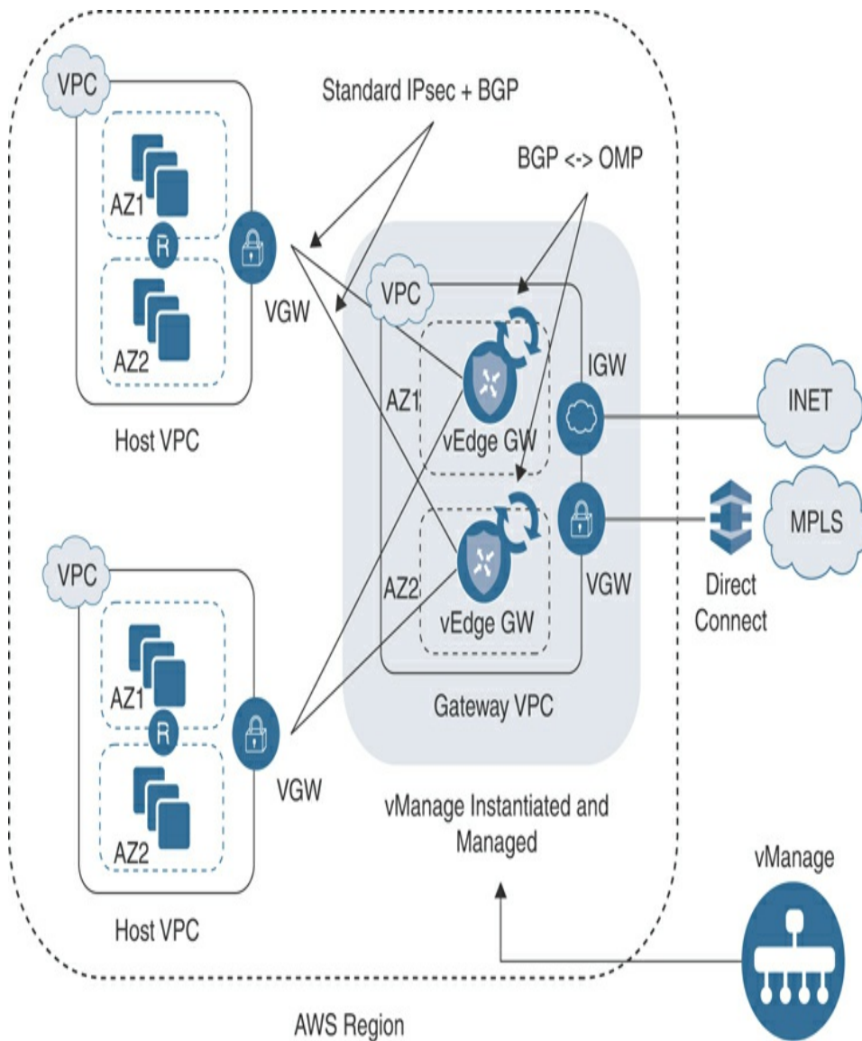
Figure 11-28 Cloud onRamp for IaaS Design
