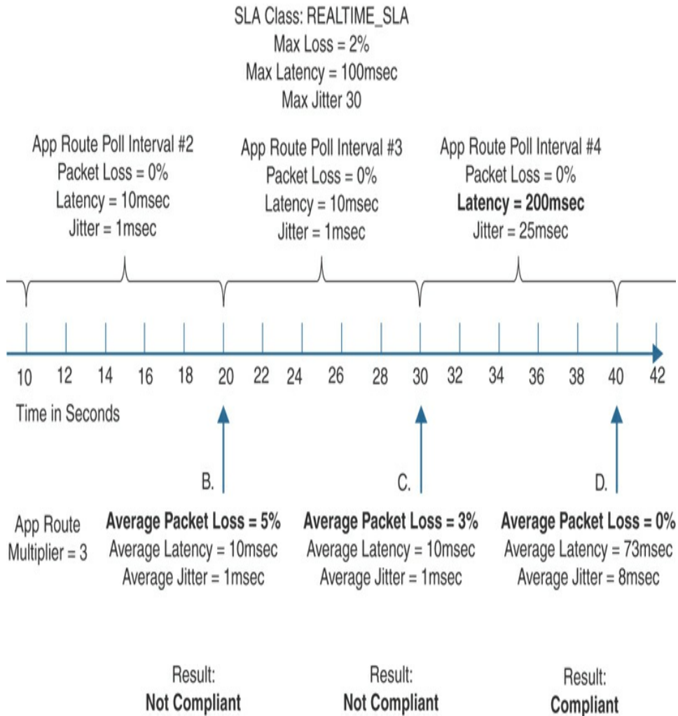
Figure 8-18 SLA Calculations with Multiple App-Route Poll Intervals
