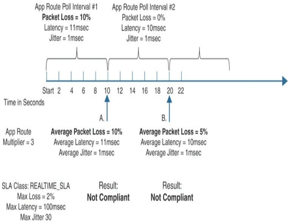
Figure 8-17 SLA Calculations with Two App-Route Poll Intervals
