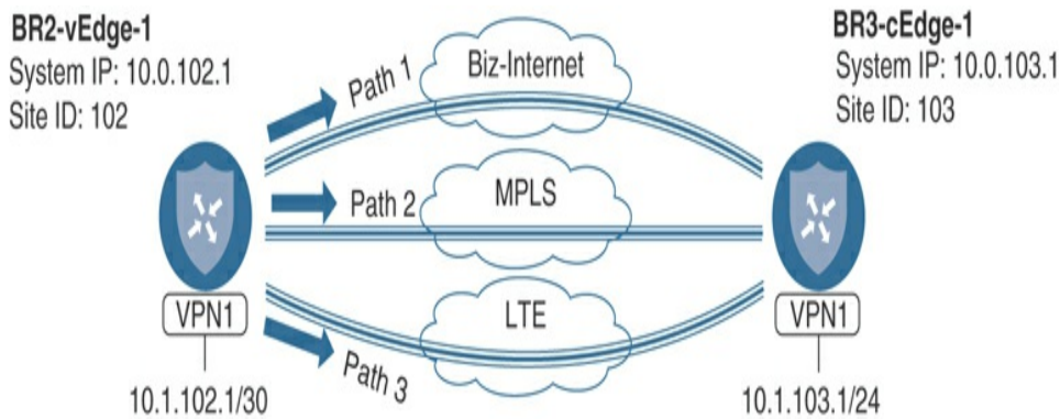
Figure 8-19 Application-Aware Routing Network Topology
