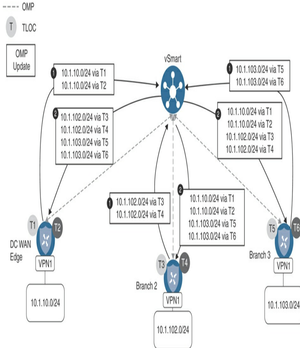
Figure 6-20 OMP Routes with Next-Hop TLOCs Reflected Through the vSmart
