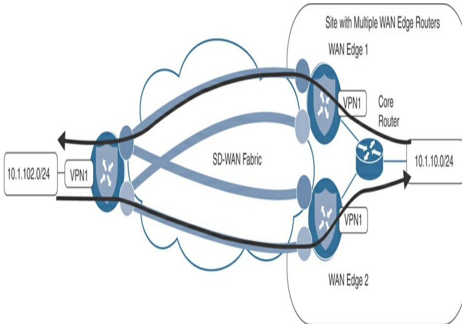
Figure 6-43 Multipathing on the Fabric May Use Multiple WAN Edge Routers for a Single Flow
