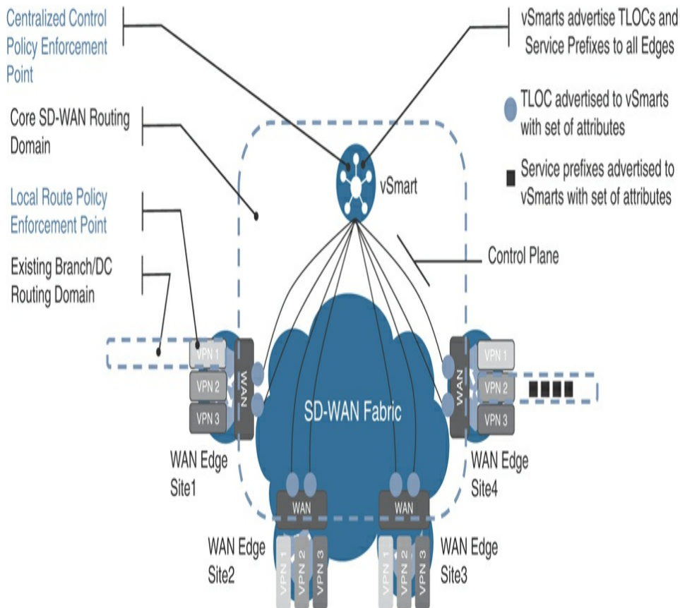
Figure 5-4 Manipulating the Control Plane with Centralized and Localized Control Policies
