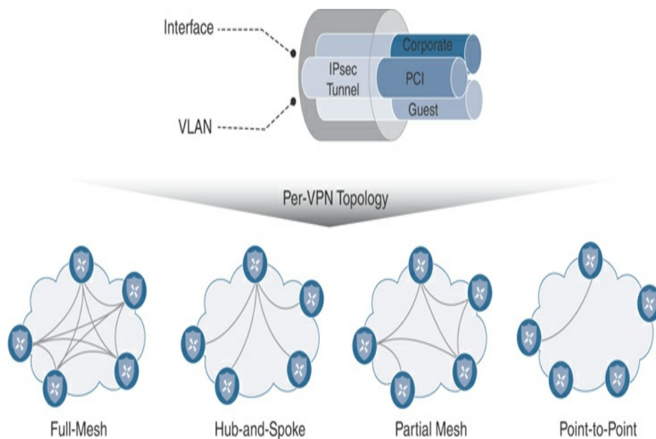
Figure 2-3 Segmentation and Per VPN Topologies
