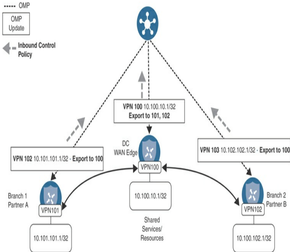
Figure 6-60 Building an Extranet to Enable Partner Connectivity
