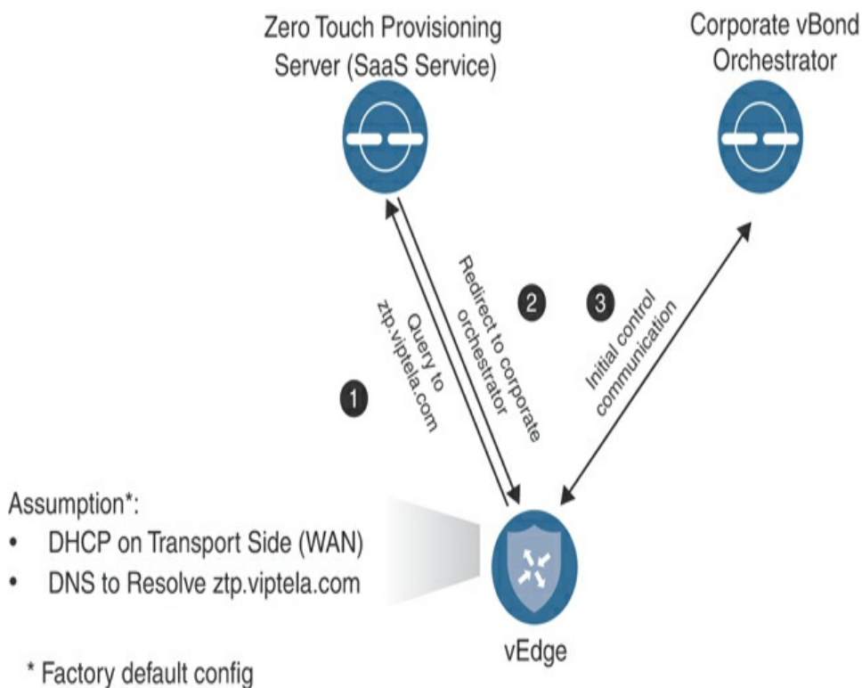
Figure 4-13 Zero Touch Provisioning Workflow
