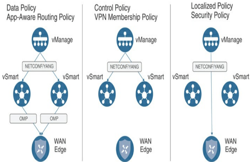
Figure 5-7 Policy Administration, Activation, and Enforcement
