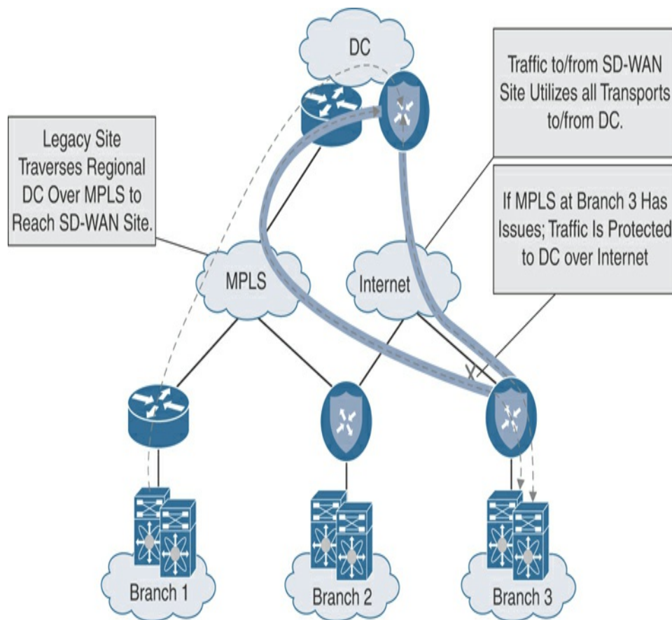
Figure 12-23 SD-WAN to Non-SD-WAN Site Overlay-Only Traffic Flow
