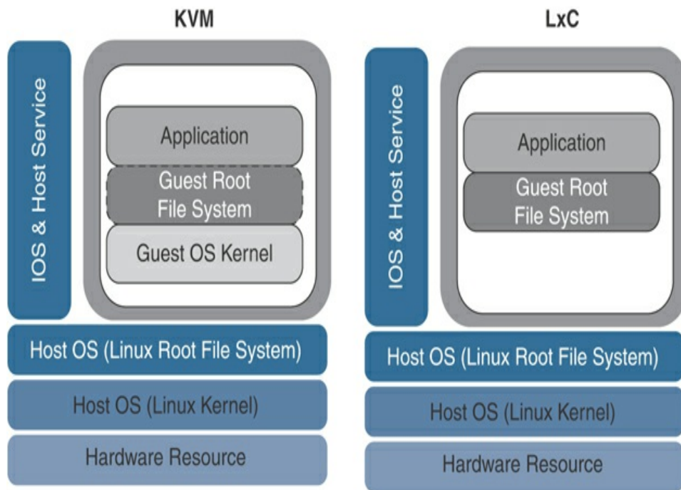
Figure 10-15 Application Service Container Architecture
