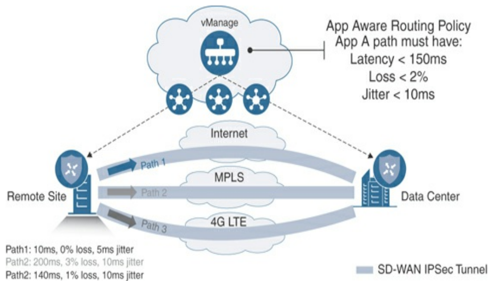
Figure 1-9 Routing Based on Application Performance
