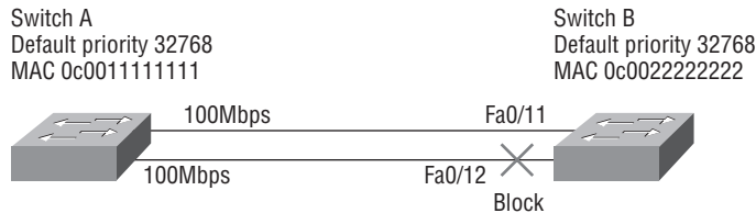
FIGURE 8.11 A switched network with redundant switched paths
