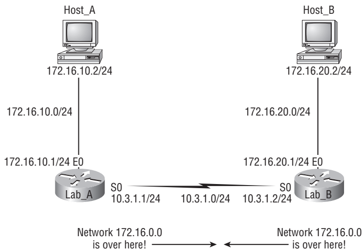
FIGURE 7.2 EIGRP auto-summarization
