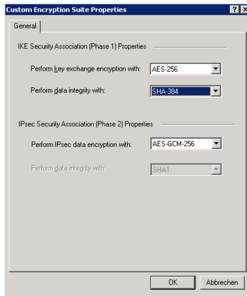
Figure 2.3.: Custom Encryption Suite Properties
